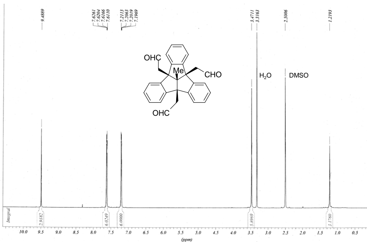
4b,8b,12b-Tris(formacymethyl)-12d-methyl-4b,8b,12b,12d-tetrahydro-dibenzo[2,3:4,5]pentaleno[1,6- ab ]indene (12d-methyltribenzotriquinacene 4b,8b,12b-tris-acetaldehyde, 15 ) (500 MHz, DMSO-d 6 )
