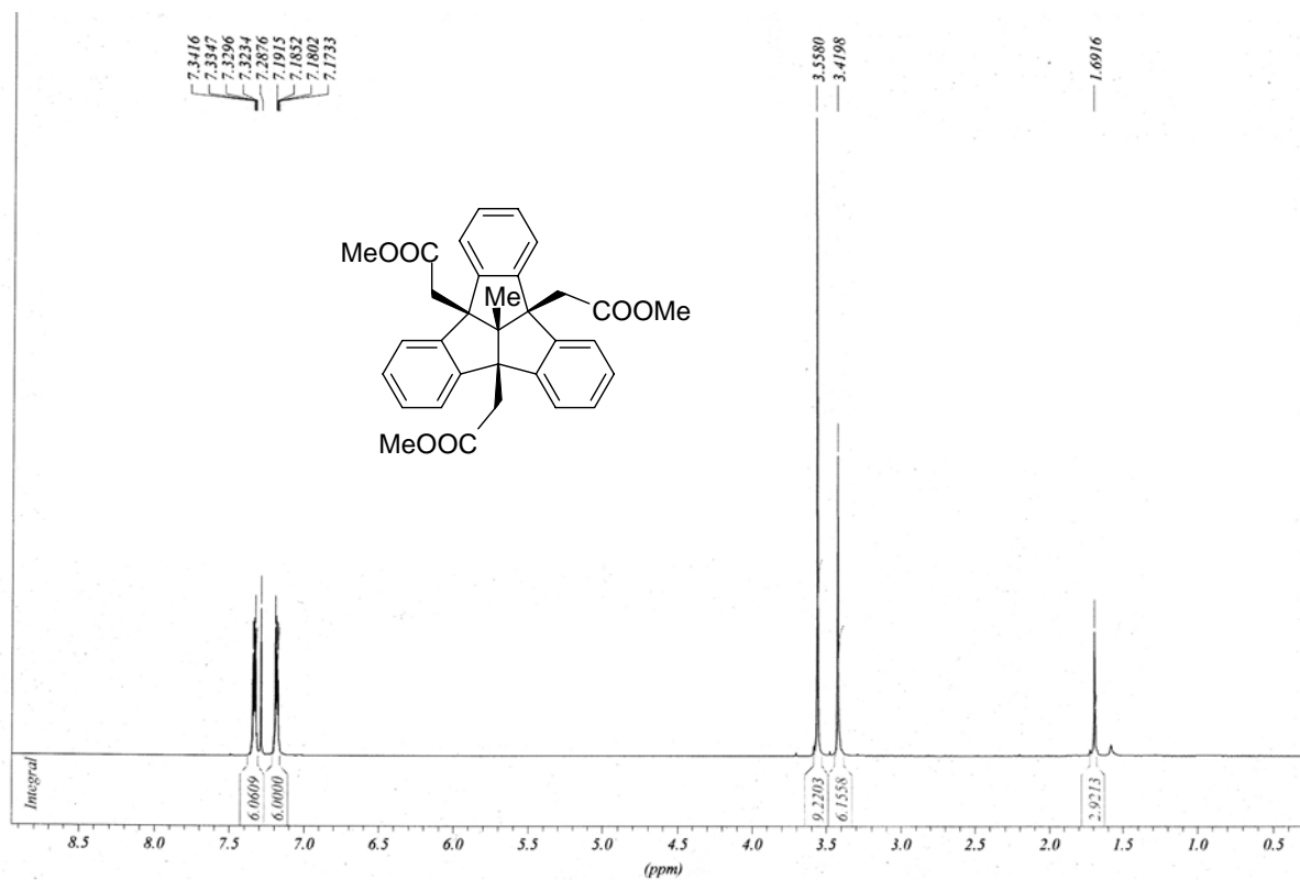
4b,8b,12b-Tris(methoxycarbonylmethyl)-12d-methyl-4b,8b,12b,12d-tetrahydro-dibenzo[2,3:4,5]pentaleno[1,6-ab]indene (trimethyl 12d-methyltribenzotriquinacene 4b,8b,12b-tris-acetate, 17 ) (500 MHz, CDCl 3 )
