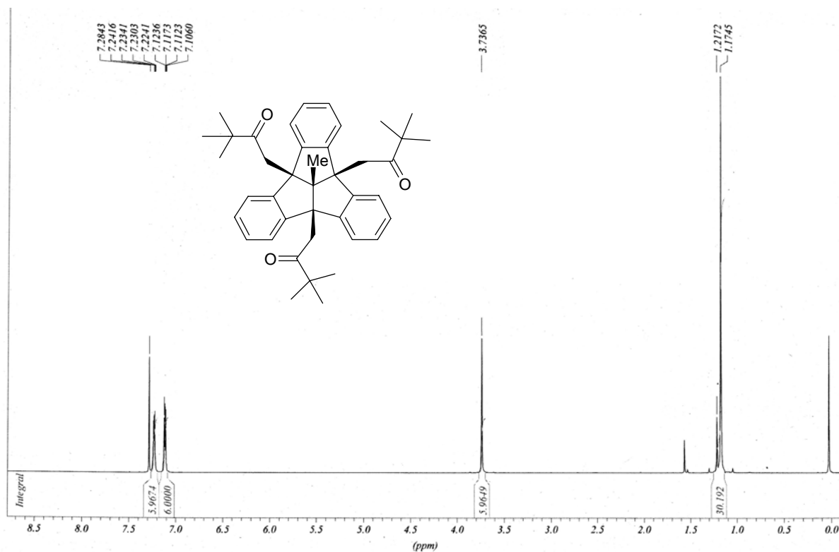
12d-Methyl-4b,8b,12b-tris(3,3-dimethyl-2-oxobutyl)-4b,8b,12b,12d-tetrahydrodibenzo[2,3:4,5]pentaleno[1,6-ab]indene ( 10 ) (500 MHz, CDCl 3 )
