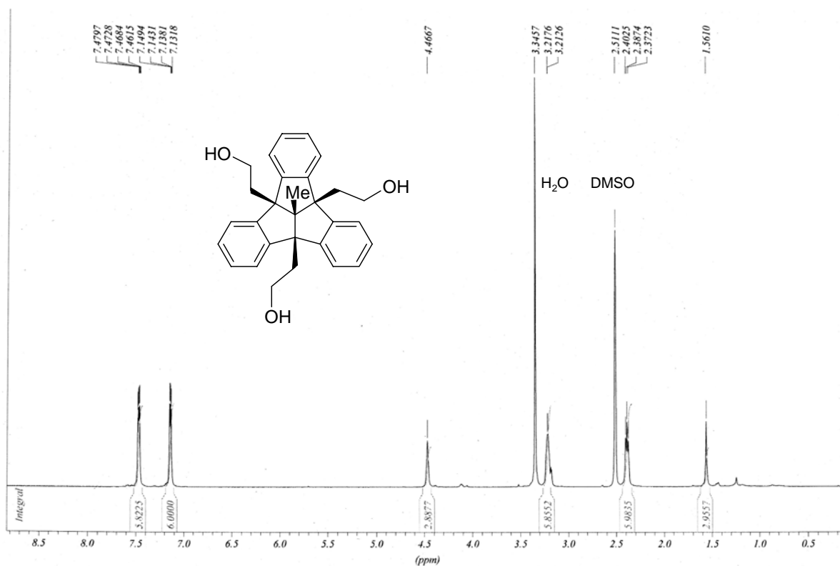
4b,8b,12b-Tris(2-hydroxyethyl)-12d-methyl-4b,8b,12b,12d-tetrahydro-dibenzo[2,3:4,5]pentaleno[1,6-ab]indene (12d-methyltribenzotriquinacene 4b,8b,12b-tris-ethanol, 18 ) (500 MHz, DMSO- d_6 )
