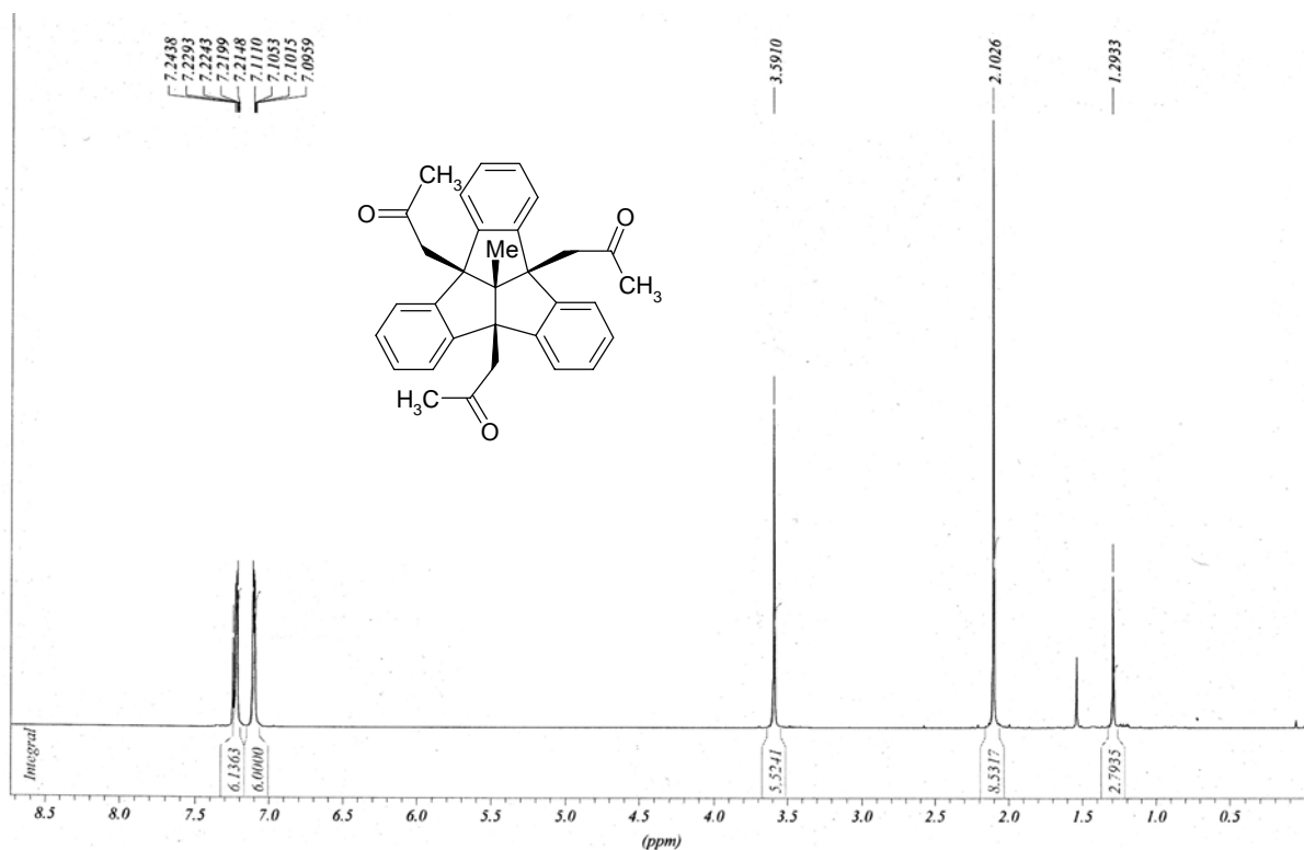
12d-Methyl-4b,8b,12b-tris(2-oxopropyl)-4b,8b,12b,12d-tetrahydrodibenzo[2,3:4,5]pentaleno[1,6- ab ]indene ( 7 ) (600 MHz, CDCl 3 )
