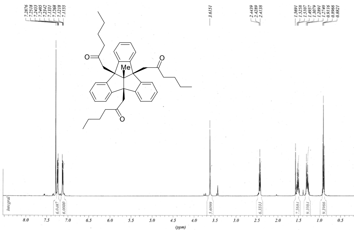
12d-Methyl-4b,8b,12b-tris(2-oxohexyl)-4b,8b,12b,12d-tetrahydrodibenzo[2,3:4,5]pentaleno[1,6- ab ]indene ( 8 ) (500 MHz, CDCl 3 )
