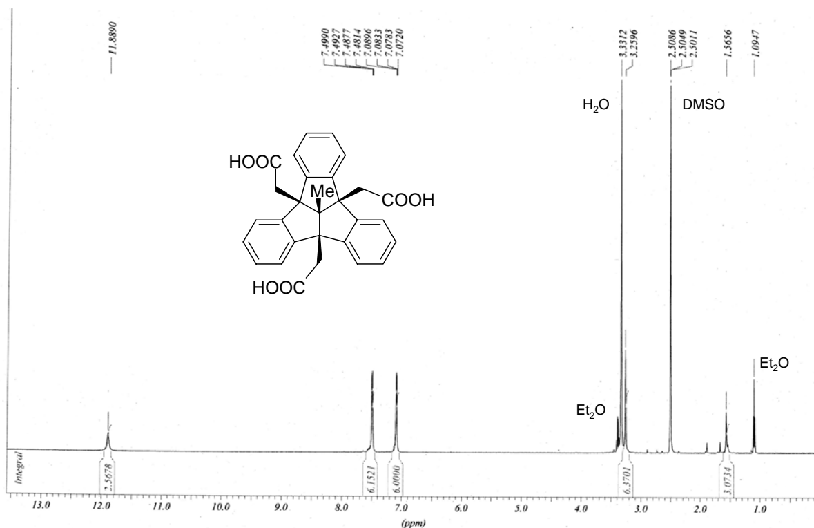
4b,8b,12b-Tris(carboxymethyl)-12d-methyl-4b,8b,12b,12d-tetrahydro-dibenzo[2,3:4,5]pentaleno[1,6-ab]indene [12d-methyltribenzotriquinacene 4b,8b,12b-tris(acetic acid), 16 ] (500 MHz, DMSO-d 6 )
