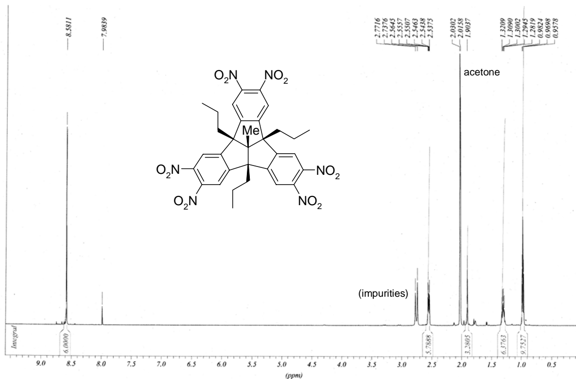
12d-Methyl-2,3,6,7,10,11-hexanitro-4b,8b,12b-tri( n -propyl)-4b,8b,12b,12d-tetrahydrodibenzo[2,3:4,5]pentaleno[1,6- ab ]indene [12d-methyl-2,3,6,7,10,11-hexanitrotribenzotriquinacene, 20 ] (500 MHz, acetone- d 6 )
