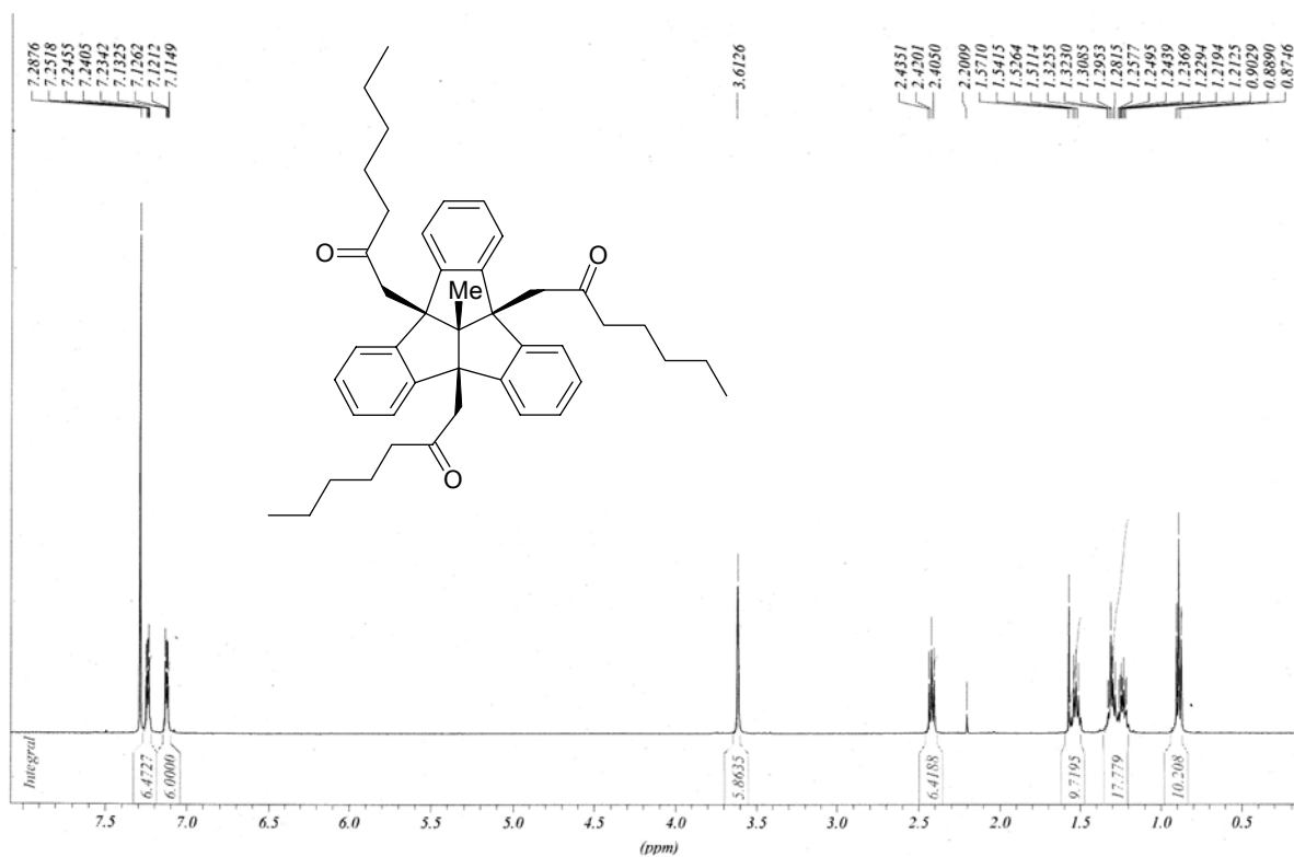
12d-Methyl-4b,8b,12b-tris(2-oxoheptyl)-4b,8b,12b,12d-tetrahydrodibenzo[2,3:4,5]pentaleno[1,6- ab ]indene ( 11 ) (500 MHz, CDCl 3 )
