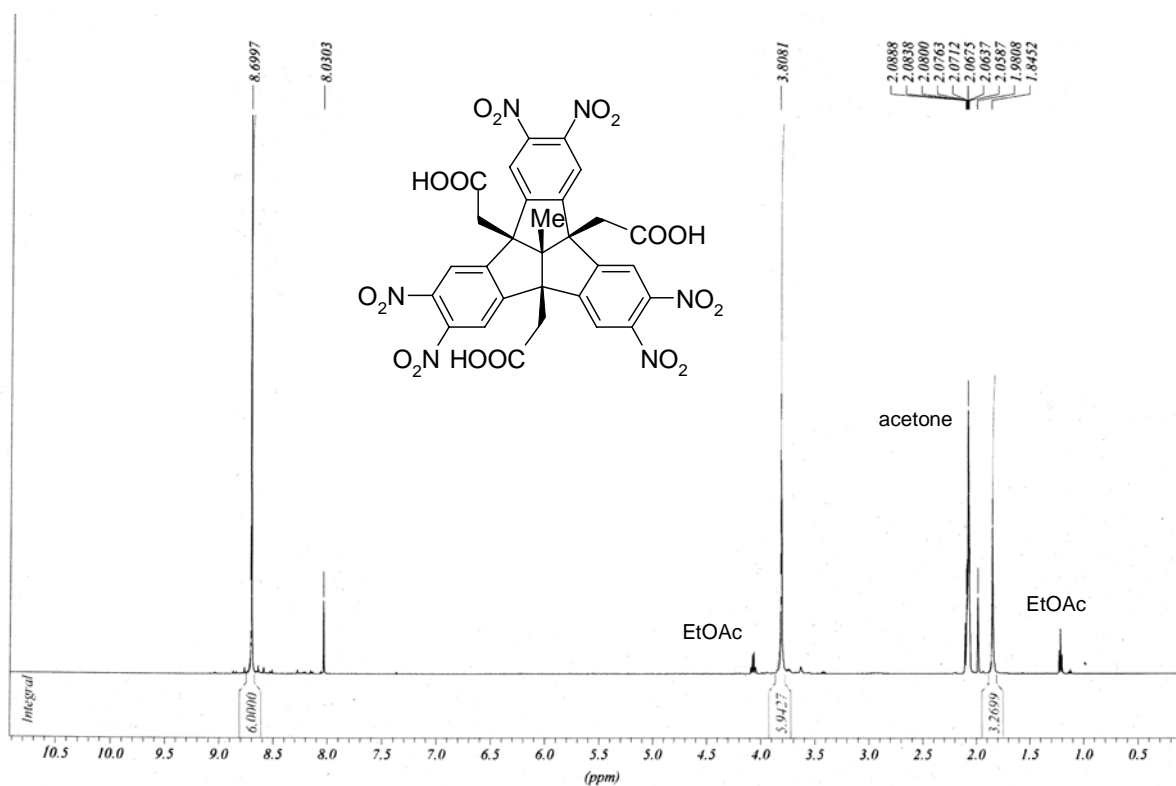
4b,8b,12b-Tris(carboxymethyl)-12d-methyl-2,3,6,7,10,11-hexanitro-4b,8b,12b,12d-tetrahydrodibenzo[2,3:4,5]pentaleno[1,6- ab ]indene [12d-methyl-2,3,6,7,10,11-hexanitrotribenzotriquinacene 4b,8b,12b-tris(acetic acid), 21 ] (500 MHz, acetone- d 6 )
