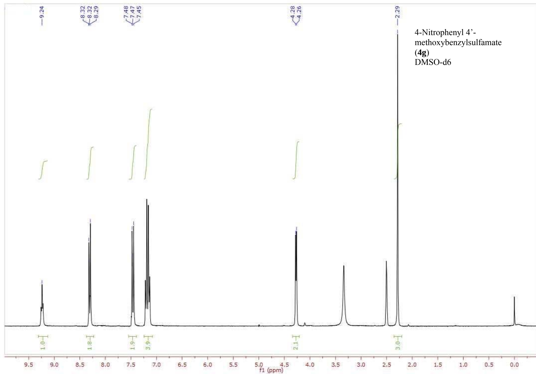
Fig. S2 1 H NMR spectra of 4-nitrophenyl benzylsulfamates (4a-g) in DMSO-d 6 (Varian Mercury 300MHz spectrometer)
