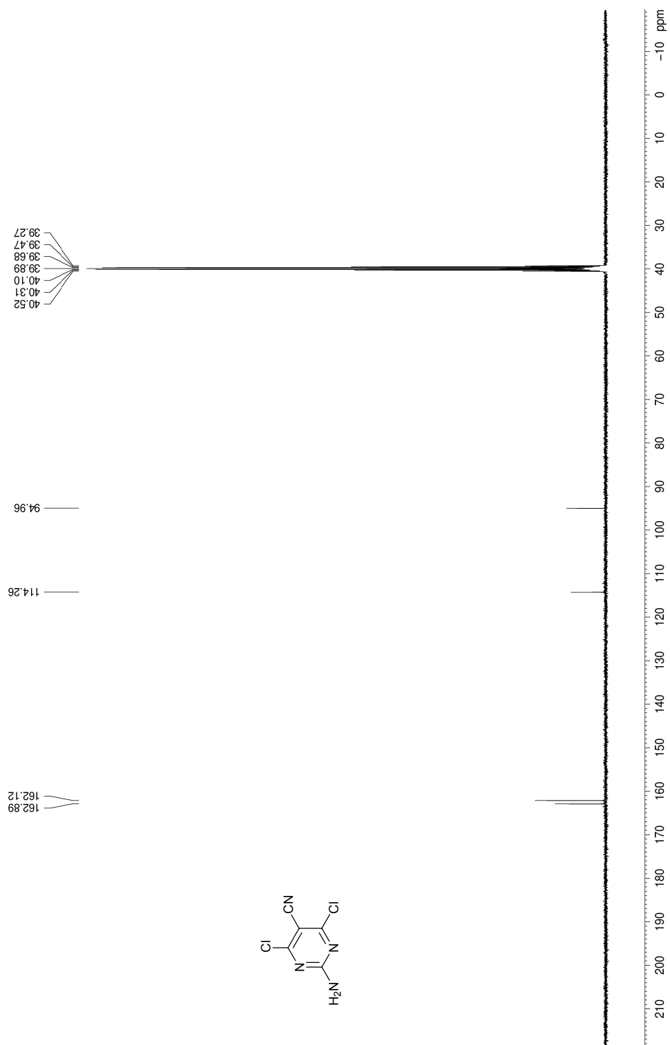
Figure S4: ^{13}\text{C} NMR spectrum of compound 4a
