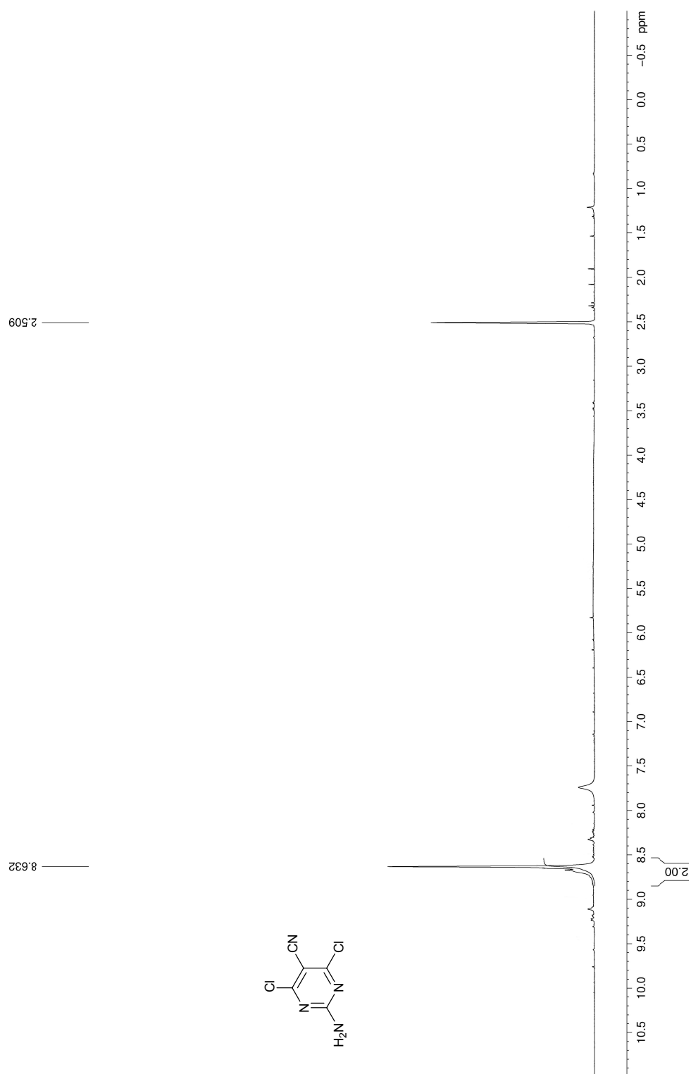
Figure S3: ^1\text{H} NMR spectrum of compound 4a
