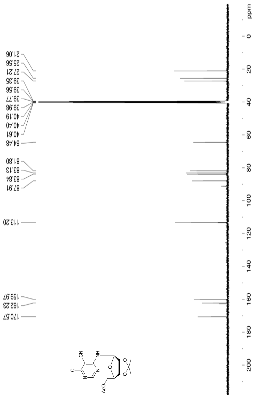
Figure S17: 13 C NMR spectrum of compound 7b
