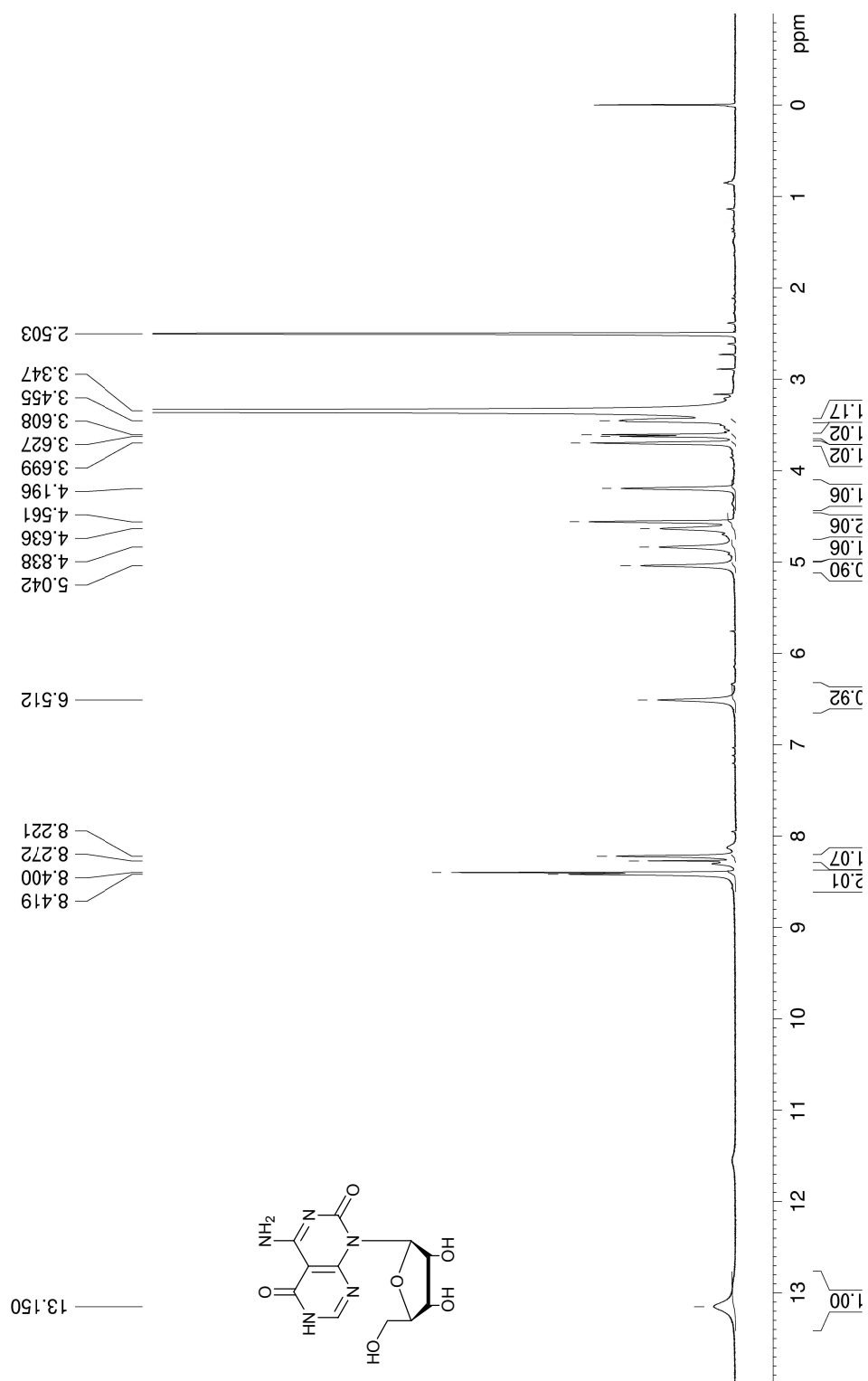
Figure S20: 1 H NMR spectrum of compound 1b
