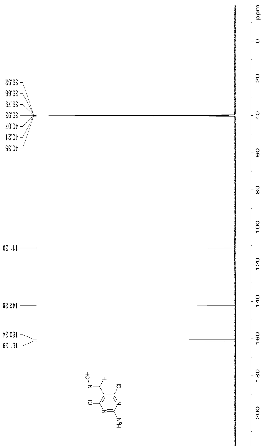
Figure S2: ^{13}\text{C} NMR spectrum of compound 3a
