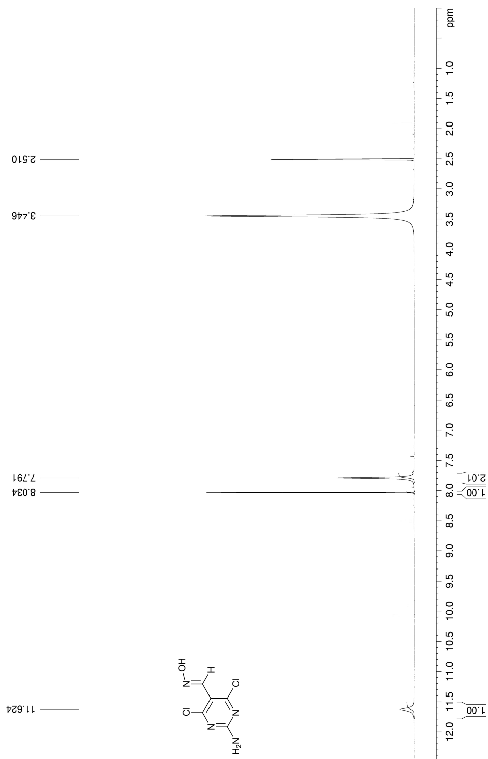
Figure S1: 1 H NMR spectrum of compound 3a
