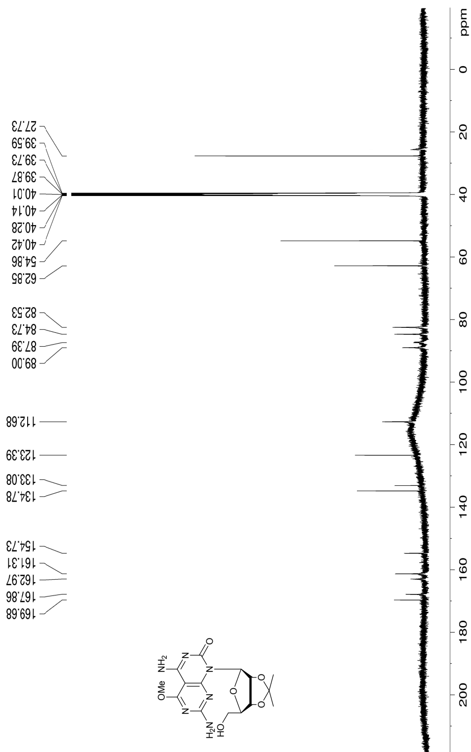
Figure S10: 13 C NMR spectrum of compound 8a
