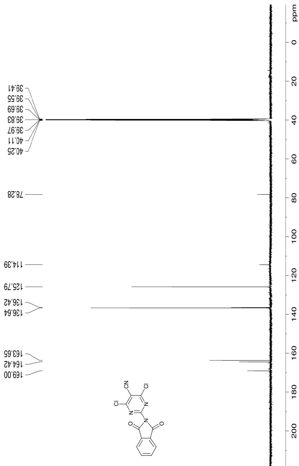
Figure S6: 13 C NMR spectrum of compound 5a
