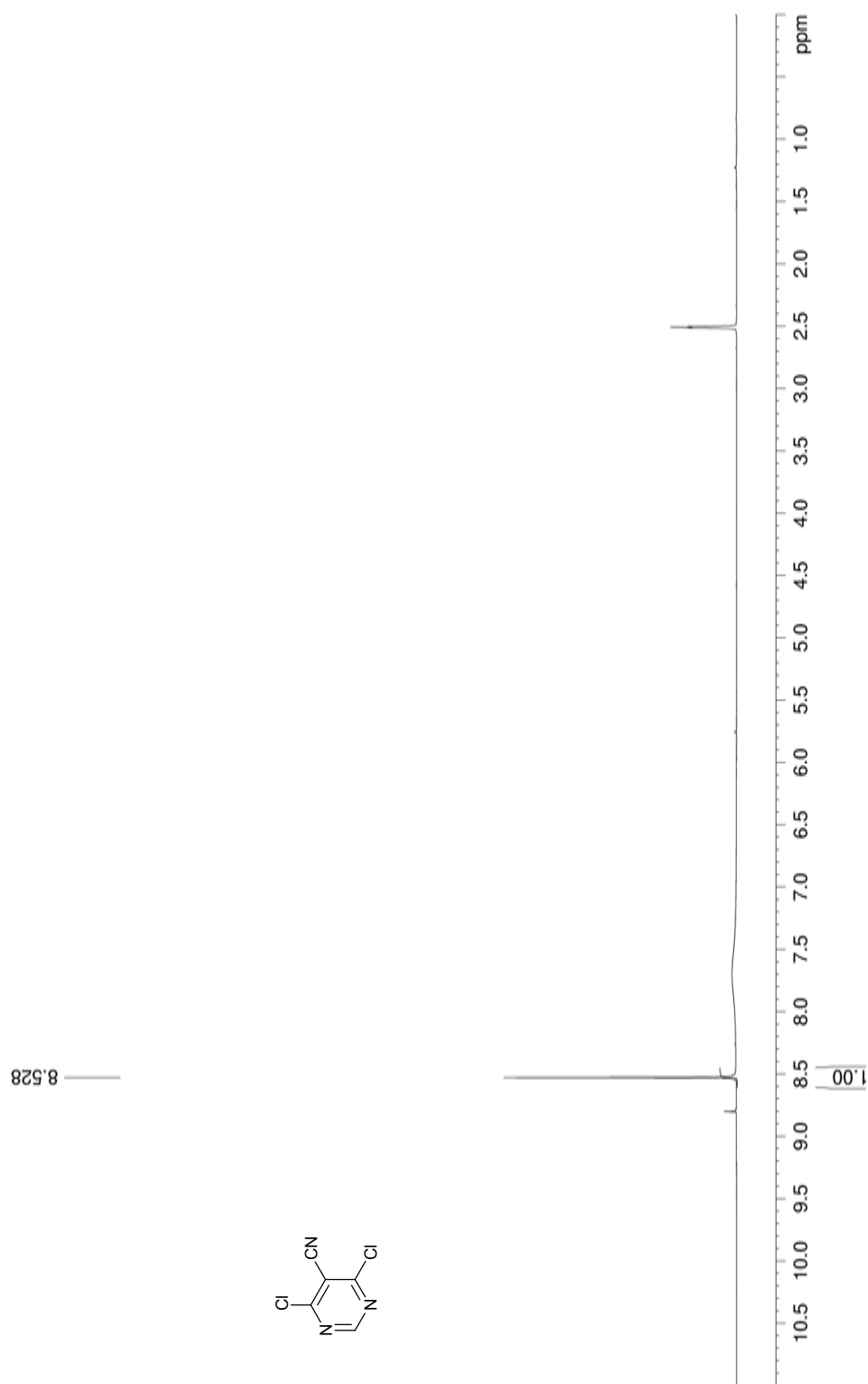
Figure S14: 1 H NMR spectrum of compound 4b
