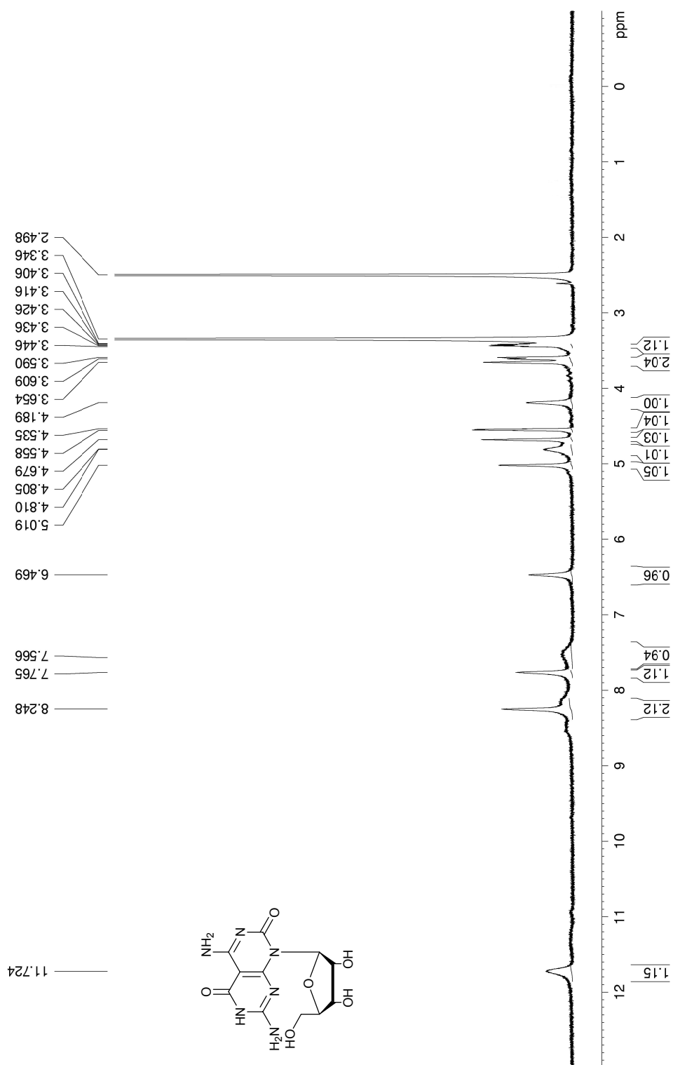
Figure S11: ^1\text{H} NMR spectrum of compound 1a
