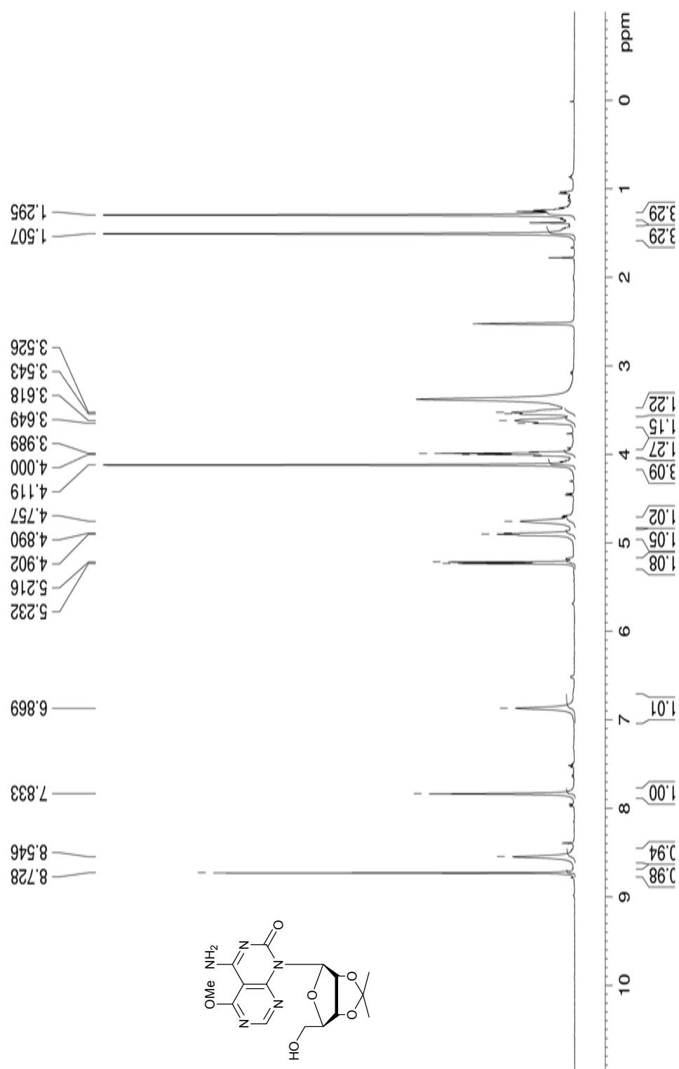
Figure S18: 1 H NMR spectrum of compound 8b
