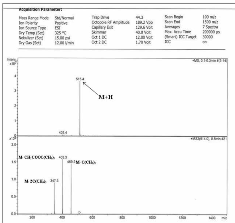
Figure S9. Mass spectrum of (4,7-bis- t -butoxycarbonylmethyl-1,4,7,10 tetraaza-cyclododec-1-yl)-acetic acid t -butyl ester, 4 [ESI + ]
