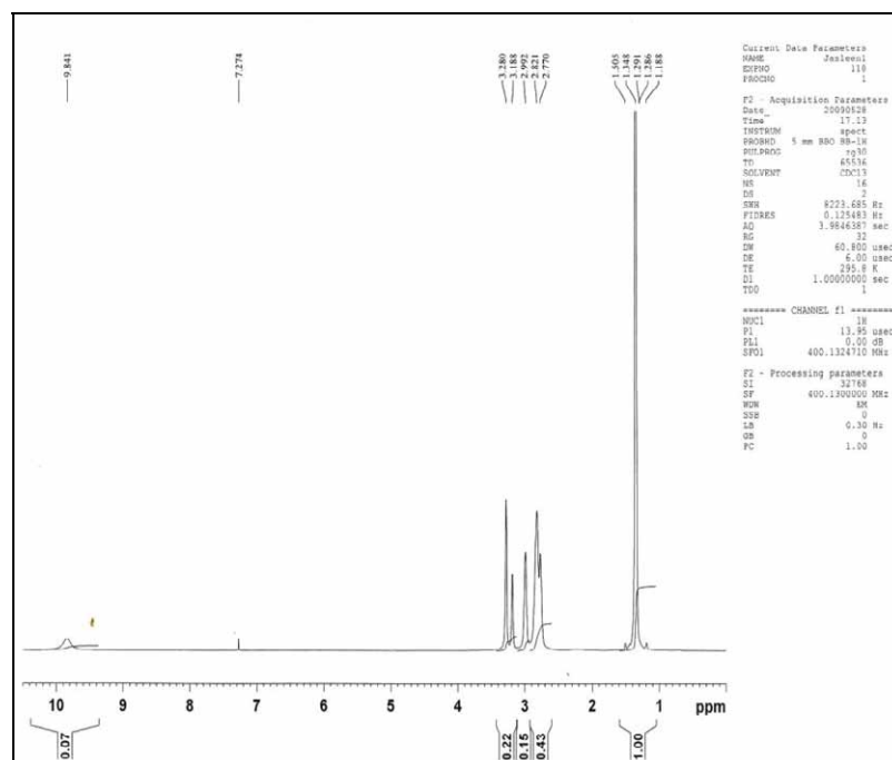
Figure S8. 13 C NMR spectrum of (4, 7-bis- t -butoxycarbonylmethyl-1,4,7,10 tetraaza-cyclododec-1-yl)-acetic acid t -butyl ester, 4 [400 MHz; CDCl 3 ]
