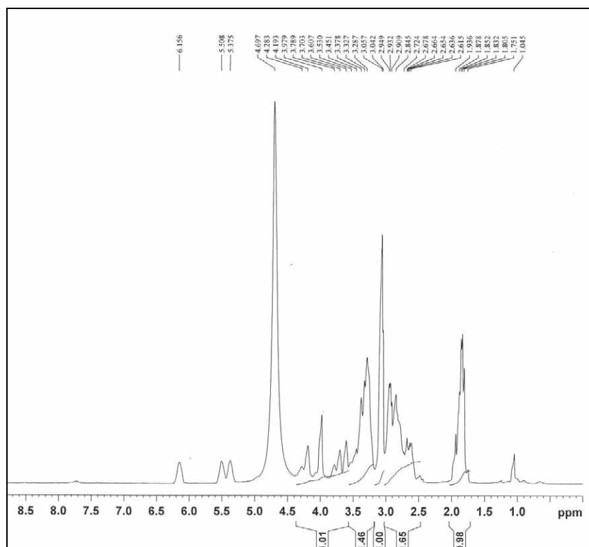
Figure S13. 1 H NMR spectrum of (2-hydroxy-ethyl)-dimethyl-[2-(4,7,10-tris-carboxymethyl-1,4,7,10-tetraaza-cyclododec-1-yl)-ethyl]-ammonium, 6 [400 MHz; D 2 O]
