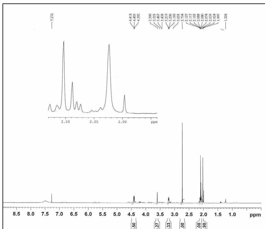
Figure S4. 1 H NMR spectrum of (2-acetoxy-ethyl)-(2-bromo-ethyl)-dimethyl-ammonium, 3 [400 MHz; CDCl 3 ]
