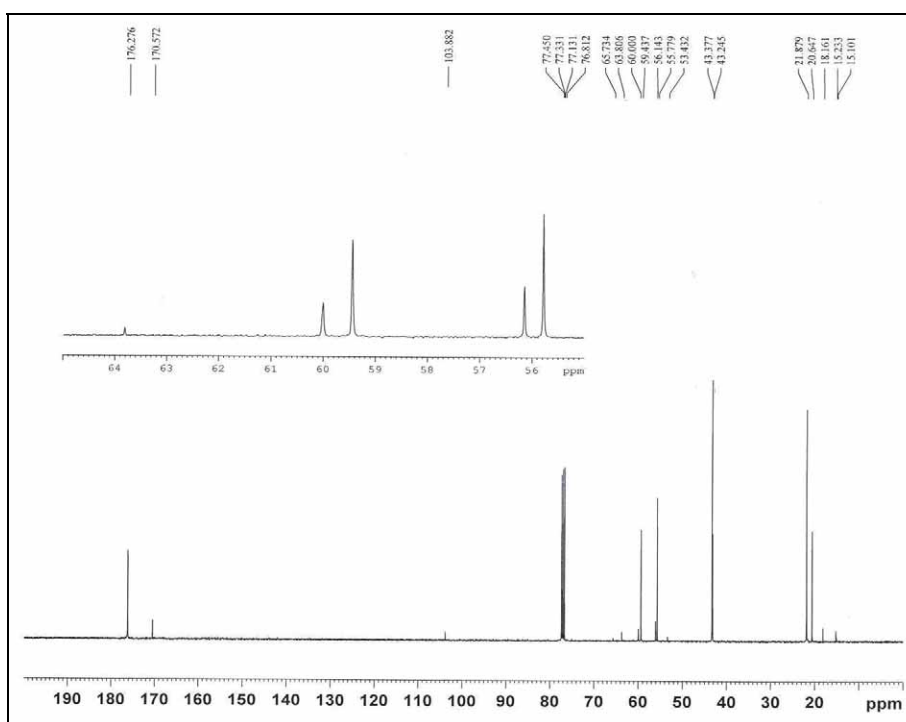
Figure S2. ^{13}\text{C} NMR spectrum of N,N -dimethylaminoethylacetate, 2 [400 MHz; \text{CDCl}_3 ]
