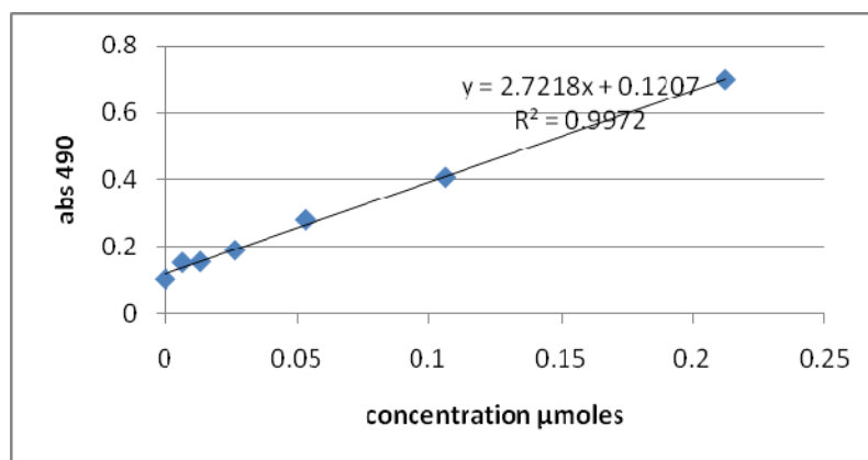
A calibration curve of sugar ( \beta -lactose) concentration versus absorbance (A)
