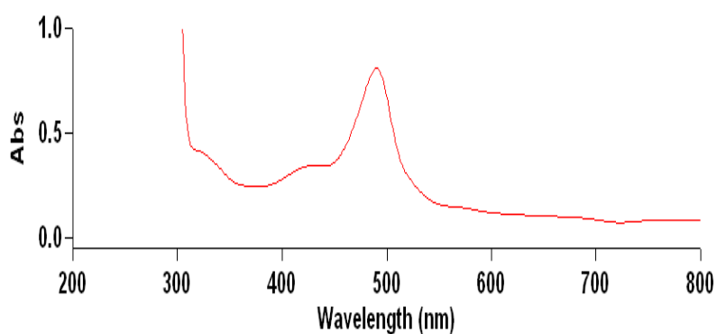
UV Absorbance spectrum of sugar-phenol conjugate
