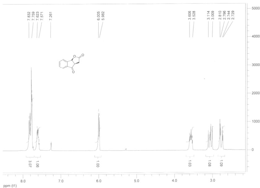
(3aR*,8bR*)-3,3a-Dihydro-2H-indeno[1,2-b]furan-2,4(8bH)-dione (8)
