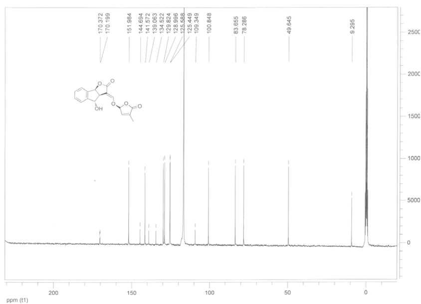
(3a S *,4 R *,8b S *, E )-4-hydroxy-3-(((( S *)-4-methyl-5-oxo-2,5-dihydrofuran-2-yl)oxy)methyl ene)-3,3a,4,8b-tetrahydro-2 H -indeno[1,2- b ]furan-2-one (11aβ)
