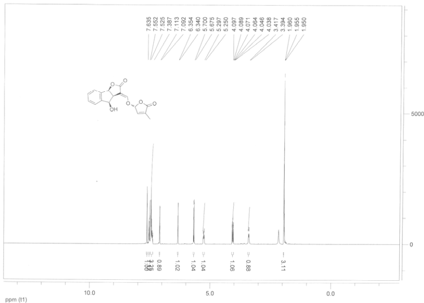
(3a S *,4 S *,8b S *, E )-4-hydroxy-3-(((( R *)-4-methyl-5-oxo-2,5-dihydrofuran-2-yl)oxy)methyl ene)-3,3a,4,8b-tetrahydro-2 H -indeno[1,2- b ]furan-2-one ( 16ba )
