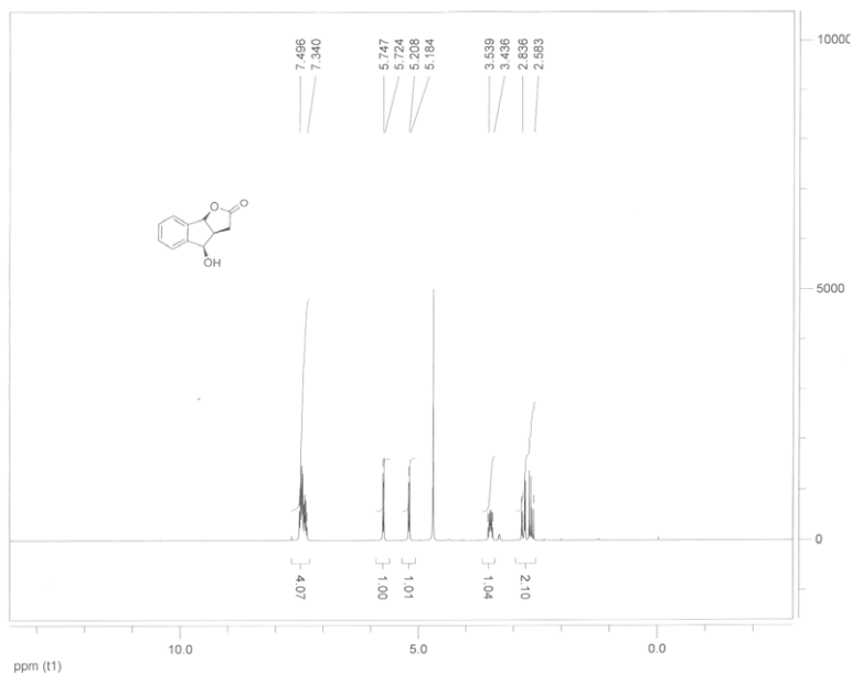
(3a S *,4 R *,8 bR *)-4-hydroxy-3,3a,4,8b-tetrahydro-2 H -indeno[1,2- b ]furan-2-one ( 9a )
