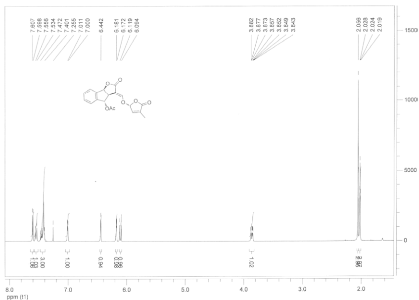
(3a S *,4 S *,8b S *, E )-3-(((( R *)-4-methyl-5-oxo-2,5-dihydrofuran-2-yl)oxy)methylene)-2-oxo-3,3a,4,8b-tetrahydro-2 H -indeno[1,2- b ]furan-4-yl acetate ( 12aa )
