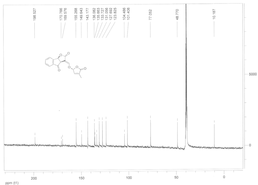
(3a R *,8b S *, E )-3-(((( R *)-4-methyl-5-oxo-2,5-dihydrofuran-2-yl)oxy)methylene)-3,3a-dihydro-2 H -indeno[1,2- b ]furan-2,4(8b H )-dione ( 18a )
