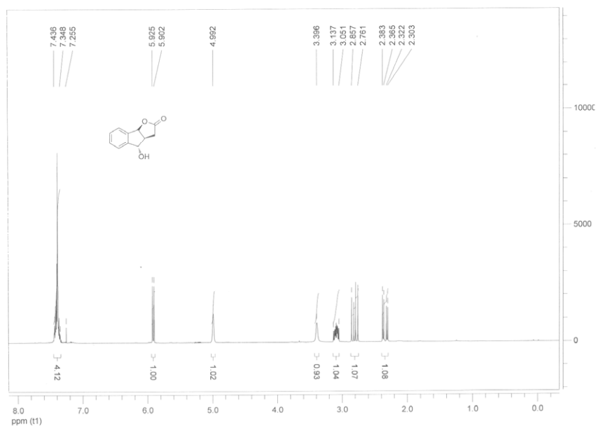
(3a S *,4 S *,8b R *)-4-hydroxy-3,3a,4,8b-tetrahydro-2 H -indeno[1,2- b ]furan-2-one ( 9b )
