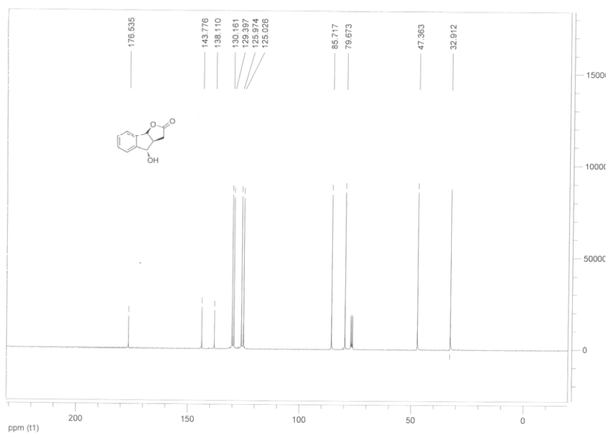
(3a S *,4 R *,8 bR *)-4-hydroxy-3,3a,4,8b-tetrahydro-2 H -indeno[1,2- b ]furan-2-one ( 9a )
