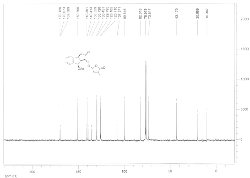
(3a S *,4 S *,8b S *, E )-3-(((( R *)-4-methyl-5-oxo-2,5-dihydrofuran-2-yl)oxy)methylene)-2-oxo-3,3a,4,8b-tetrahydro-2 H -indeno[1,2- b ]furan-4-yl acetate (17ba)
