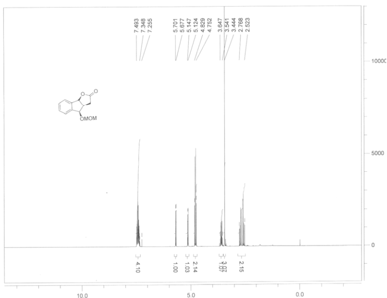
(3a S *,4 R *,8b S *)-4-(methoxymethoxy)-3,3a,4,8b-tetrahydro-2 H -indeno[1,2- b ]furan-2-one ( 13b )
