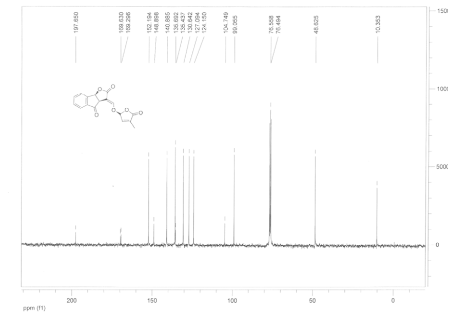
(3aR*,8bS*,E)-3-((((R*)-4-methyl-5-oxo-2,5-dihydrofuran-2-yl)oxy)methylene)-3,3a-dihydro-2H-indeno[1,2- b ]furan-2,4(8bH)-dione ( 18β )
