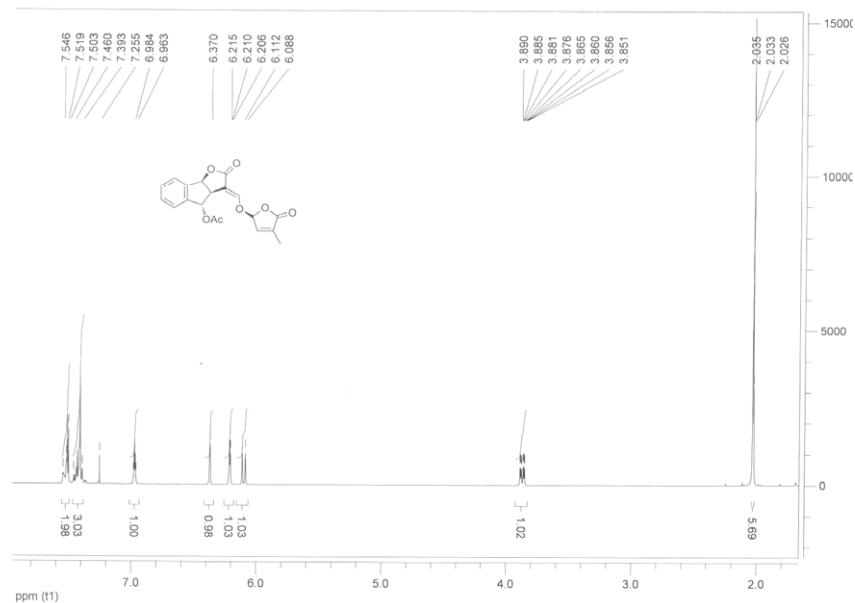
(3a S *,4 R *,8b S *, E )-3-(((( R *)-4-methyl-5-oxo-2,5-dihydrofuran-2-yl)oxy)methylene)-2-oxo-3,3a,4,8b-tetrahydro-2 H -indeno[1,2- b ]furan-4-yl acetate ( 12aβ )
