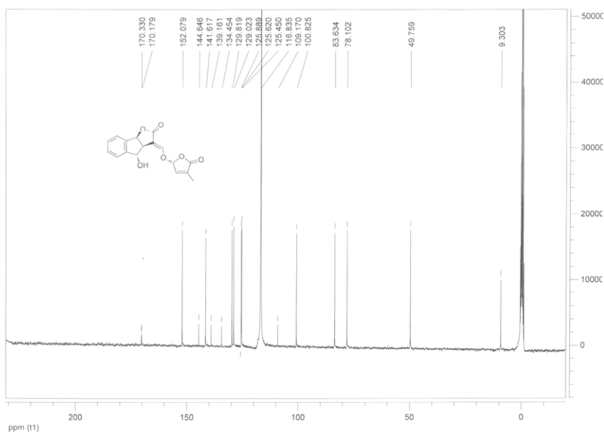
(3a S *,4 R *,8b S *, E )-4-hydroxy-3-(((( R *)-4-methyl-5-oxo-2,5-dihydrofuran-2-yl)oxy)methylene)-3,3a,4,8b-tetrahydro-2 H -indeno[1,2- b ]furan-2-one ( 11aa )
