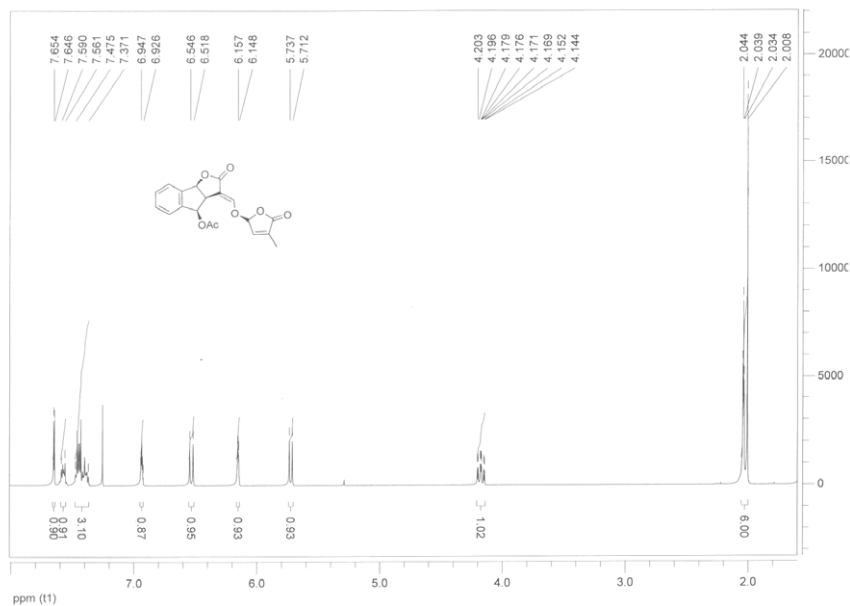
(3a S *,4 R *,8b S *, E )-3-(((( S *)-4-methyl-5-oxo-2,5-dihydrofuran-2-yl)oxy)methylene)-2-oxo-3,3a,4,8b-tetrahydro-2 H -indeno[1,2- b ]furan-4-yl acetate ( 17bβ )
