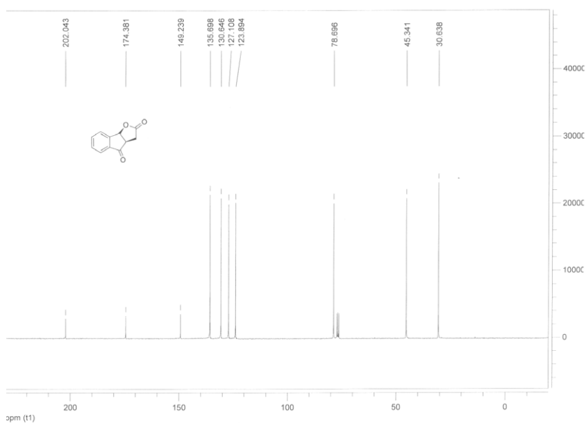
(3aR*,8bR*)-3,3a-Dihydro-2H-indeno[1,2-b]furan-2,4(8bH)-dione (8)
