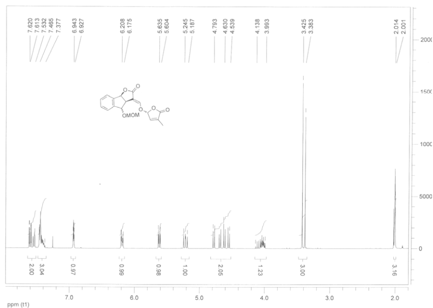
(3a S *,4 R *,8b S *, E )-4-(methoxymethoxy)-3-((( R *, S *)-4-methyl-5-oxo-2,5-dihydrofuran-2-yl)oxy)methylene)-3,3a,4,8b-tetrahydro-2 H -indeno[1,2- b ]furan-2-one ( 14b )
