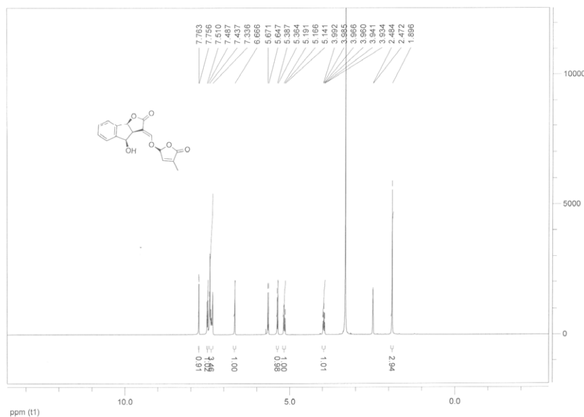
(3a S *,4 S *,8b S *, E )-4-hydroxy-3-(((( S *)-4-methyl-5-oxo-2,5-dihydrofuran-2-yl)oxy)methylene)-3,3a,4,8b-tetrahydro-2 H -indeno[1,2- b ]furan-2-one ( 16bβ )
