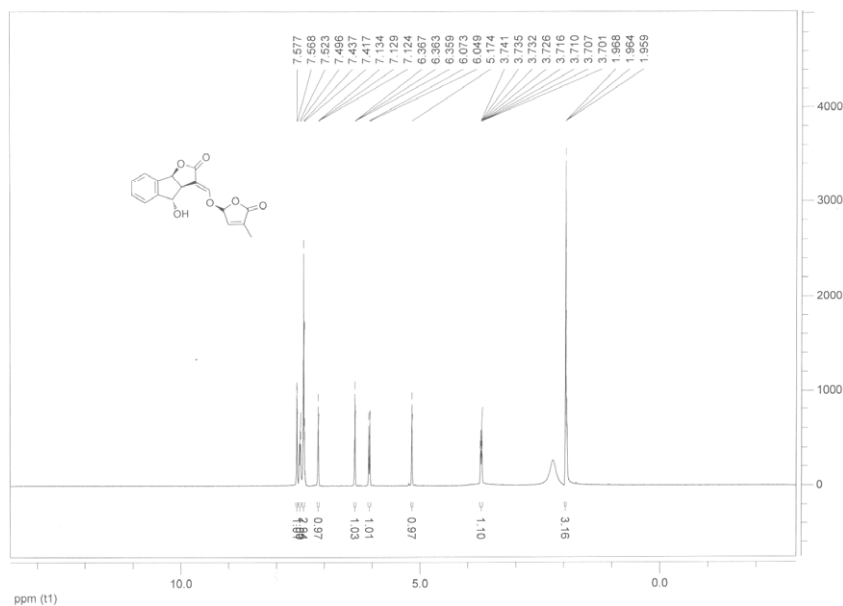
(3a S *,4 R *,8b S *, E )-4-hydroxy-3-(((( S *)-4-methyl-5-oxo-2,5-dihydrofuran-2-yl)oxy)methyl ene)-3,3a,4,8b-tetrahydro-2 H -indeno[1,2- b ]furan-2-one (11aβ)
