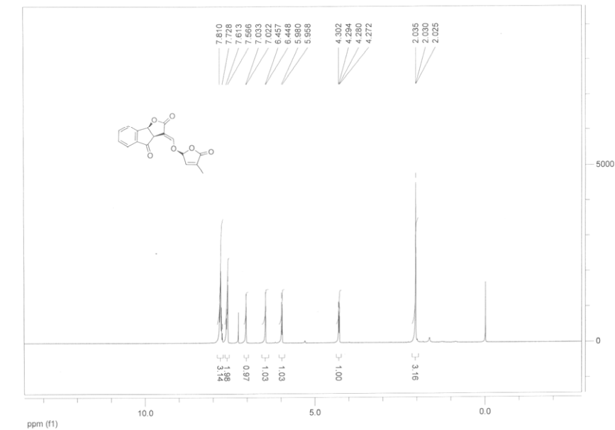
(3aR*,8bS*,E)-3-((((R*)-4-methyl-5-oxo-2,5-dihydrofuran-2-yl)oxy)methylene)-3,3a-dihydro-2H-indeno[1,2-b]furan-2,4(8bH)-dione ( 18β )
