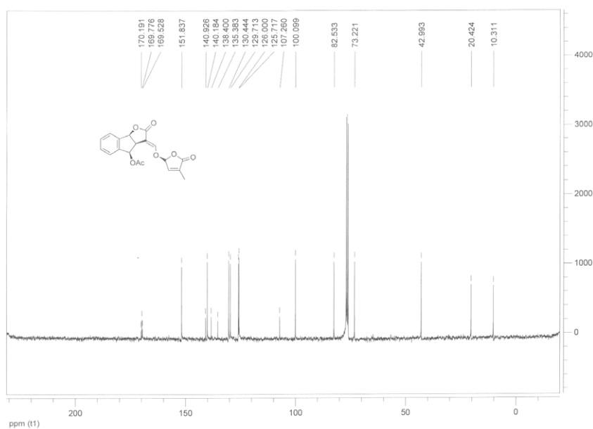
(3a S *,4 R *,8b S *, E )-3-(((( S *)-4-methyl-5-oxo-2,5-dihydrofuran-2-yl)oxy)methylene)-2-oxo-3,3a,4,8b-tetrahydro-2 H -indeno[1,2- b ]furan-4-yl acetate ( 17bβ )
