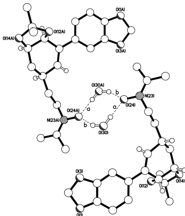
Fig. S3 The molecular structure of 16 showing the C_i -symmetric dimer formed by hydrogen bonding to the included water molecule. The O–H \cdots O hydrogen bonds have [O \cdots O], [H \cdots O] distances (Å) and [O–H \cdots O] angles (°) of a ) 2.794(2), 1.90, 175, and b ) 2.811(2), 1.98, 153.
