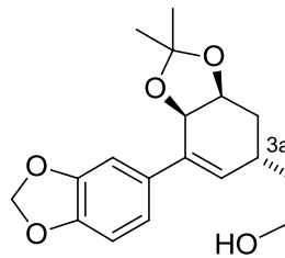
epi-11 (trianthine series)
