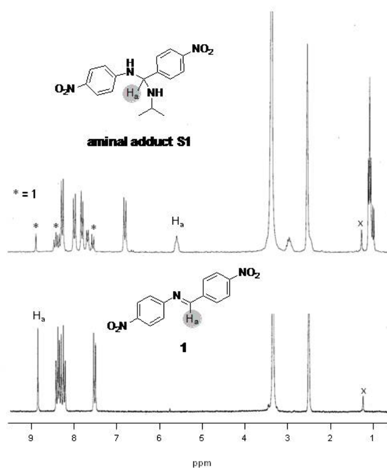
Fig. S1 Transimination reaction of imines 1 (15 mM) with isopropylamine (15 mM) in DMSO- d 6 at ambient temperature.
