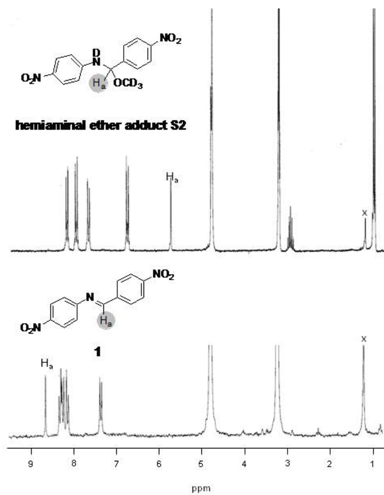
Fig. S2 Transimination reaction of imines 1 (15 mM) with isopropylamine (15 mM) in methanol- d 4 at ambient temperature.
