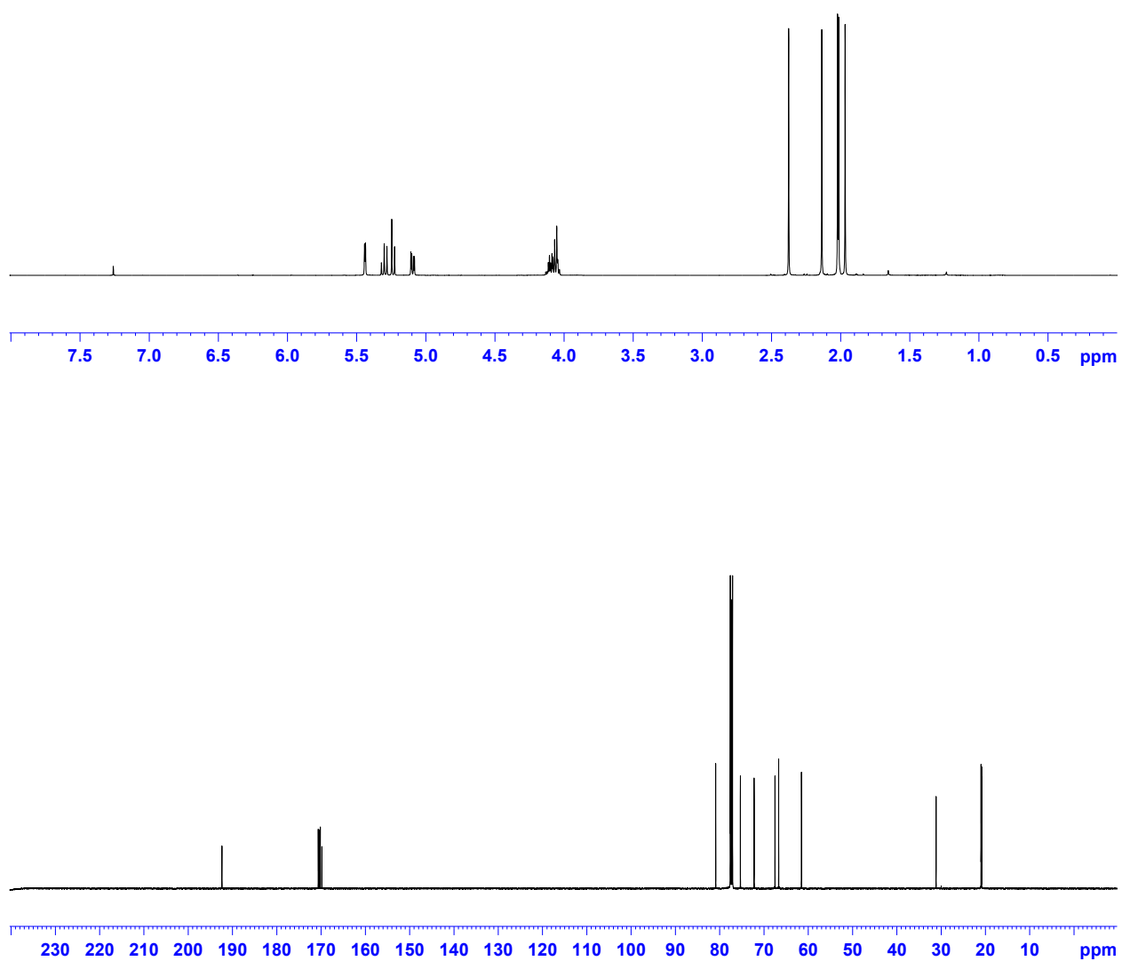
Figure SX. ^1\text{H-NMR} (top) and ^{13}\text{C-NMR} (bottom) spectra of compound 2 .
