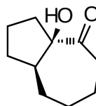
Compound 42
