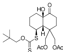
Compound 24
