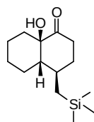
Compound 28
