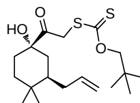
Compound 47b
