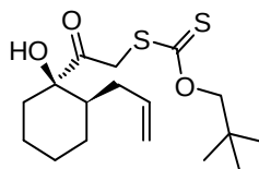
Compound 32
