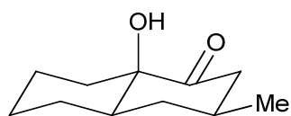
Compound 37e
