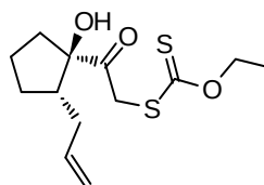
Compound 40b
