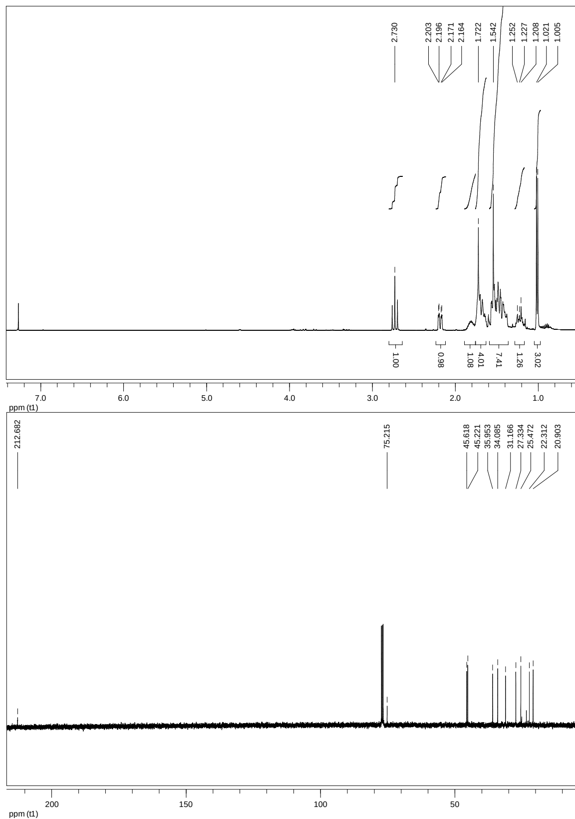
Compound 37e
