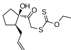
Compound 40a
