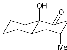
Compound 37a
