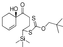
Compound 25
