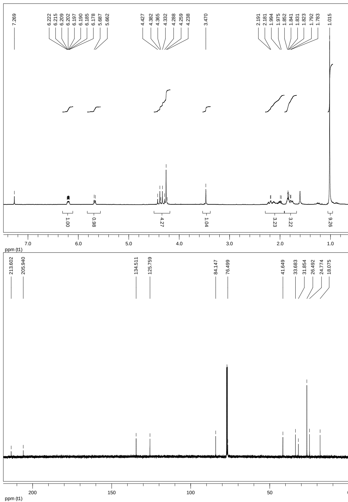
Compound 15
