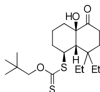
Compound 22
