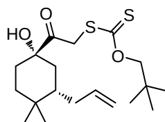
Compound 47a
