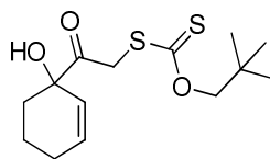
Compound 15
