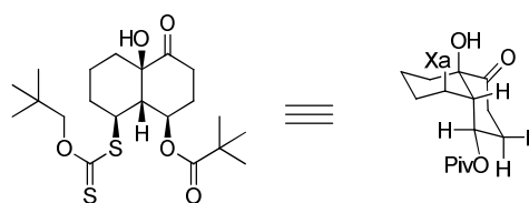
Compound 20
