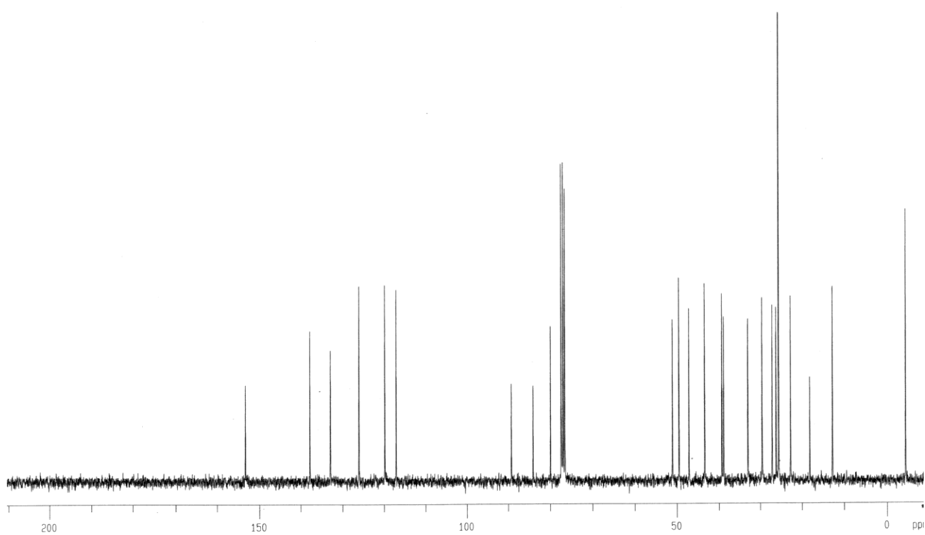
13 C NMR spectrum of 8
