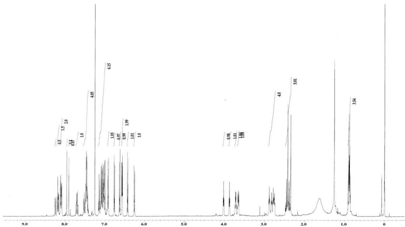
^1\text{H} NMR spectrum of 3
