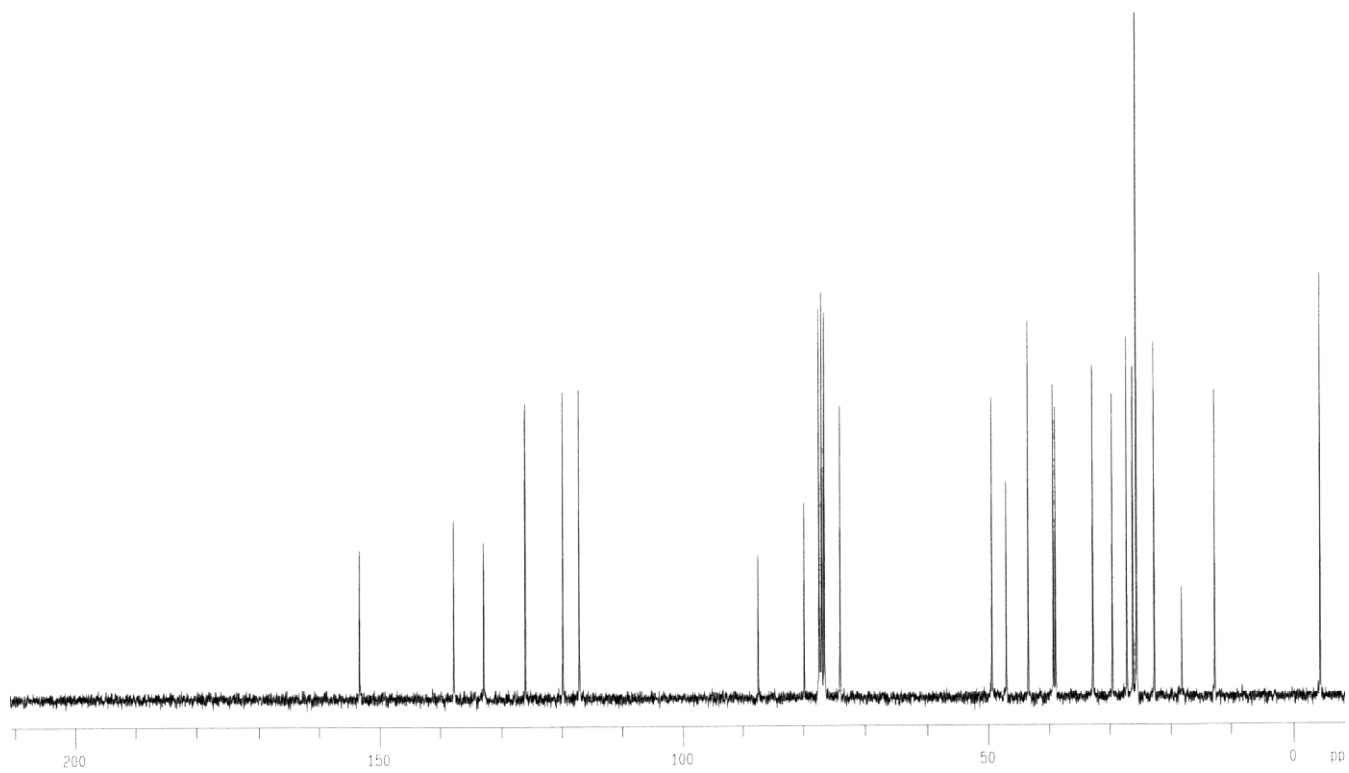
^{13}\text{C} NMR spectrum of 7
