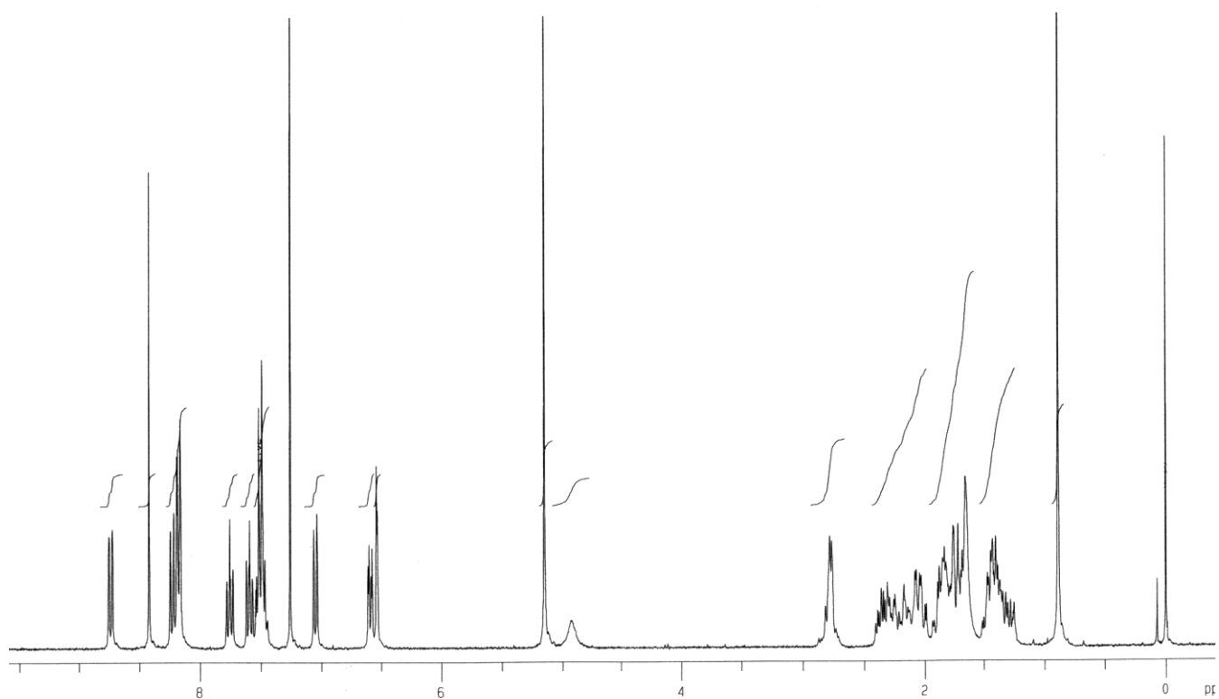
^1\text{H} NMR spectrum of 2
