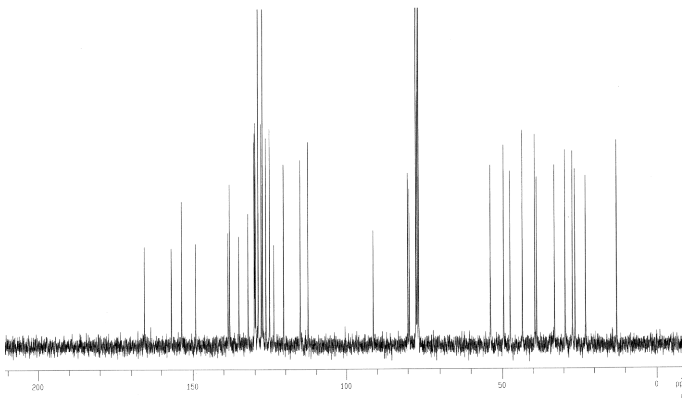
^{13}\text{C} NMR spectrum of 2
