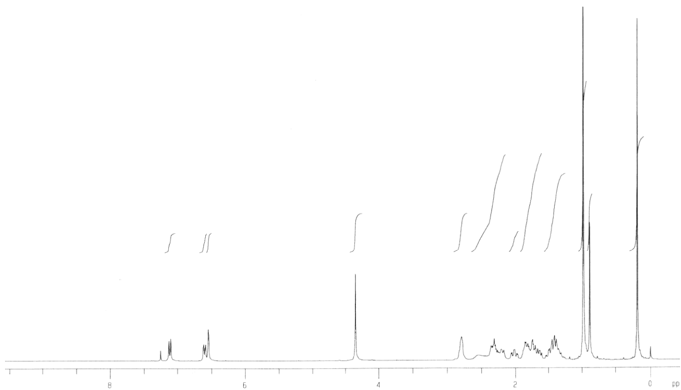
1 H NMR spectrum of 8
