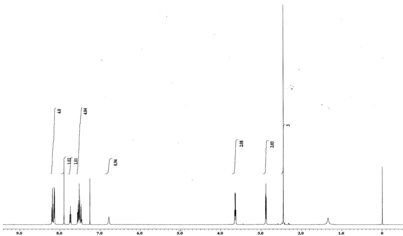
^1\text{H} NMR spectrum of 13
