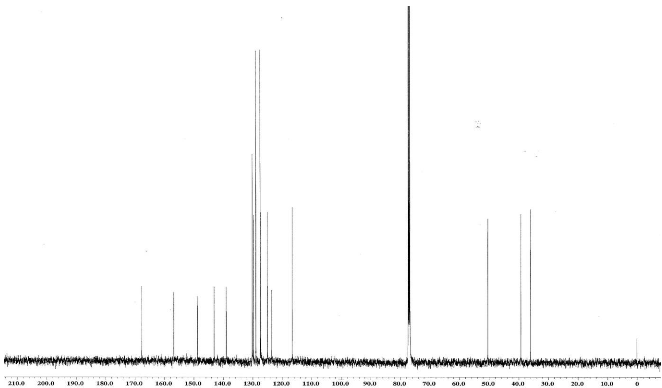
^{13}\text{C} NMR spectrum of 13
