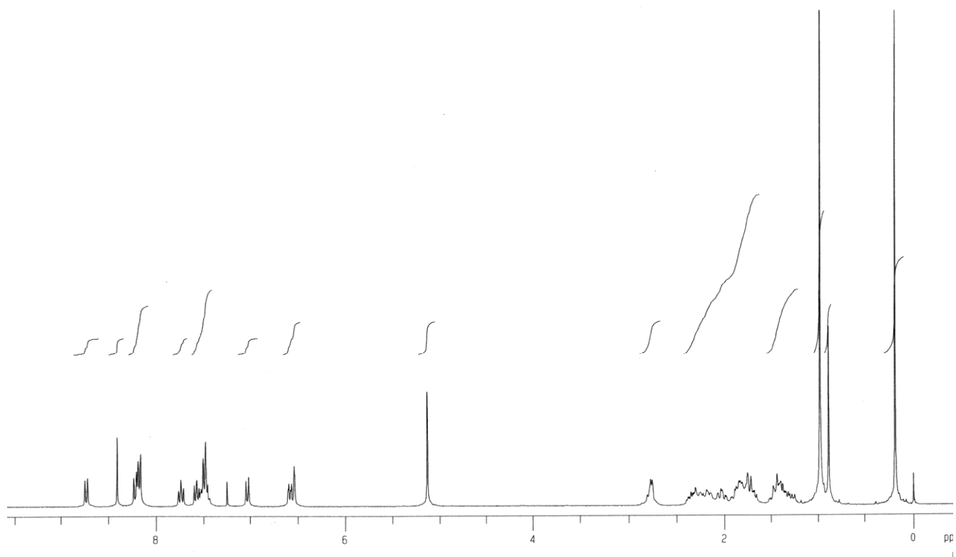
^1\text{H} NMR spectrum of 10
