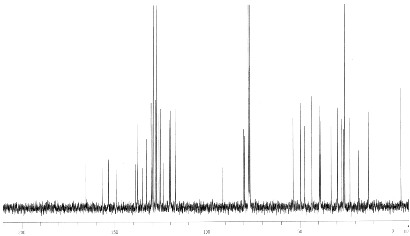
^{13}\text{C} NMR spectrum of 10
