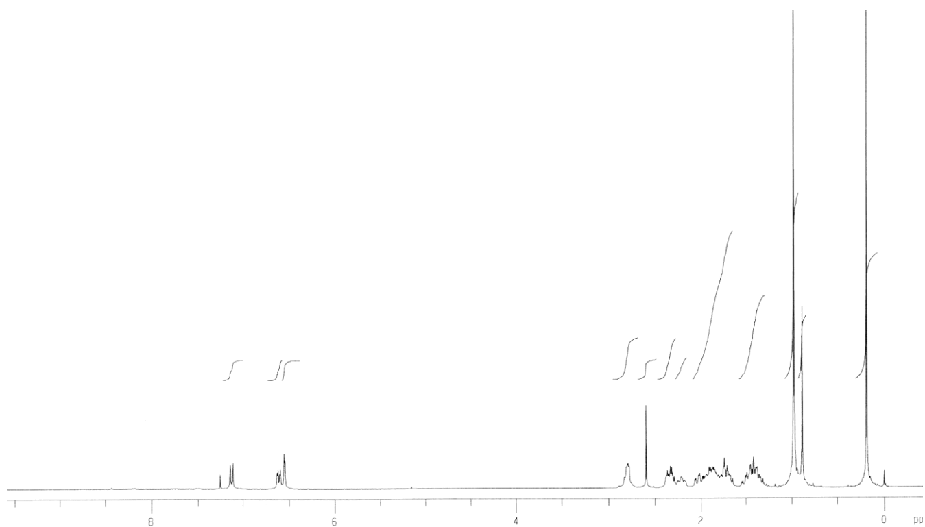
^1\text{H} NMR spectrum of 7
