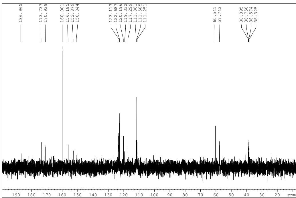
^{13}\text{C} NMR: D 2 O/Na 2 CO 3
