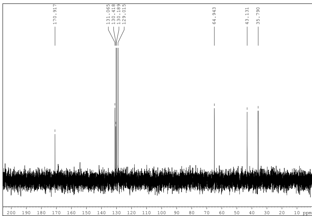
^{13}\text{C} NMR: \text{D}_2\text{O}
