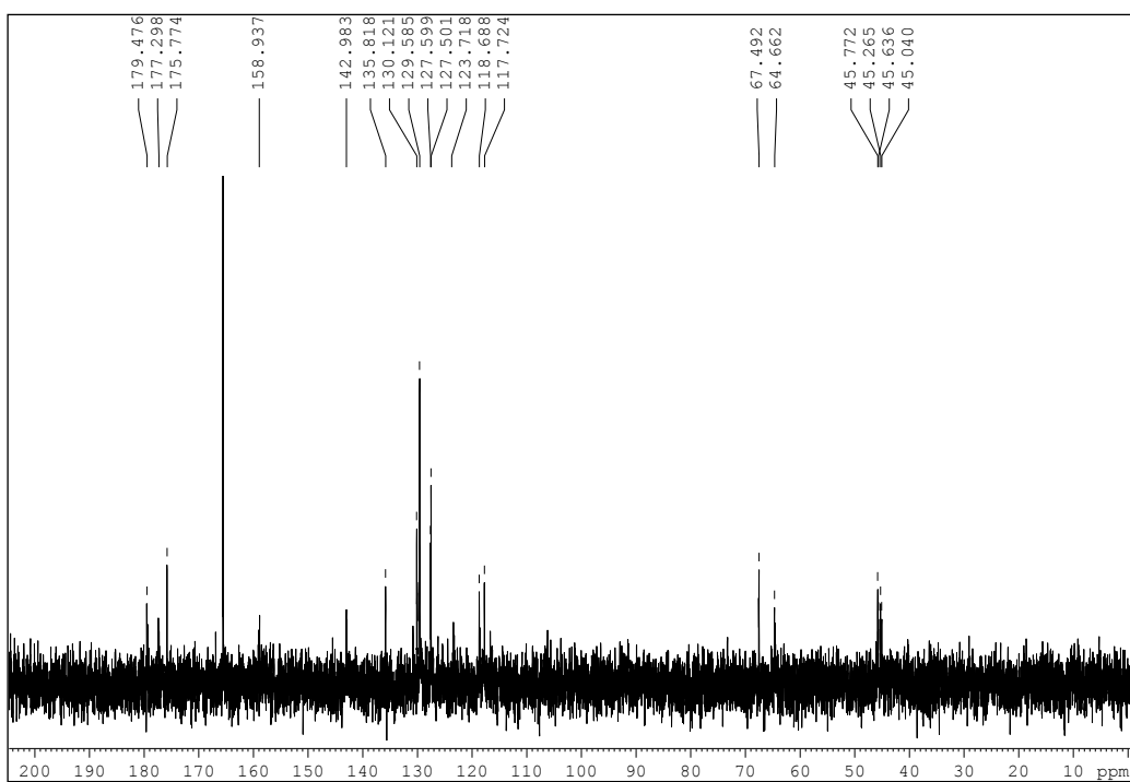
^{13}\text{C} NMR: D 2 O/Na 2 CO 3
