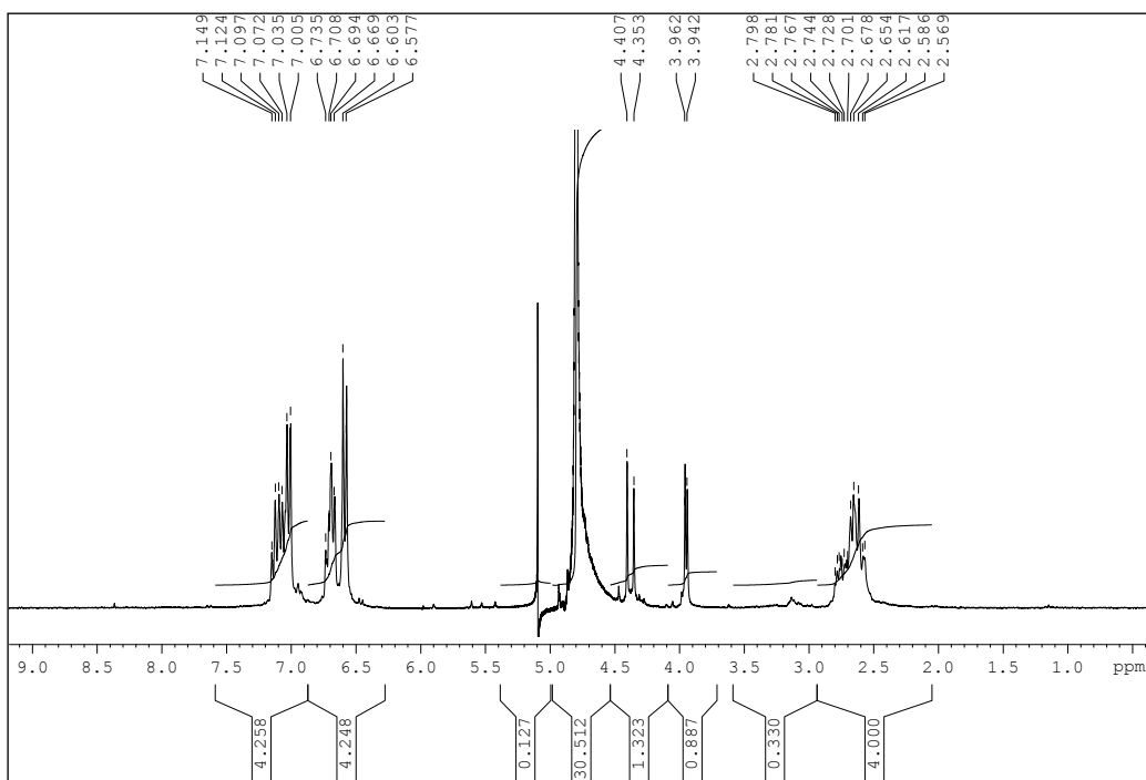
^1\text{H} NMR: D 2 O/Na 2 CO 3
