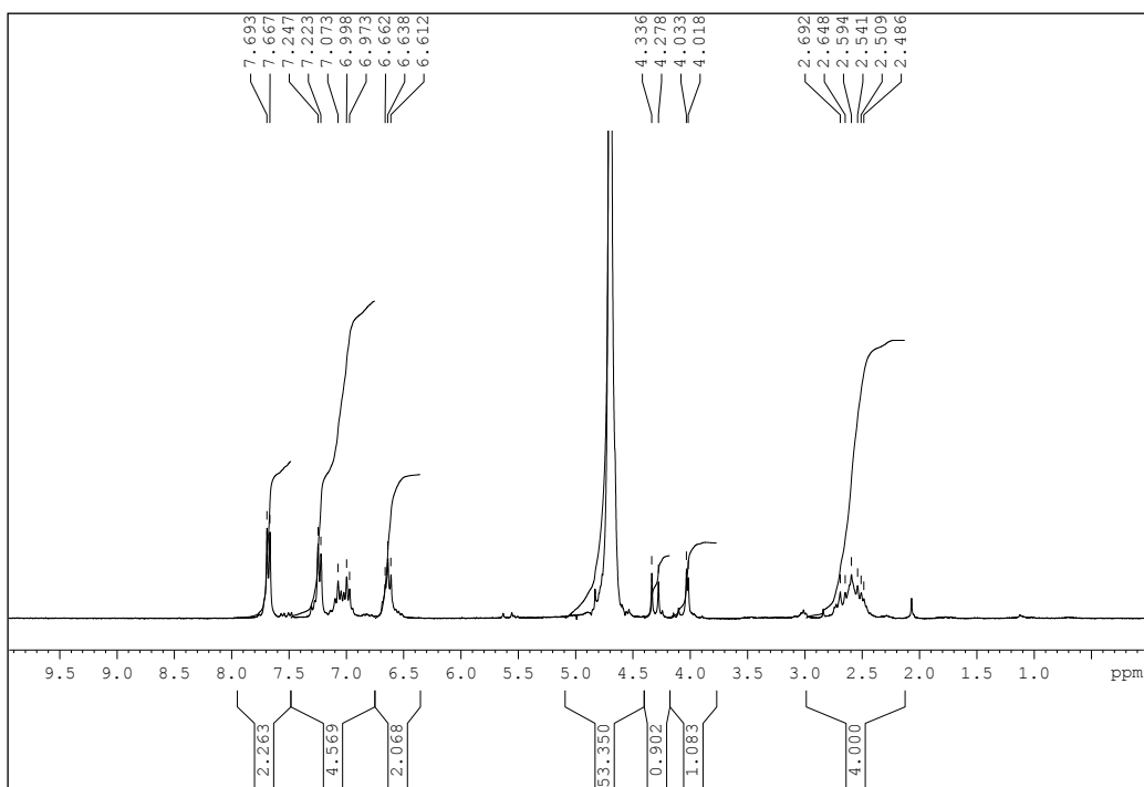
^1\text{H} NMR: D 2 O/Na 2 CO 3
