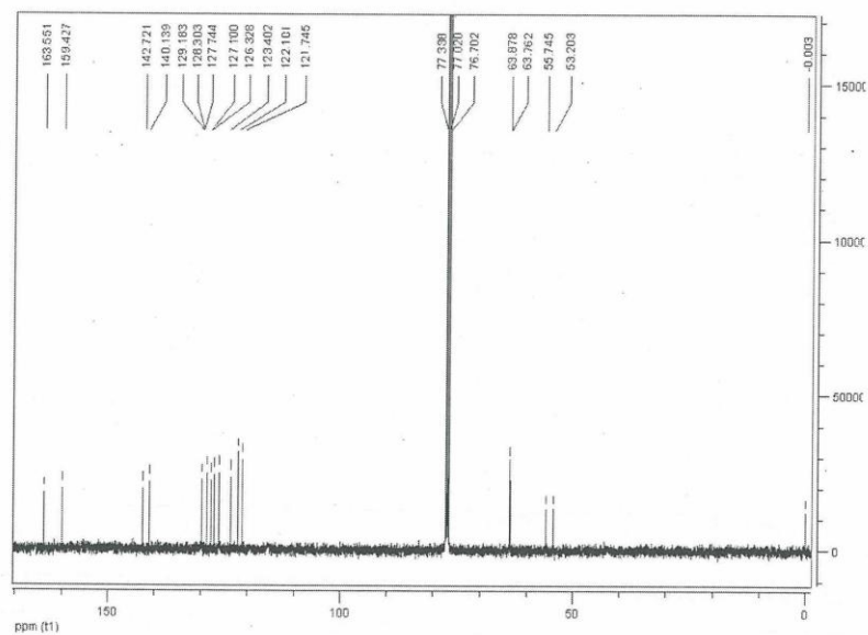
13 C NMR of Compound 3g
