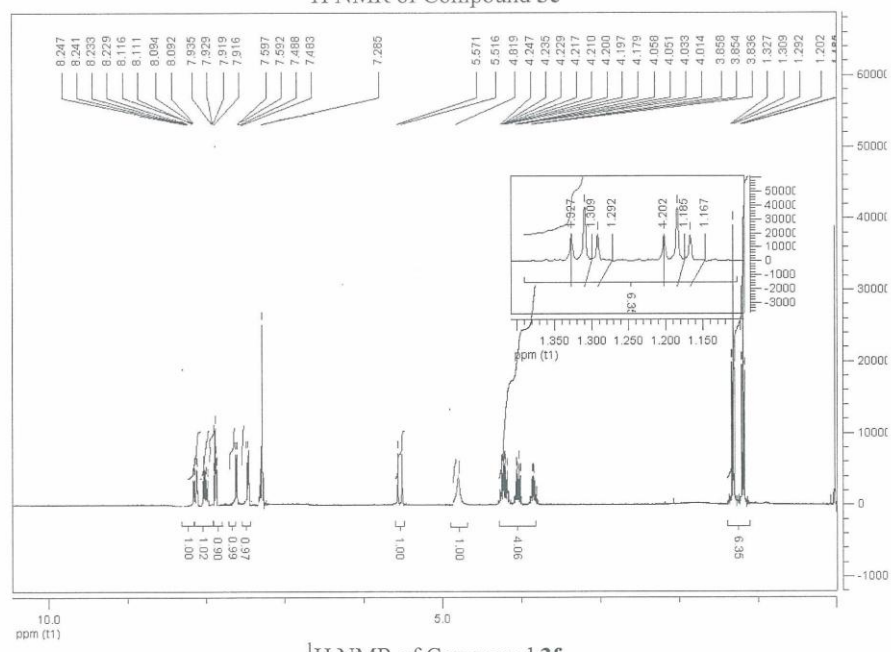
1 H NMR of Compound 3f
