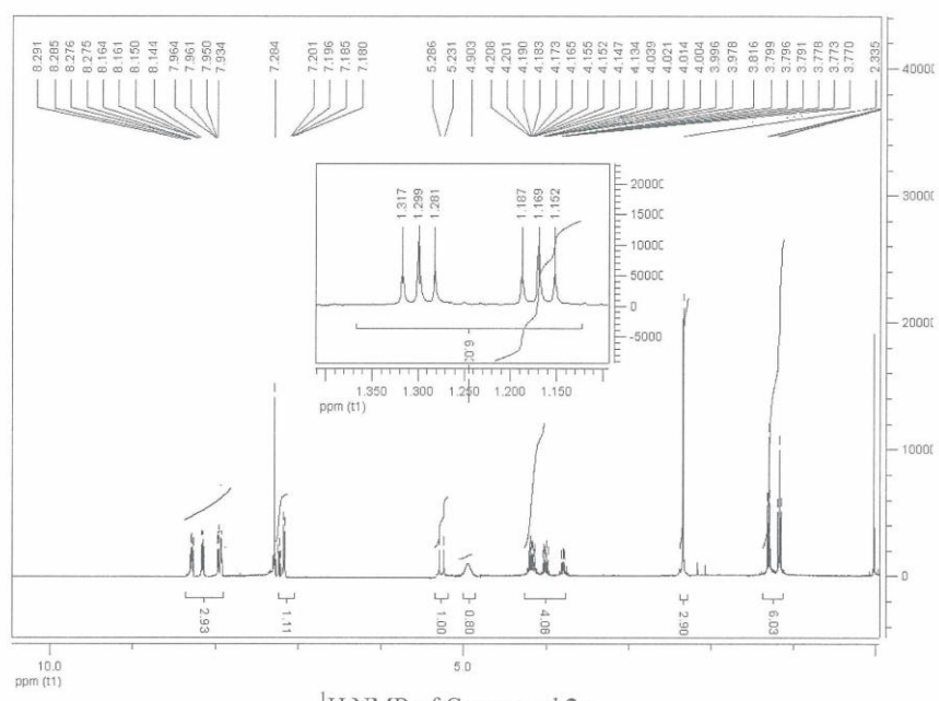
1 H NMR of Compound 3c
