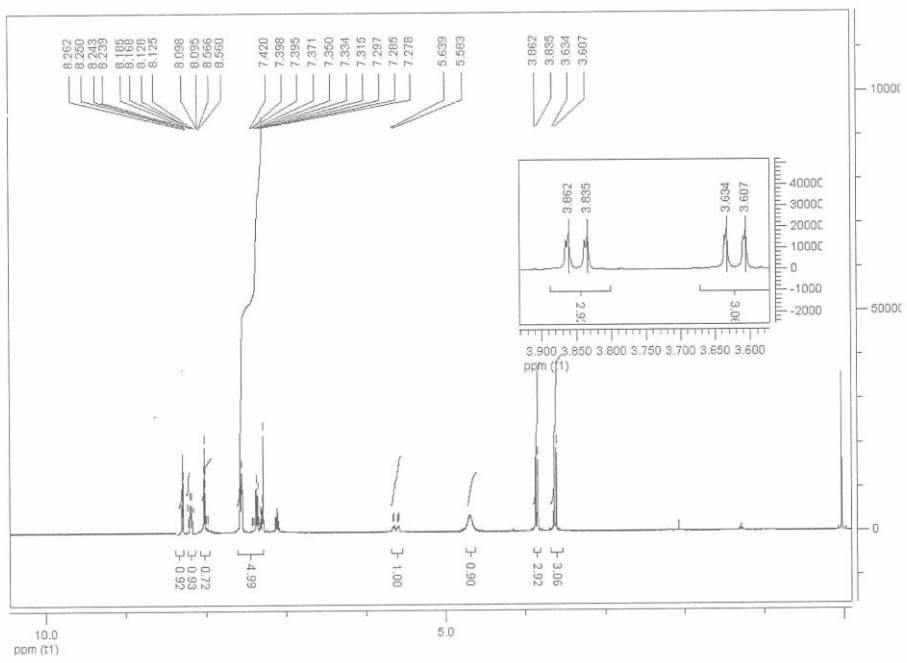
1 H NMR of Compound 3g
