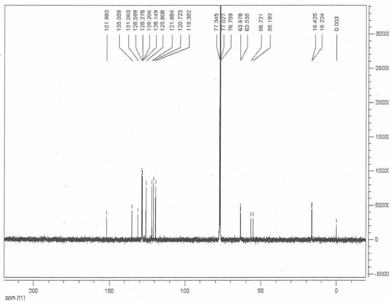
13 C NMR of Compound 9
