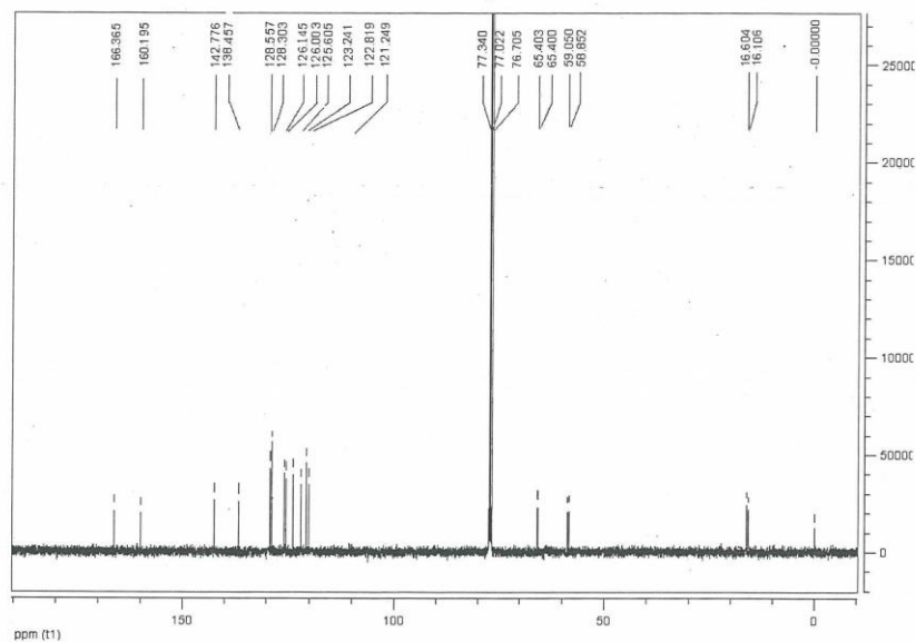
13 C NMR of Compound 3a
