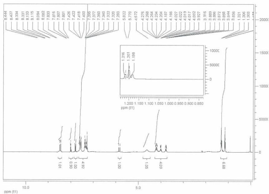
1 H NMR of Compound 3a
