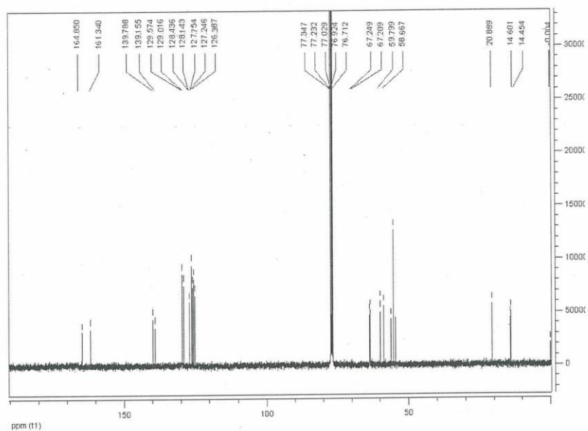
13 C NMR of Compound 3c
