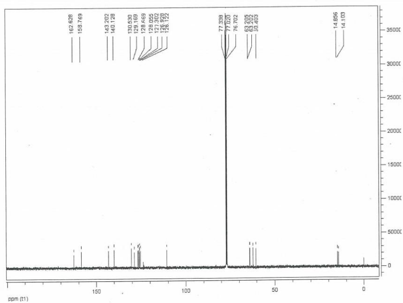
13 C NMR of Compound 3d
