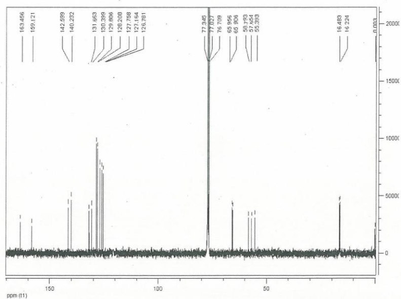
13 C NMR of Compound 3e
