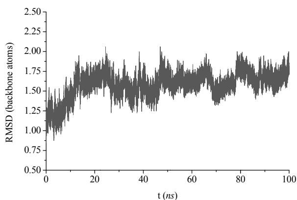
Figure S1. Time evolution of the Root-Mean-Square Deviation (RMSD, in Å) for the protein backbone atoms (except the N -term coil) of the MD trajectory.
