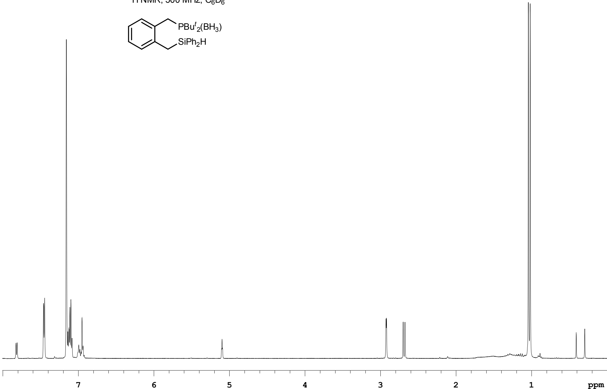
Compound 13 1 H NMR, 500 MHz, C 6 D 6
