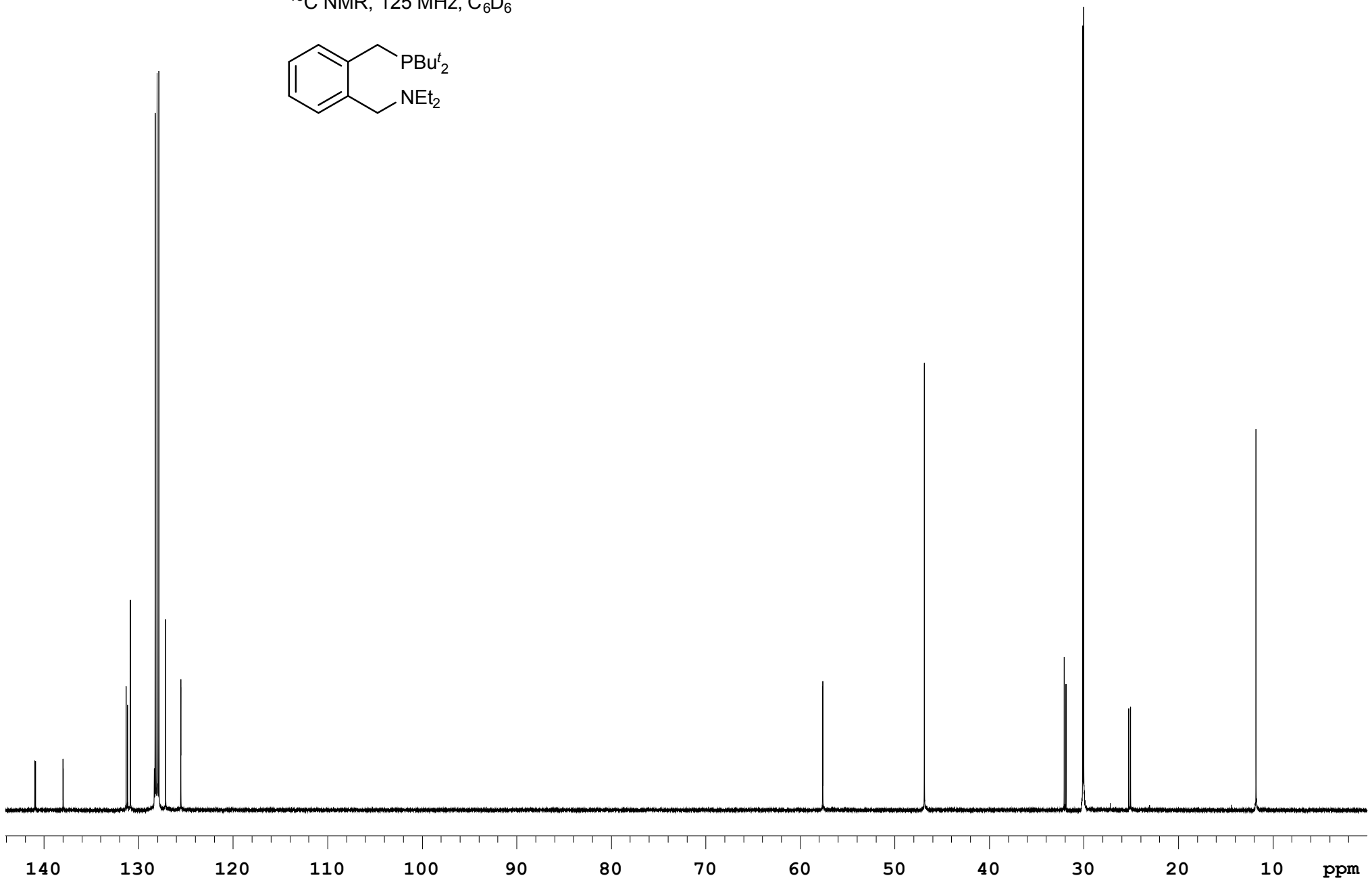
Compound 12c 13 C NMR, 125 MHz, C 6 D 6
