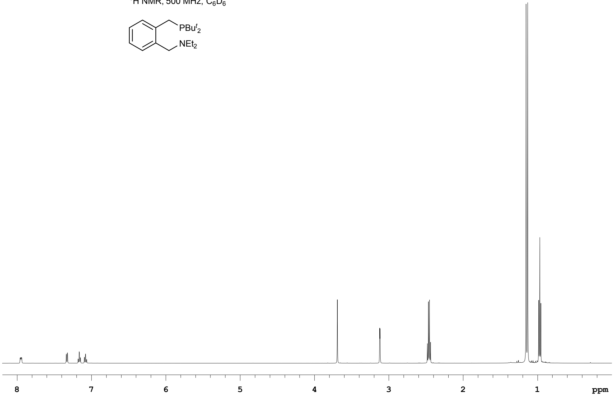
Compound 12c 1 H NMR, 500 MHz, C 6 D 6
