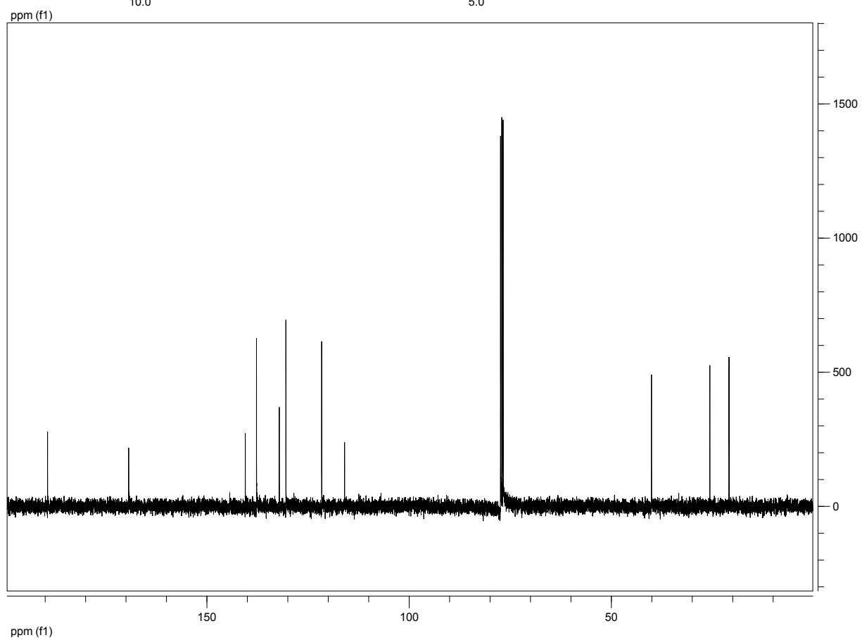
Compound 13b
