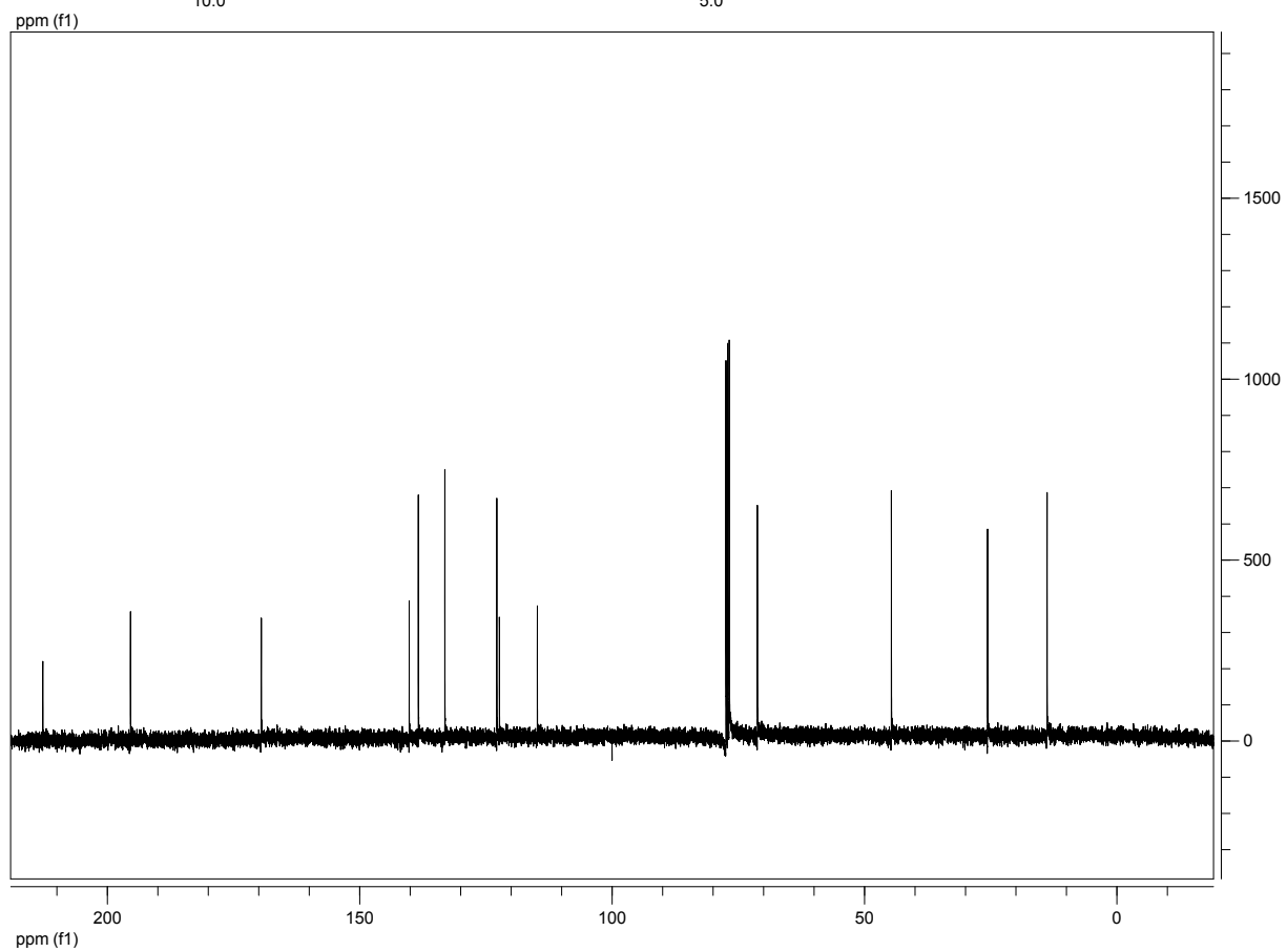
Compound 15c
