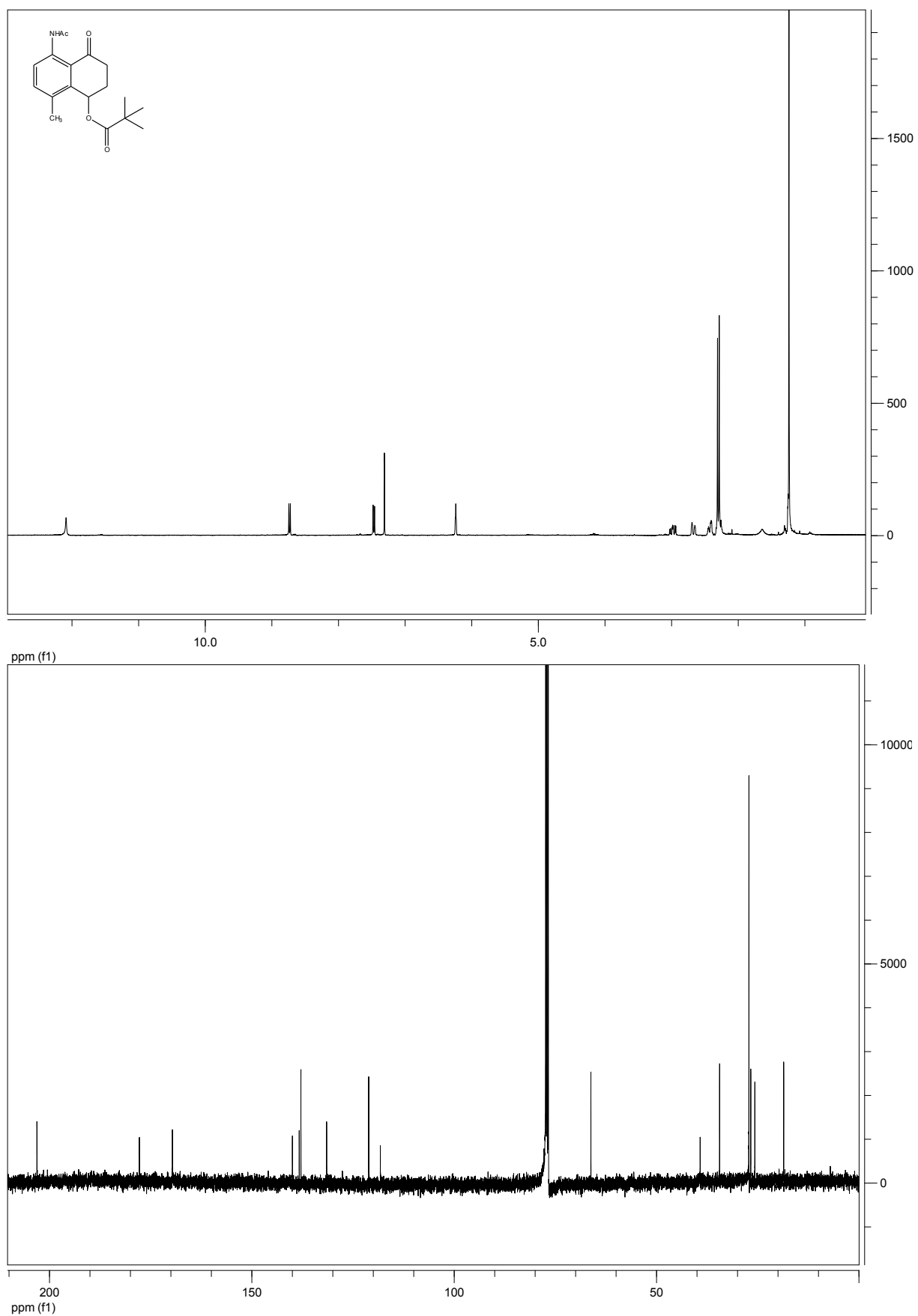
Compound 17b
