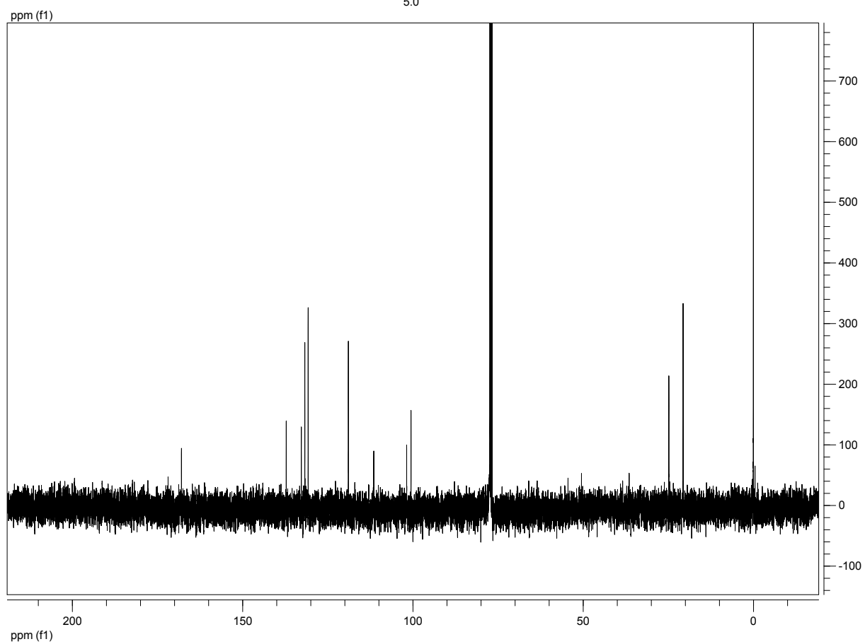
Compound 12b
