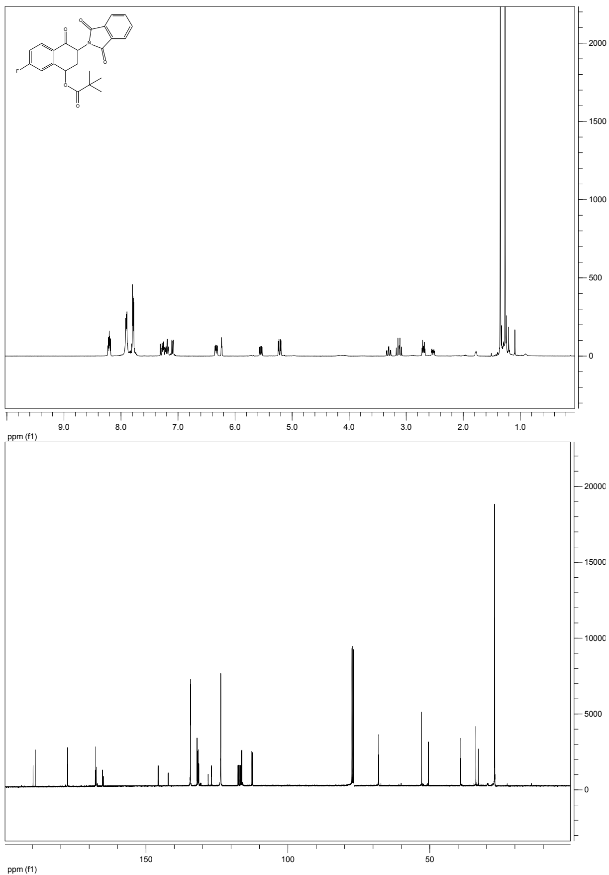
Compound 6c
