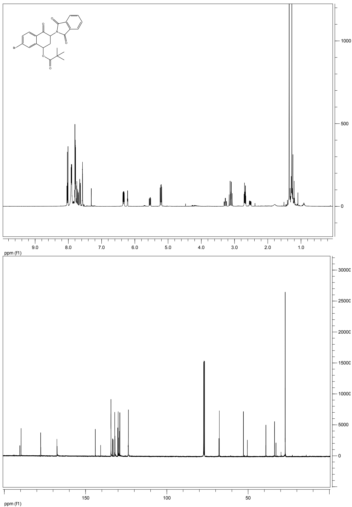
Compound 6d
