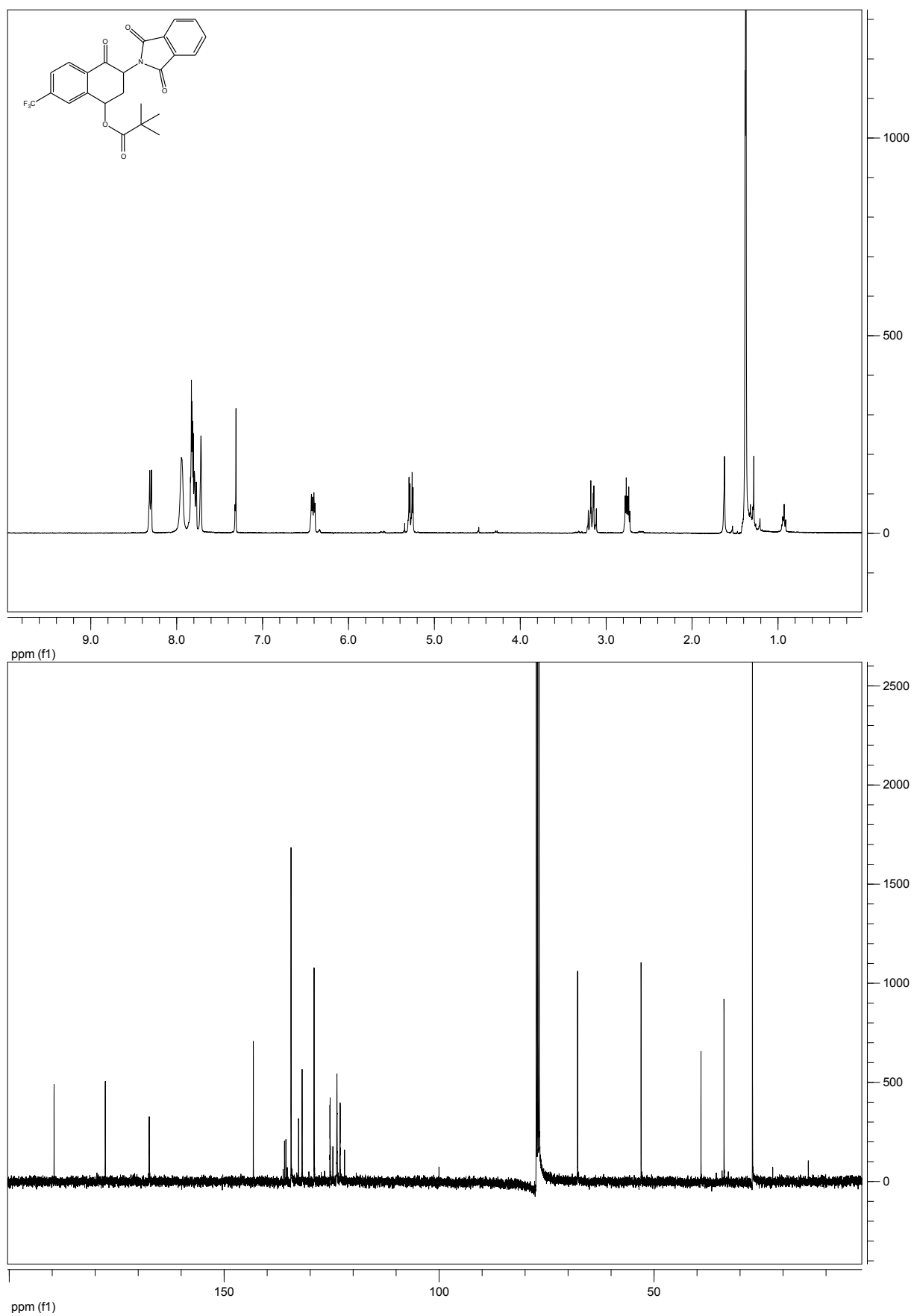
Compound 7a
