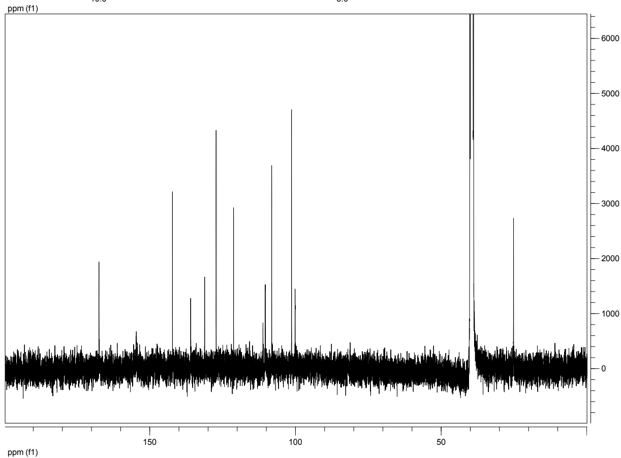
Compound 19c
