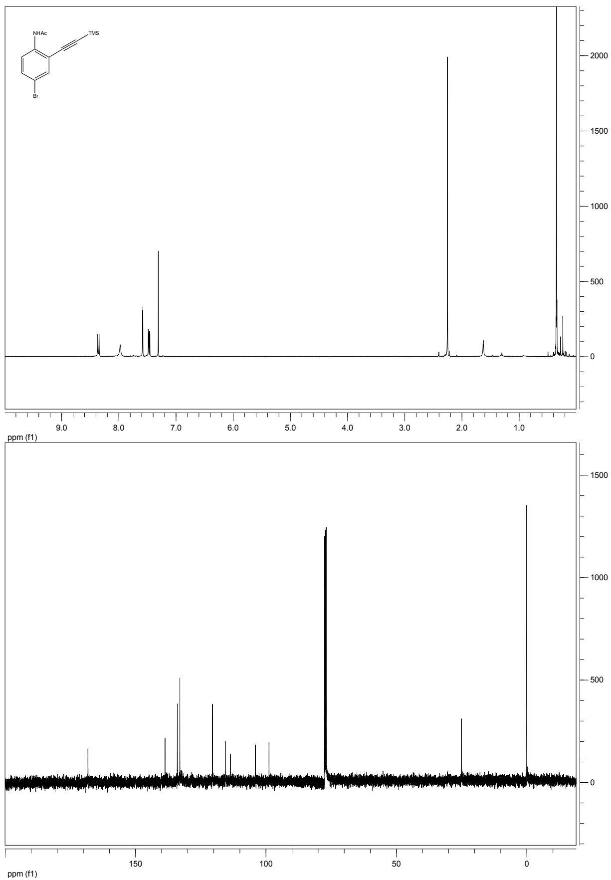
Compound 12c
