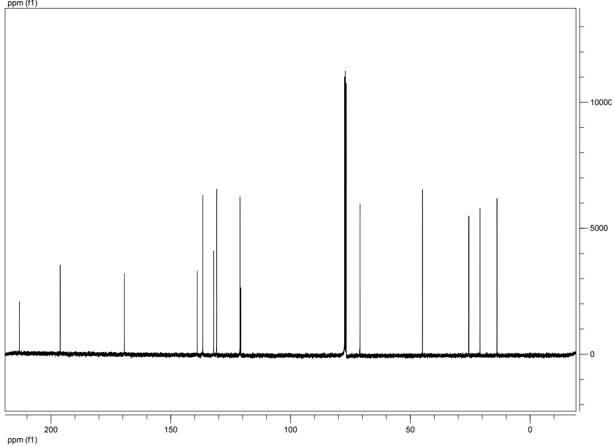
Compound 15b
