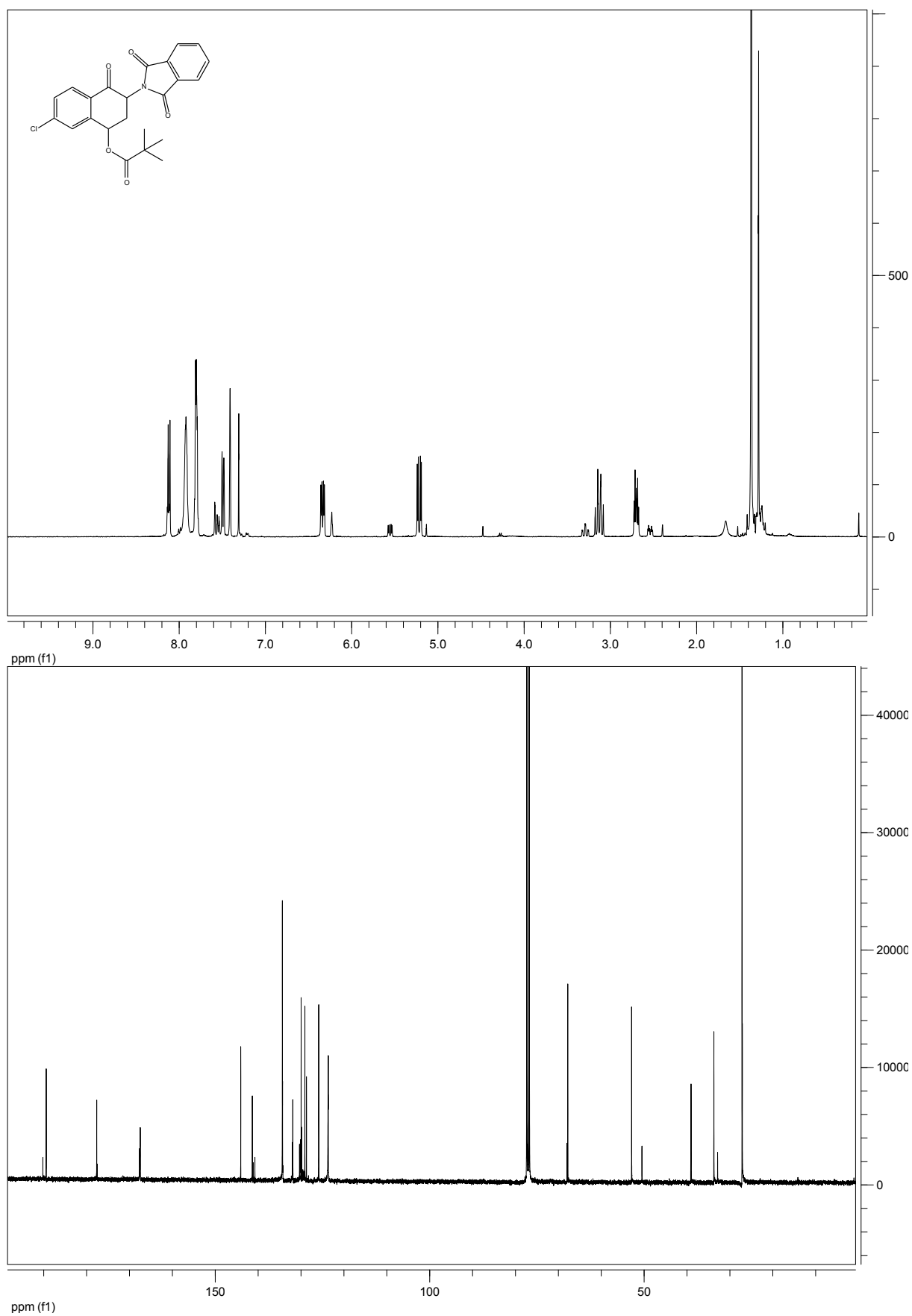
Compound 6e
