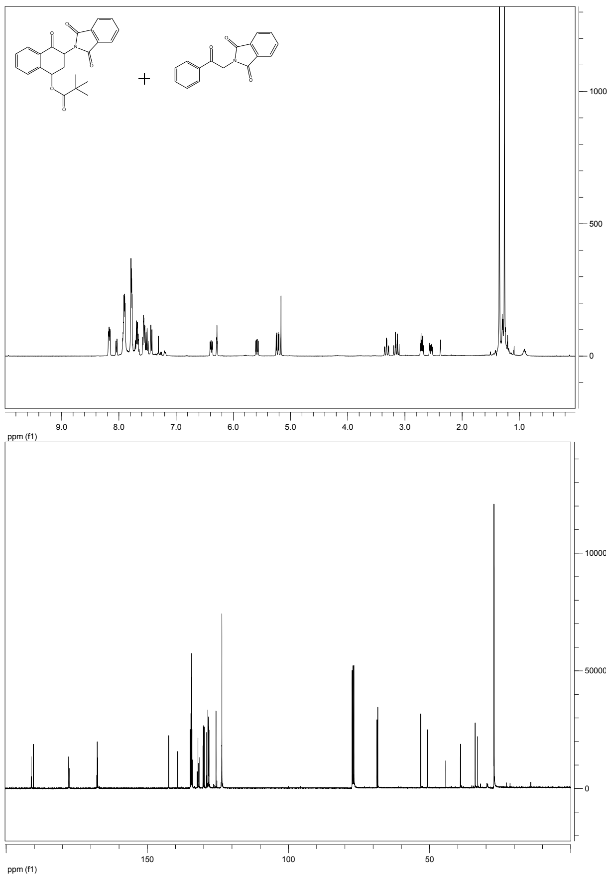
Compound 6b
