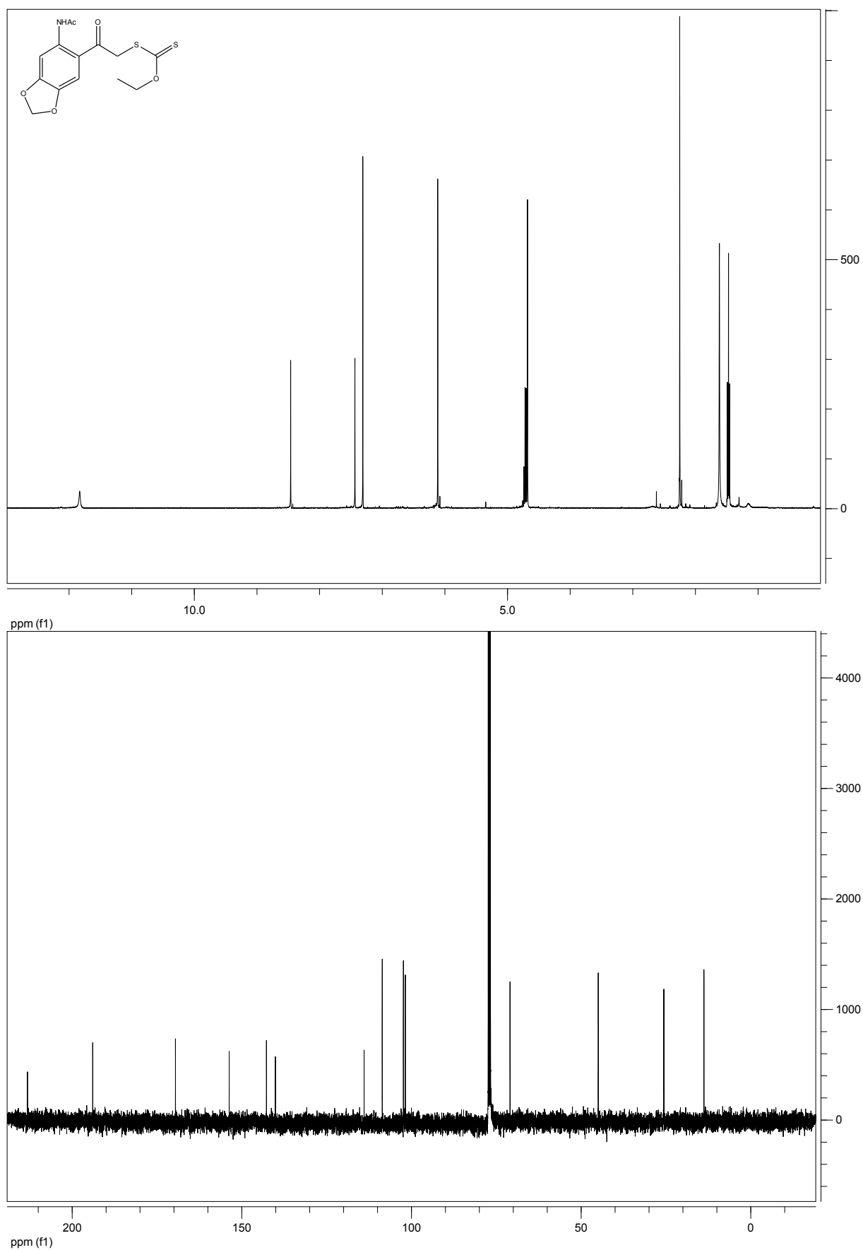
Compound 17a
