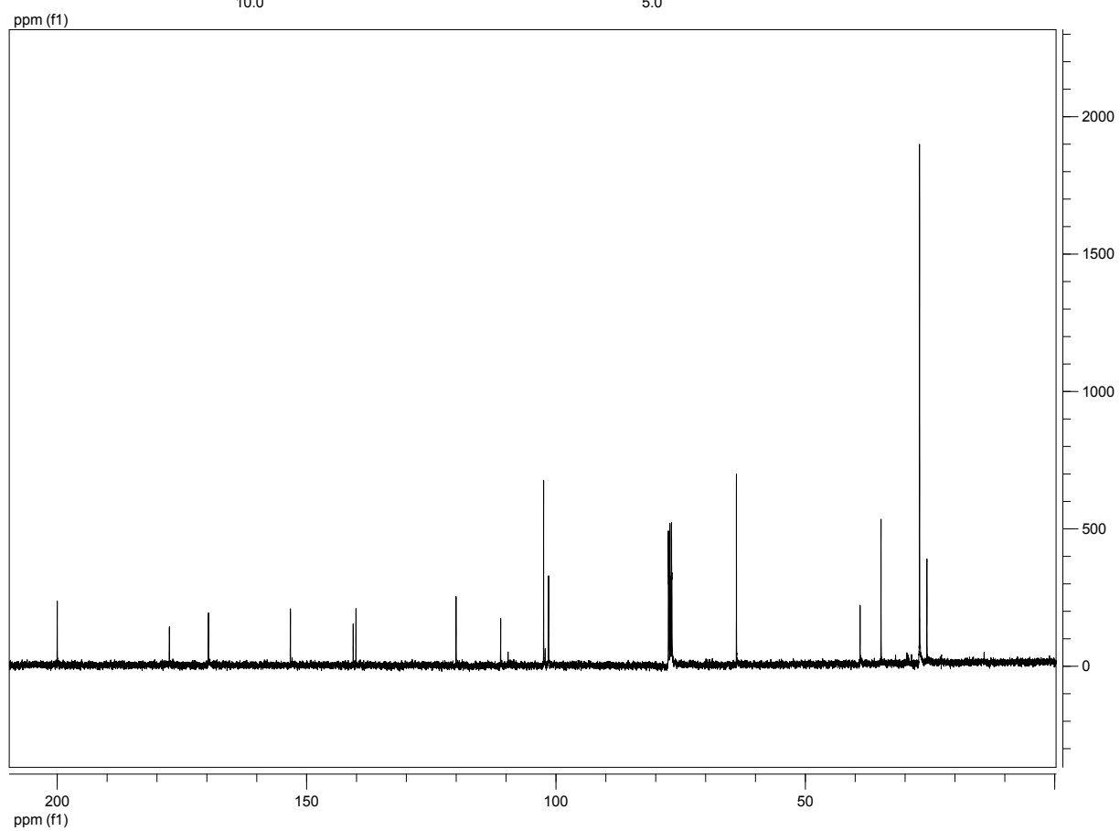
Compound 18a
