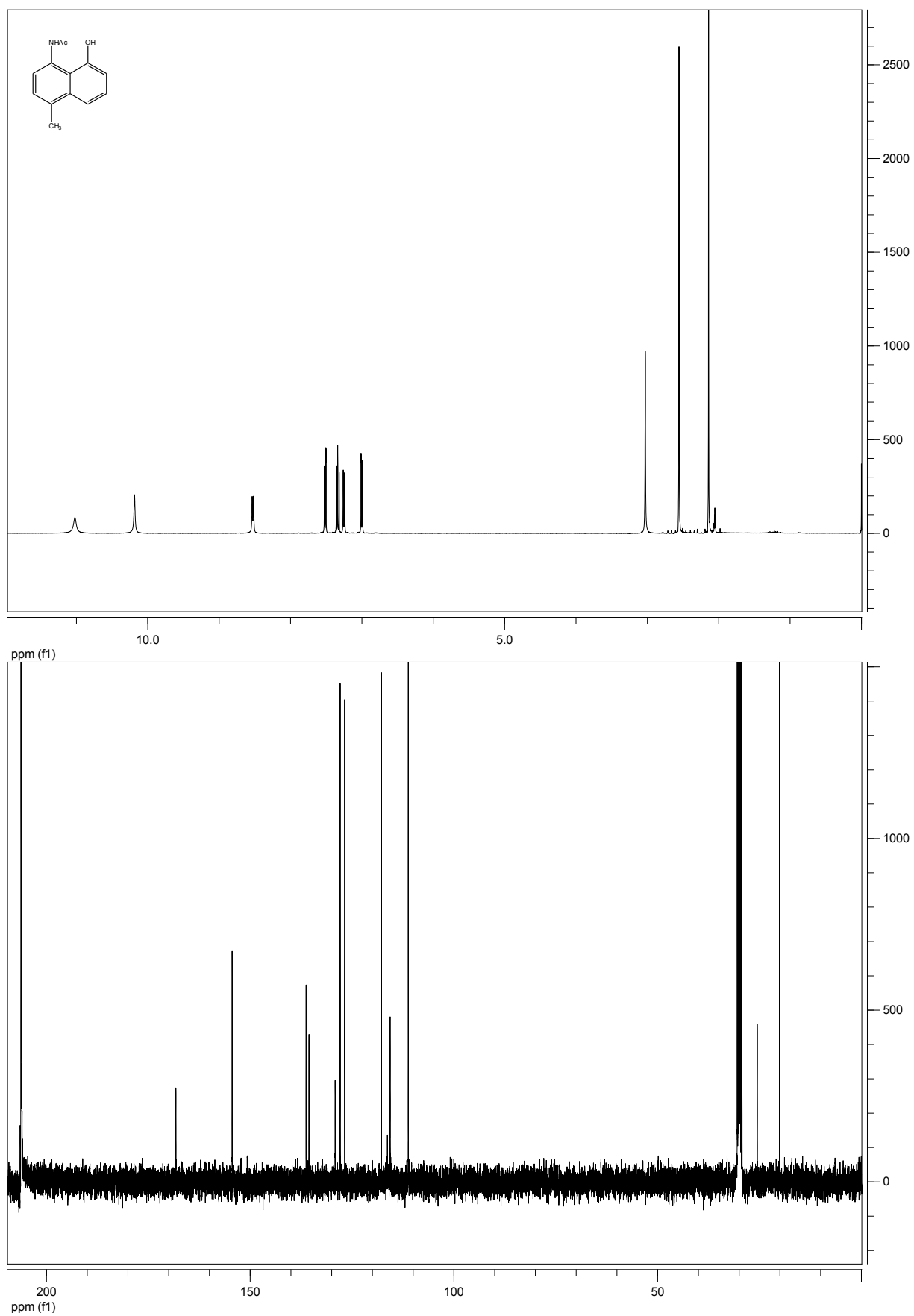
Compound 18b
