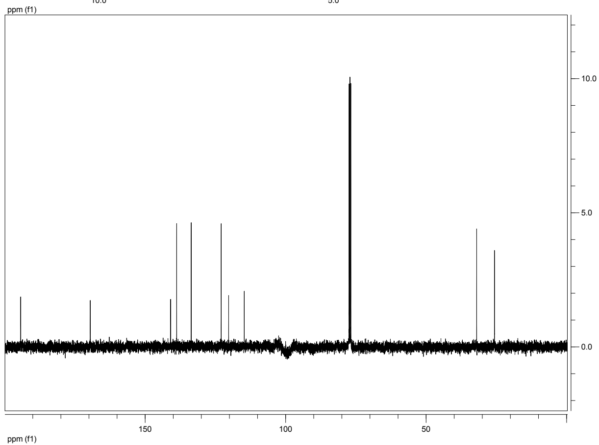
Compound 14c
