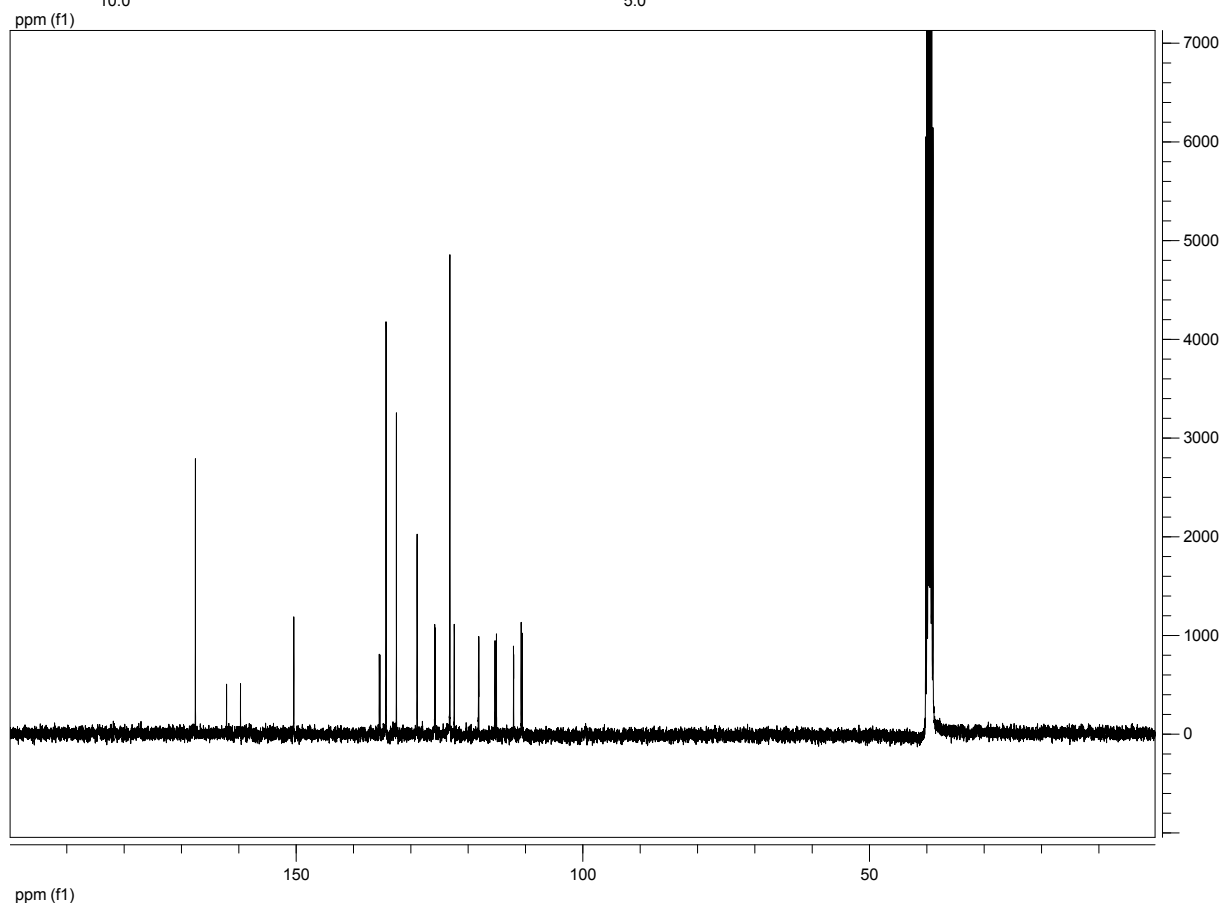
Compound 7c
