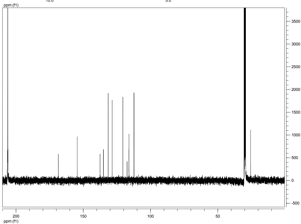
Compound 18c
