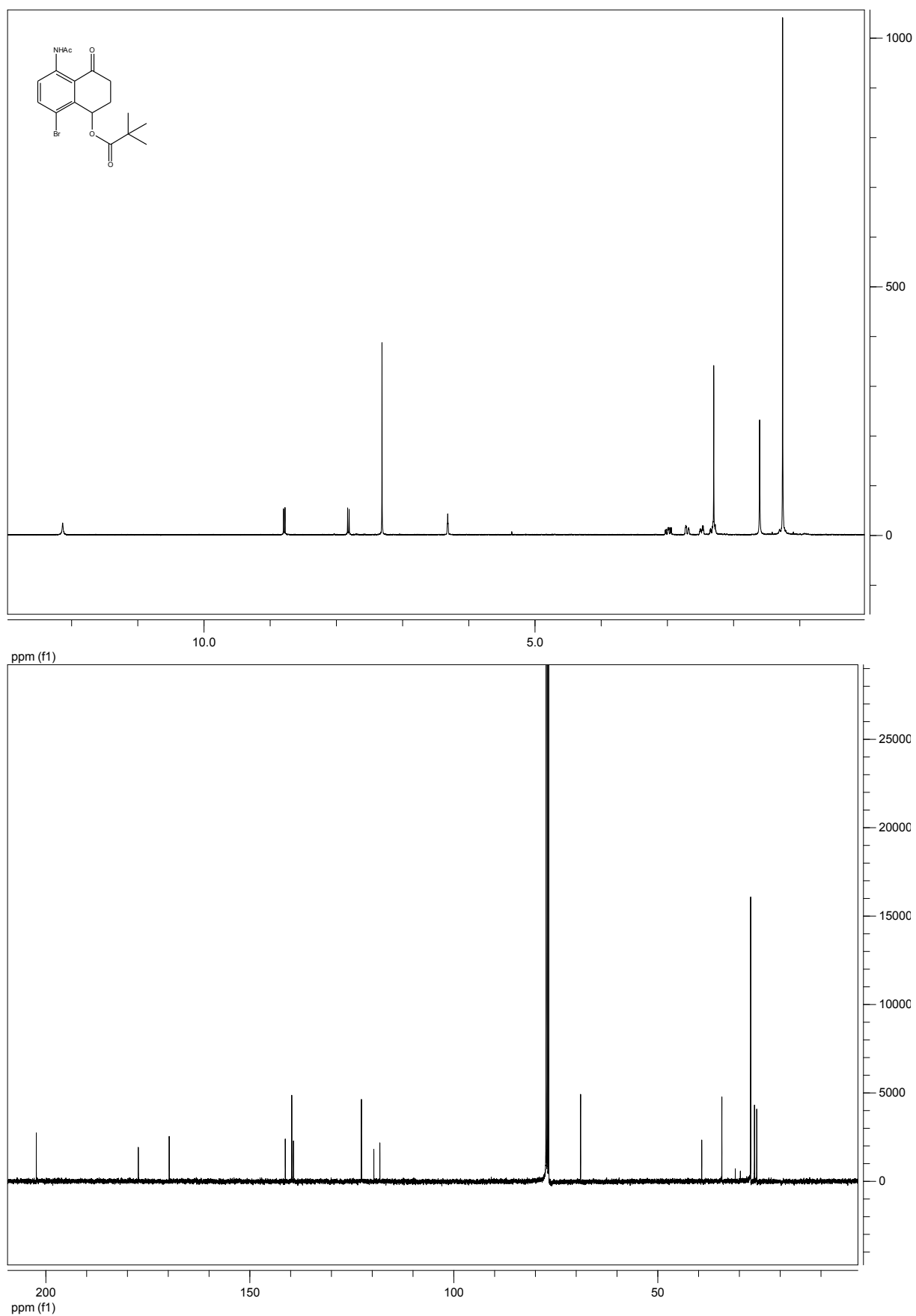
Compound 17c
