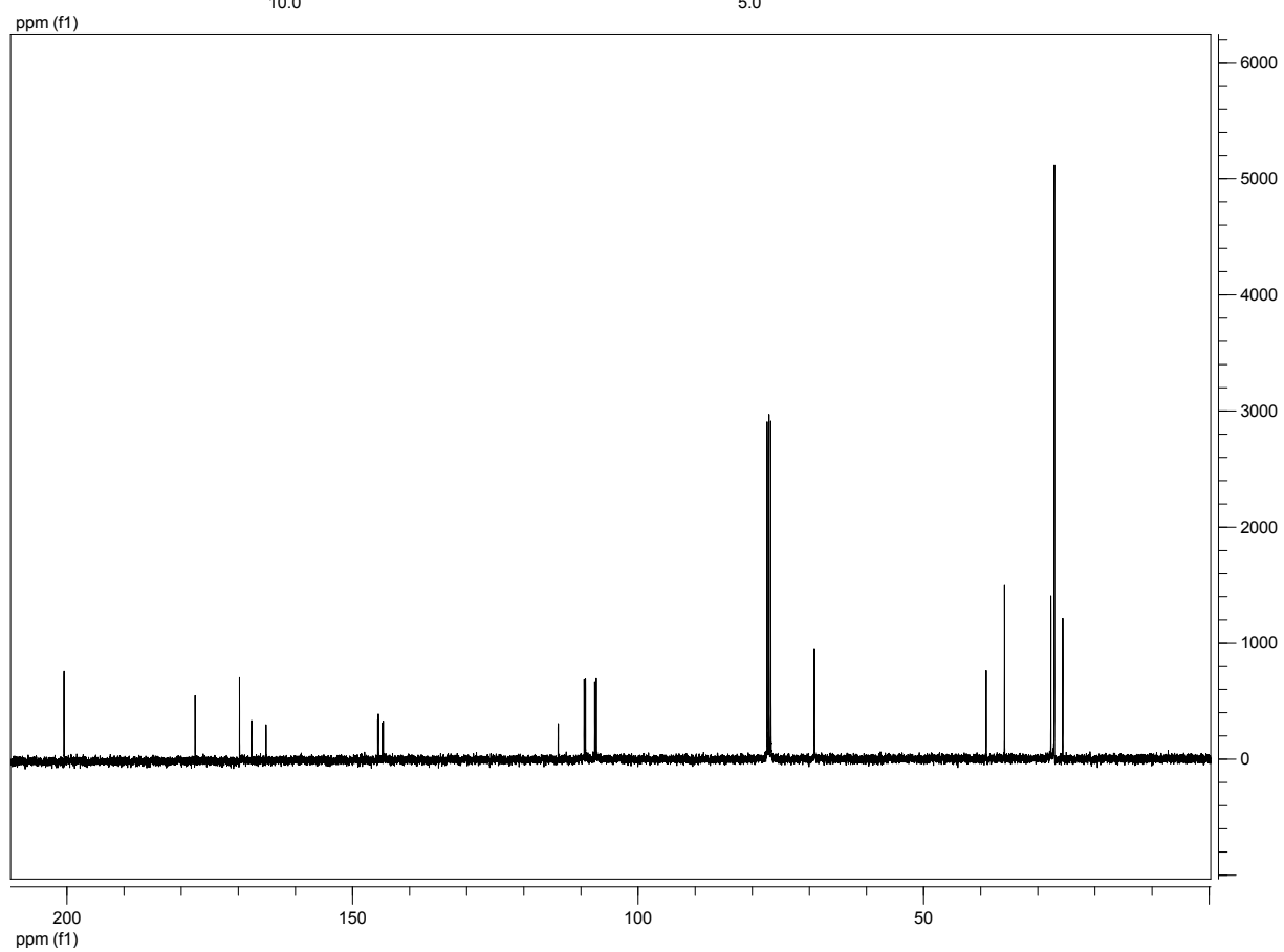
Compound 17e
