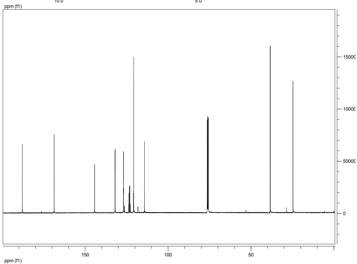
Compound 14a
