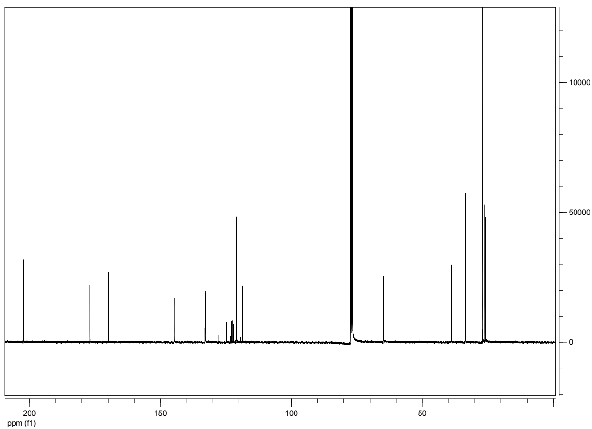
Compound 17d
