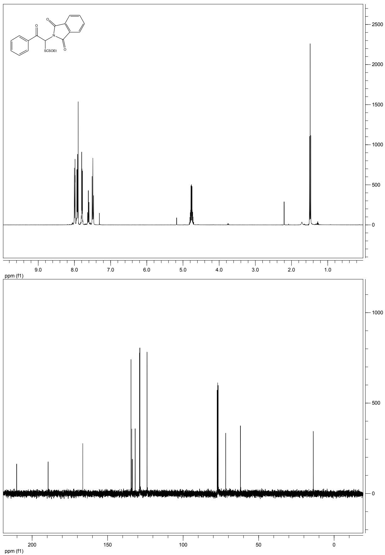
Compound 4b
