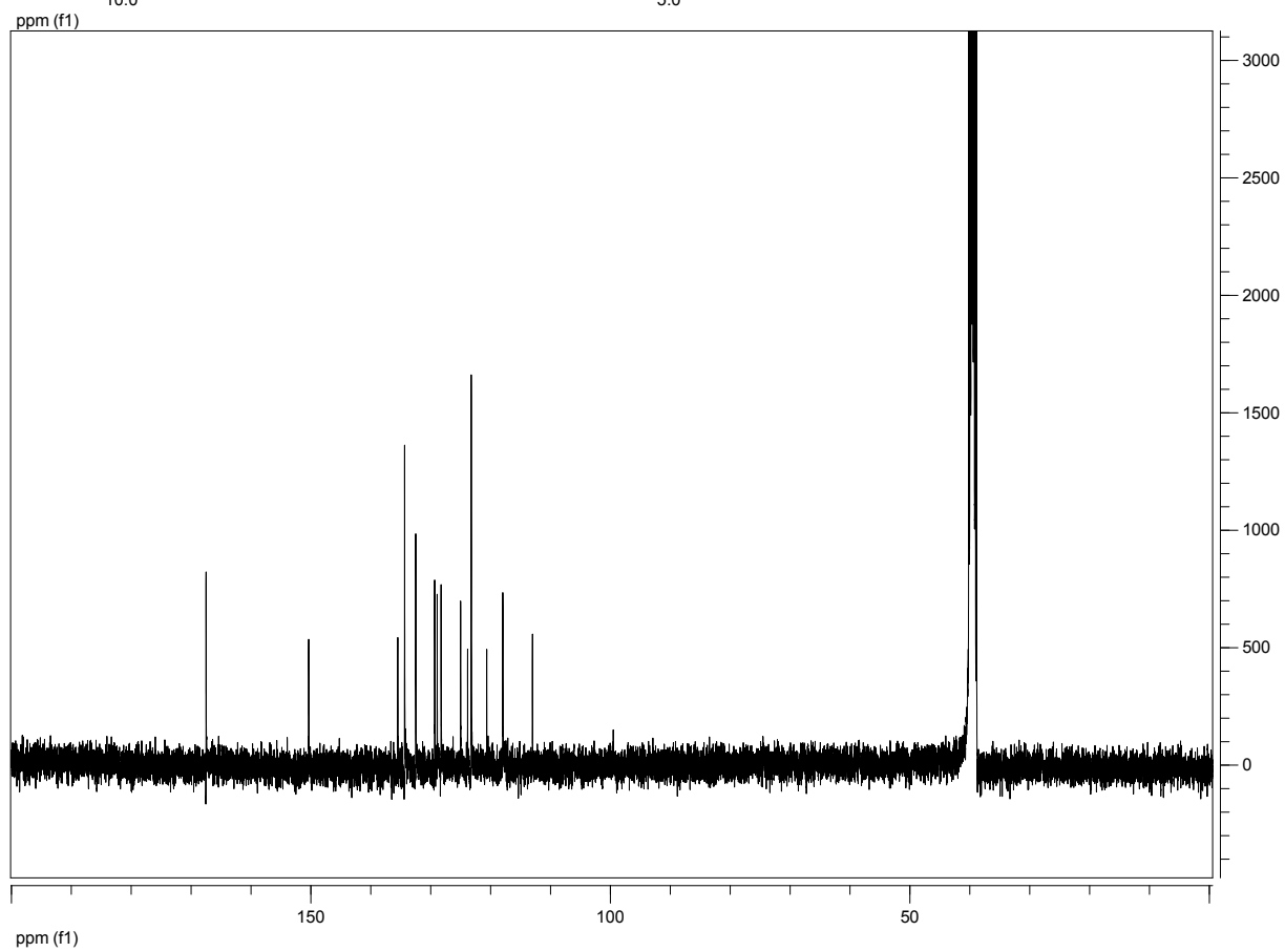
Compound 7d
