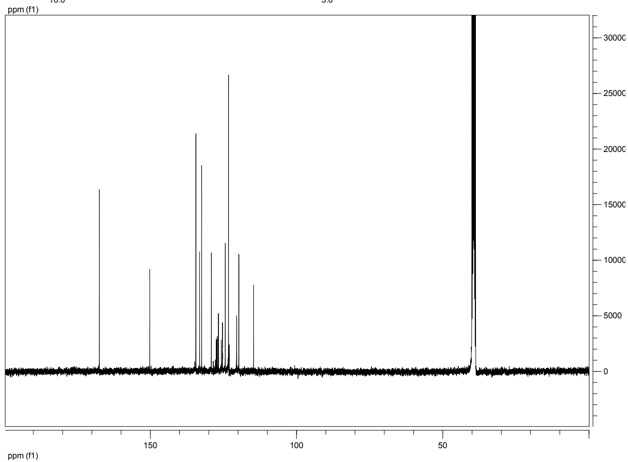
Compound 12a
