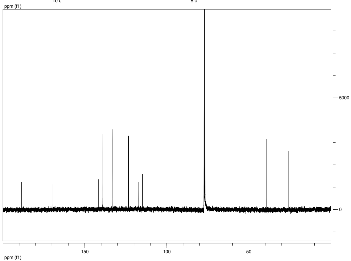
Compound 13c
