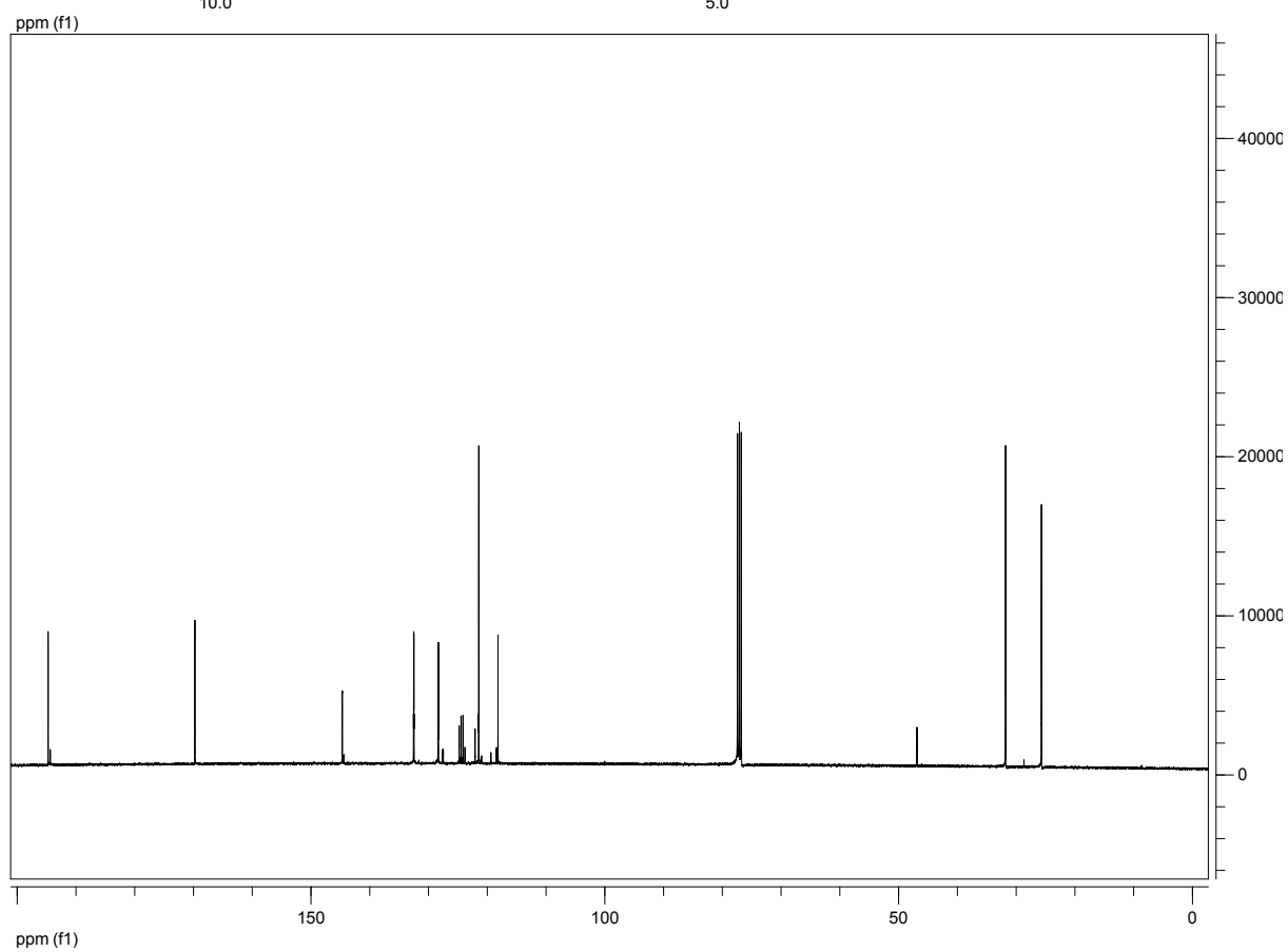
Compound 15a
