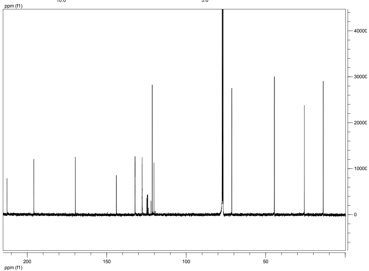
Compound 15d
