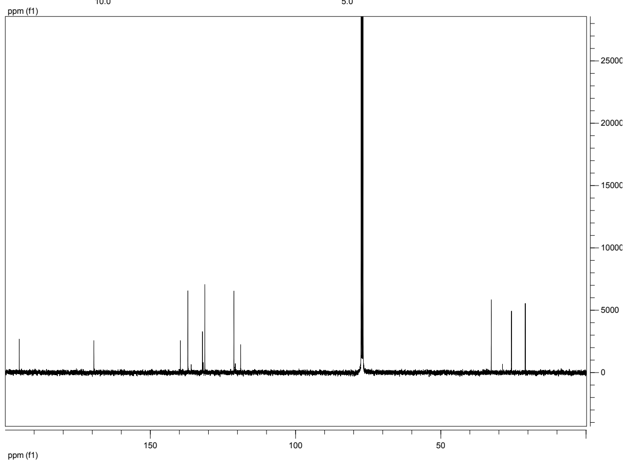
Compound 14b
