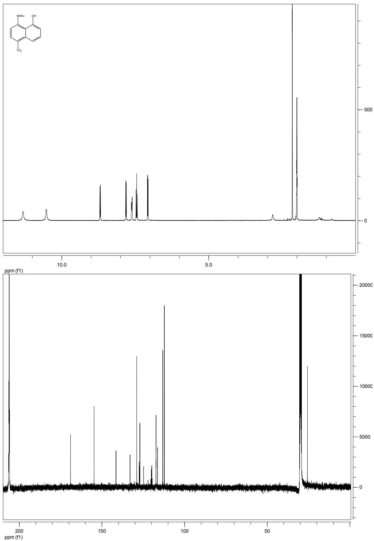
Compound 18d
