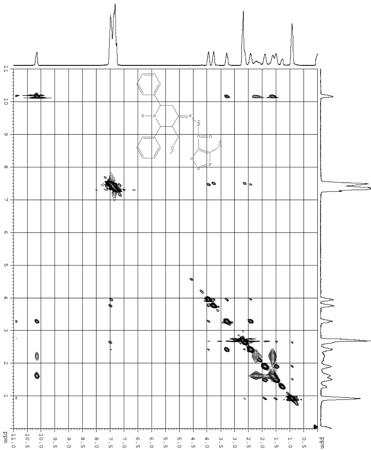
1 H- 1 H NOESY NMR Spectrum of 4-Methyl-N'-(3-ethyl-2r,6c-diarylpiperidin-4-ylidene)-1,2,3-thiadiazole-5-carbohydrazide (5g)
