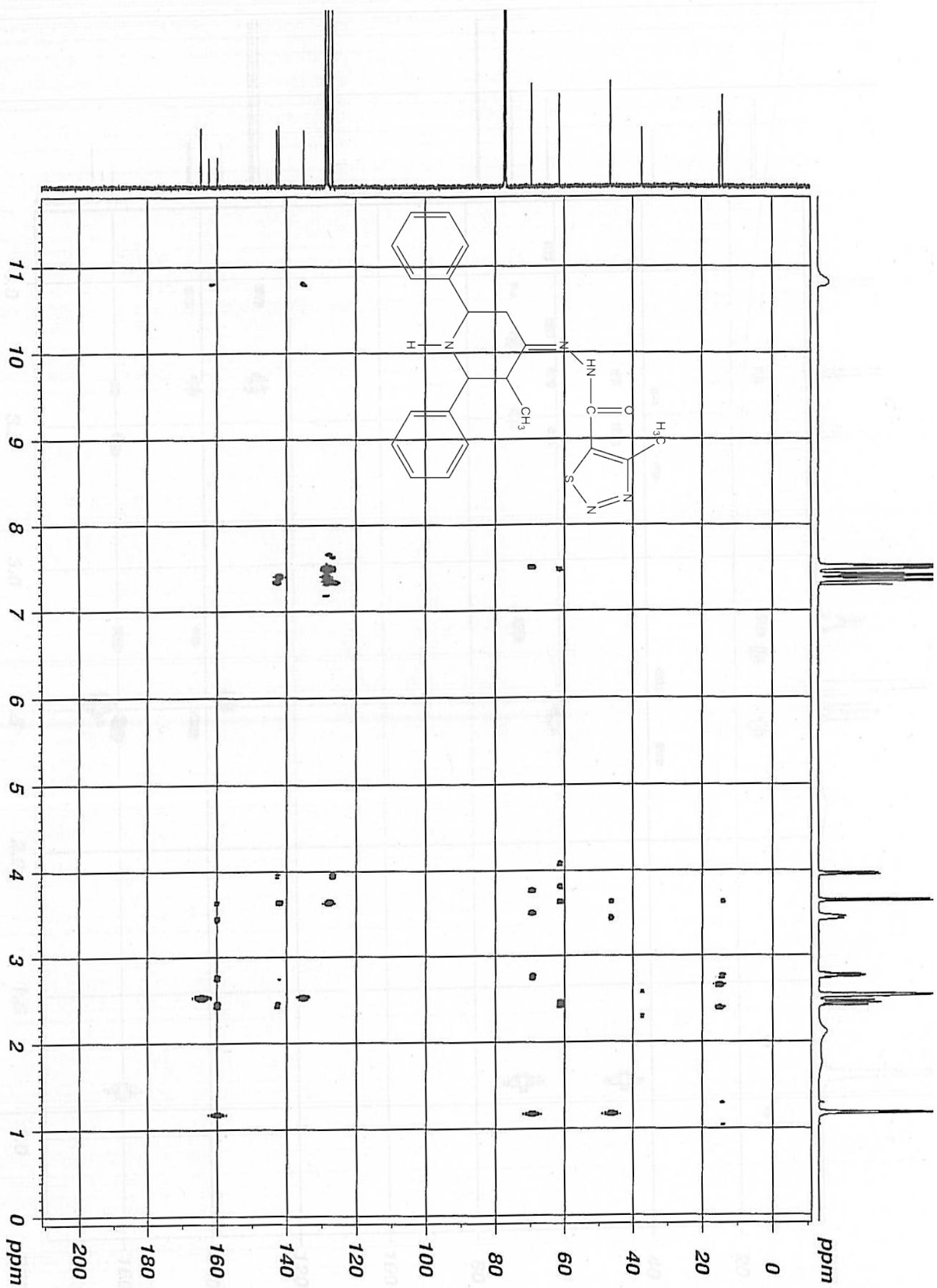
HMBC NMR Spectrum of 4-Methyl-N'-(3-methyl-2,6-diaryl(piperidin-4-ylidene)-1,2,3-thiadiazole-5-carbohydrazide (5a)
