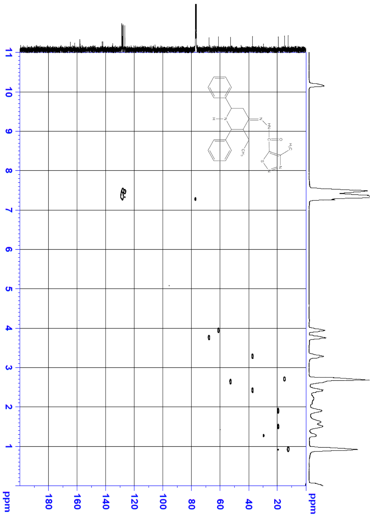
HSQC NMR Spectrum of 4-Methyl-N'-(3-ethyl-2r,6c-diaryl)piperidin-4-ylidene)-1,2,3-thiadiazole-5-carbohydrazide (5g)
