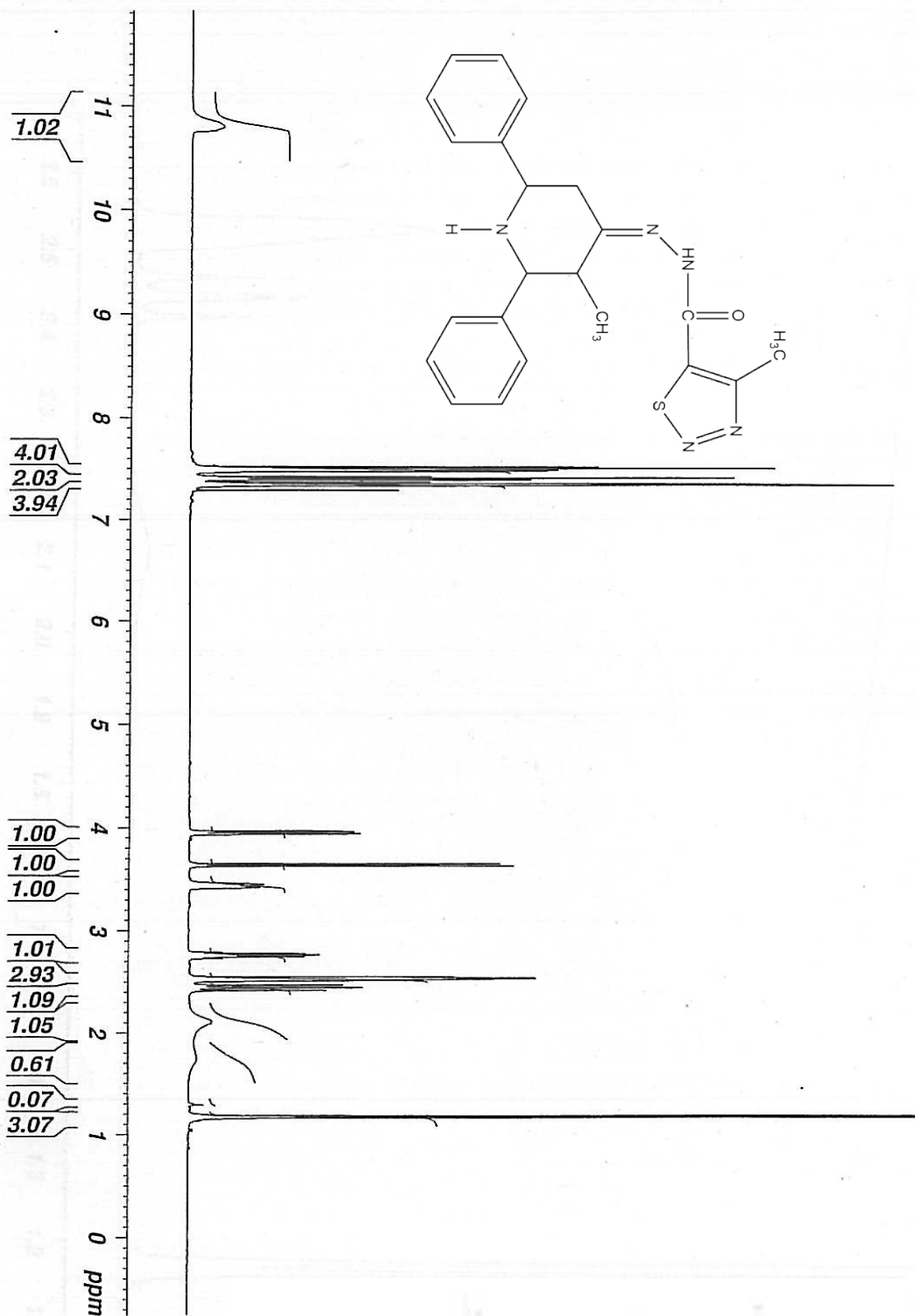
1 H NMR Spectrum of 4-Methyl-N'-(3-methyl-2,6-diaryl-1-piperidin-4-ylidene)-1,2,3-thiadiazole-5-carbohydrazide (5a)
