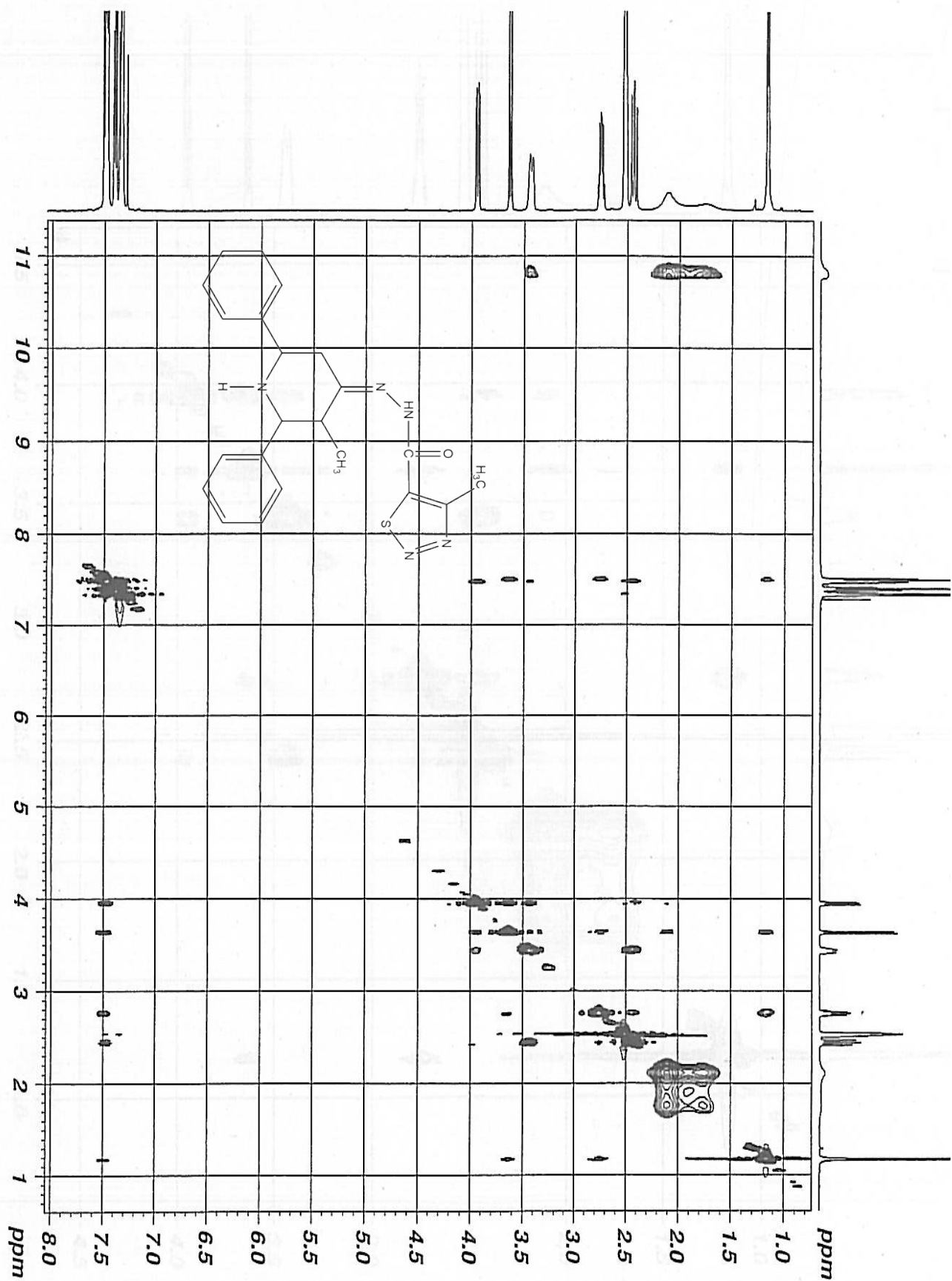
^1\text{H} - ^1\text{H} NOESY NMR Spectrum of 4-Methyl-N'-(3-methyl-2r,6c-diaryl)piperidin-4-ylidene)-1,2,3-thiadiazole-5-carbohydrazide (5a)
