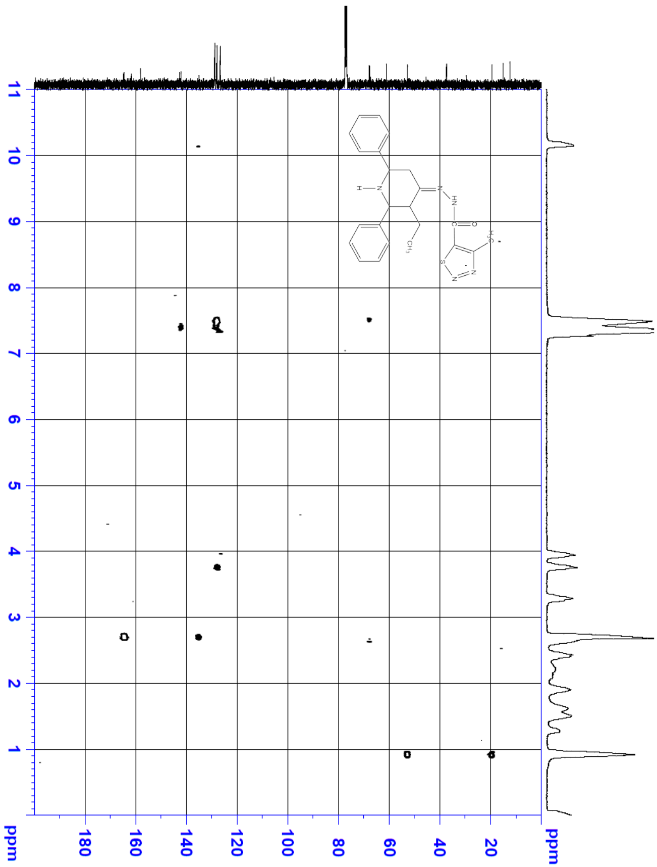
HMBC NMR Spectrum of 4-Methyl-N-(3-ethyl-2r,6c-diarylpiperidin-4-ylidene)-1,2,3-thiadiazole-5-carbonyldrazide (5g)
