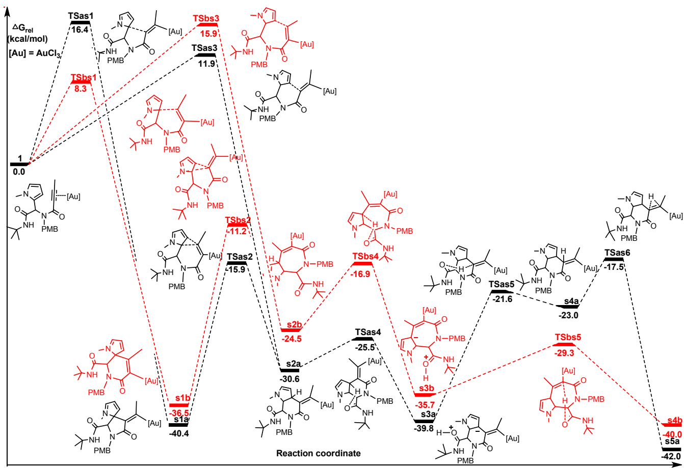
Figure S2 Energy profiles for AuCl 3 catalyzed; the relative energies are given in kcal/mol.
