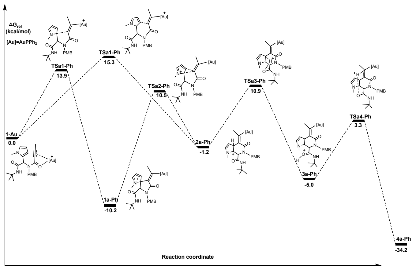
Figurer S1 Energy profiles for Au (PPh 3 ) catalyzed; the relative energies are given in kcal/mol.
