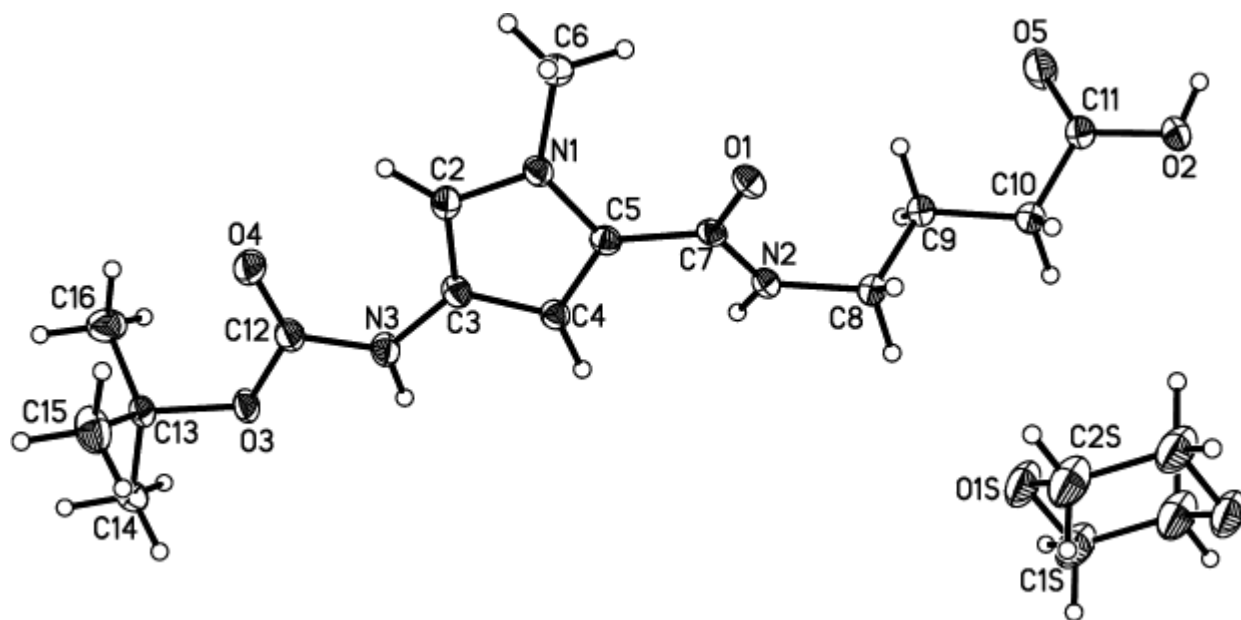
X-ray Figure 5. Projection view with 50% thermal ellipsoids for Boc-Py-β-COOH·0.5dioxane solvate.
