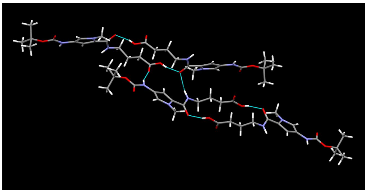
X-ray Figure 6. Intermolecular hydrogen bonding in the crystal structure of Boc-Py-β-COOH·0.5dioxane solvate.
