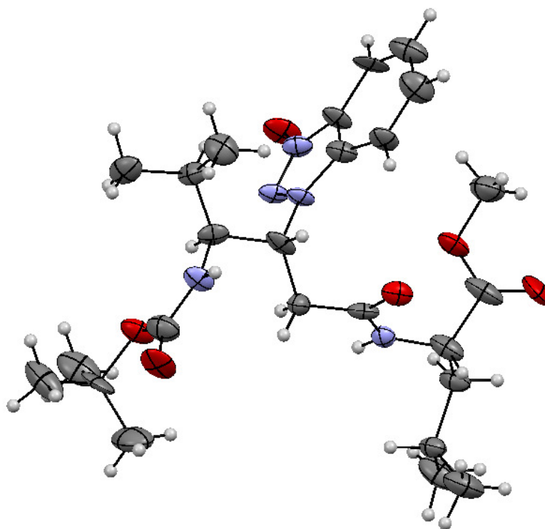
Figure S3: ORTEP diagram of Boc- \gamma L( \beta -OBt)-OMe – II ( 6c ).
