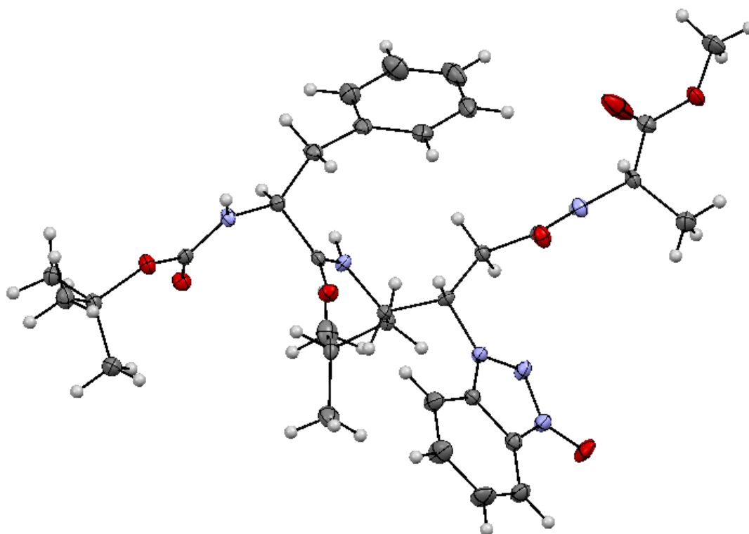
Figure S5: ORTEP diagram of Boc-F- \gamma L( \beta -OBt)-A-OMe ( 13 ).
