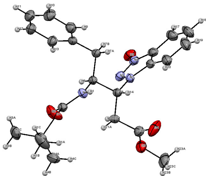
Figure S2: ORTEP diagram of Boc- \gamma F( \beta -OBt)-OMe – II ( 6a ).
