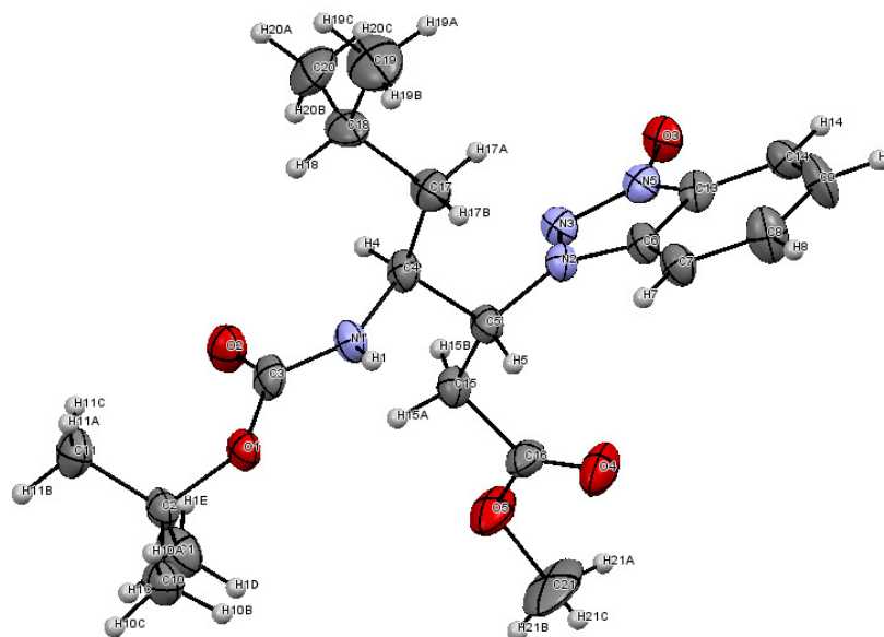
Figure S3: ORTEP diagram of Boc- \gamma L( \beta -OBt)-OMe – II ( 6c ).
