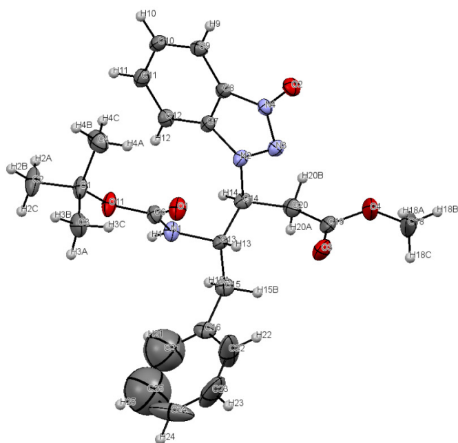
Figure S1: ORTEP diagram of Boc- \gamma F( \beta -OBt)-OMe – I ( 7a ).
