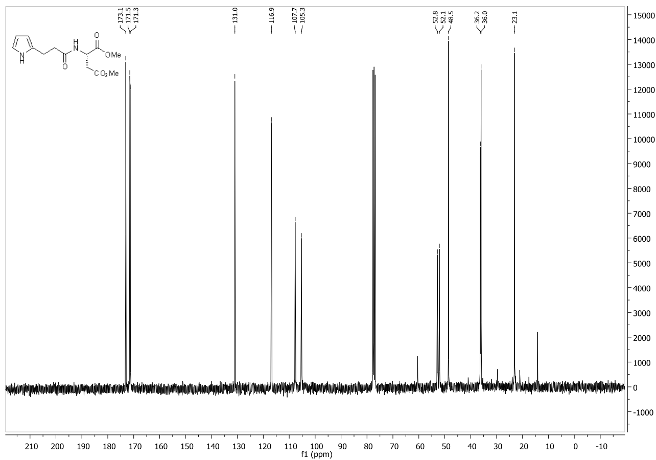
Compound 13b :
