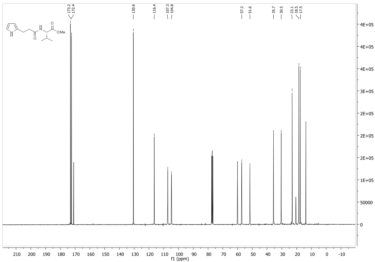
Compound 11b :
