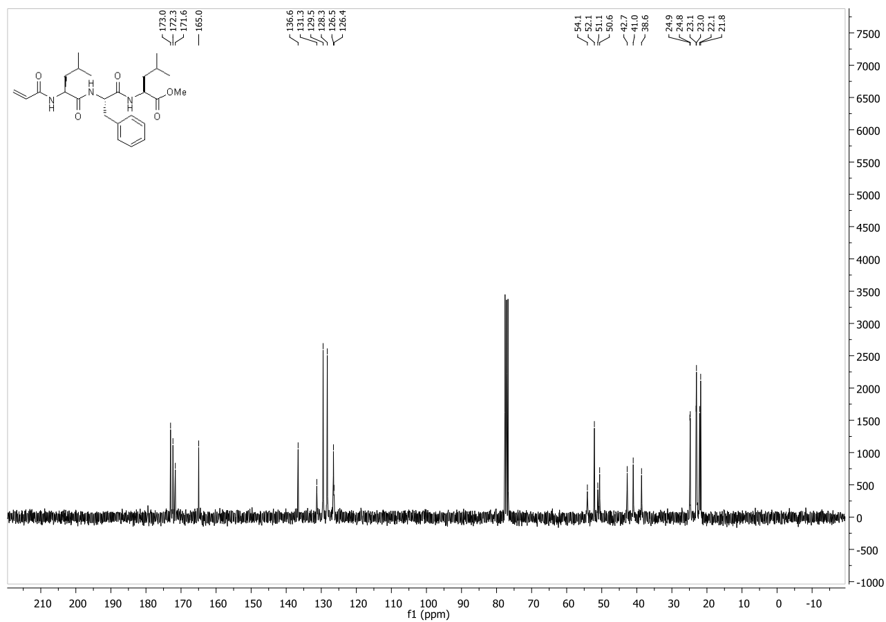
Compound 3a :
