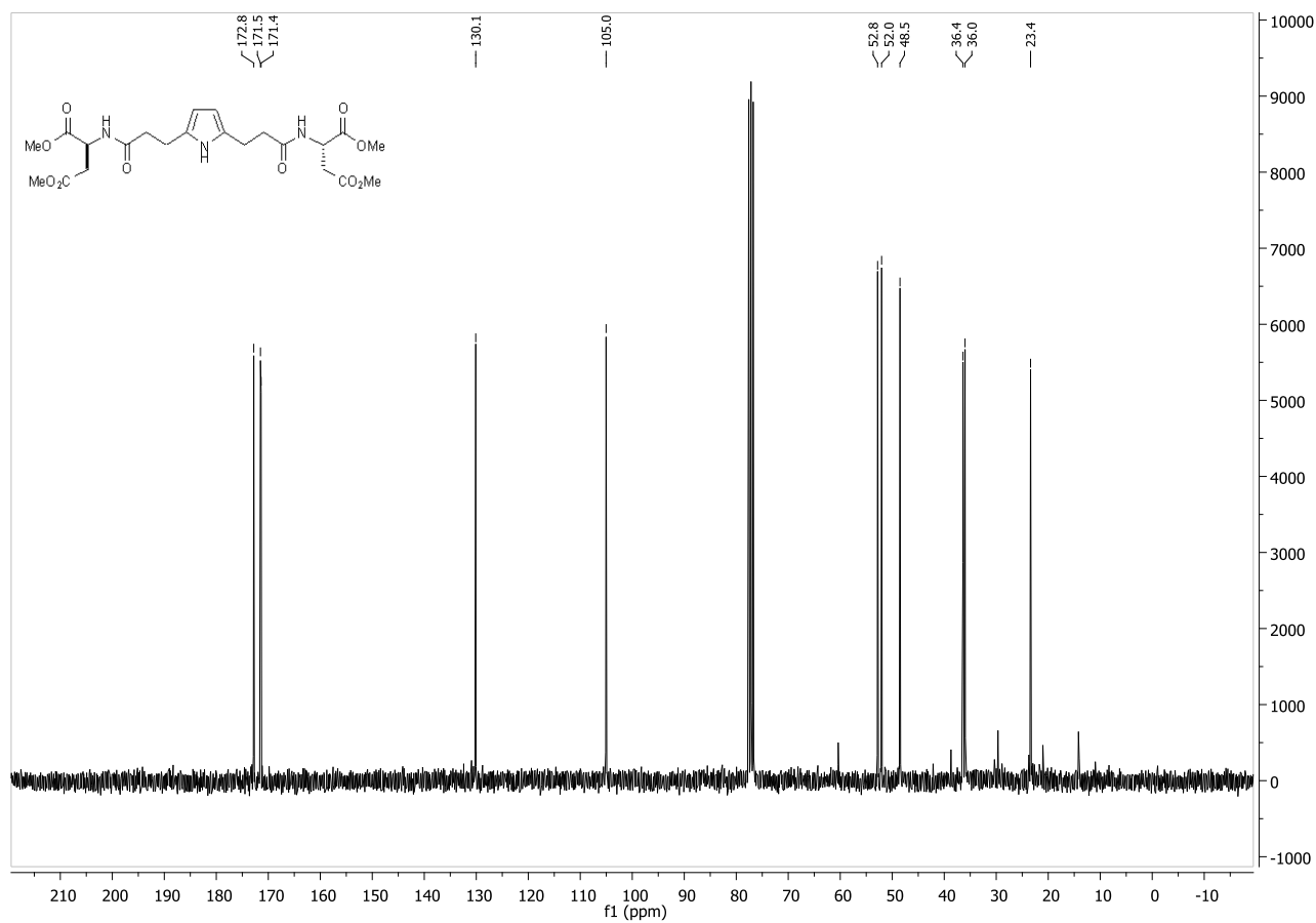
Compound 14a :
