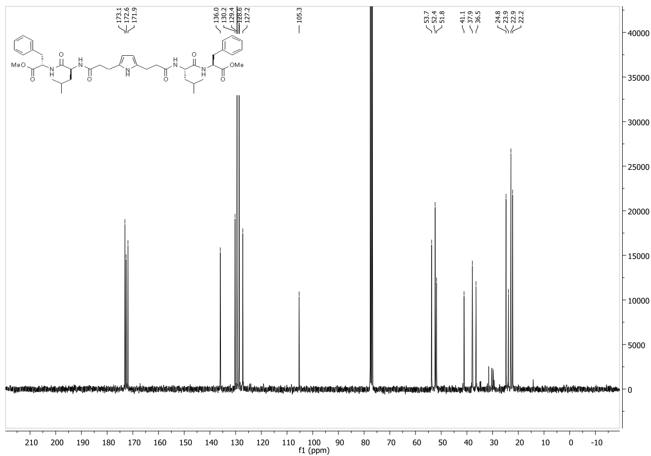
Compound 19a :
