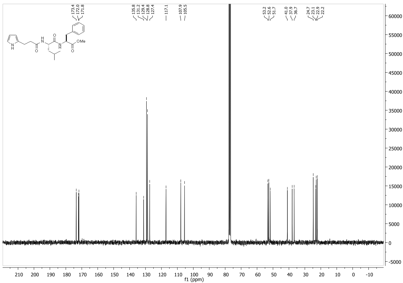
Compound 18b :
