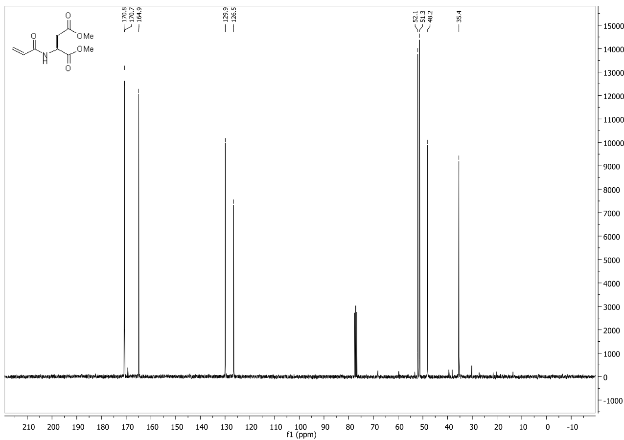
Compound 8 :
