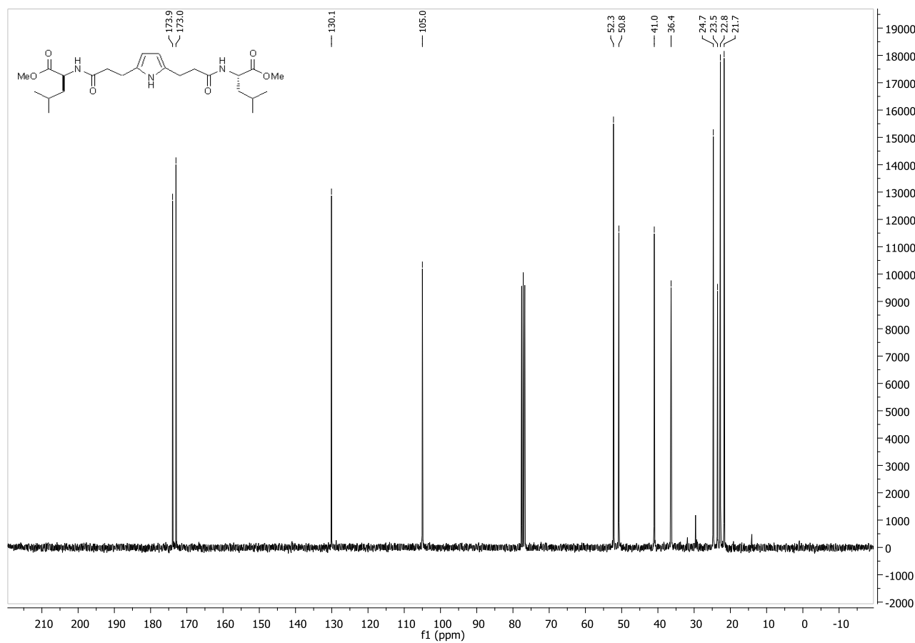
Compound 13a :
