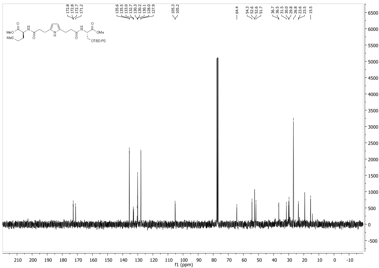
Compound 23 :
