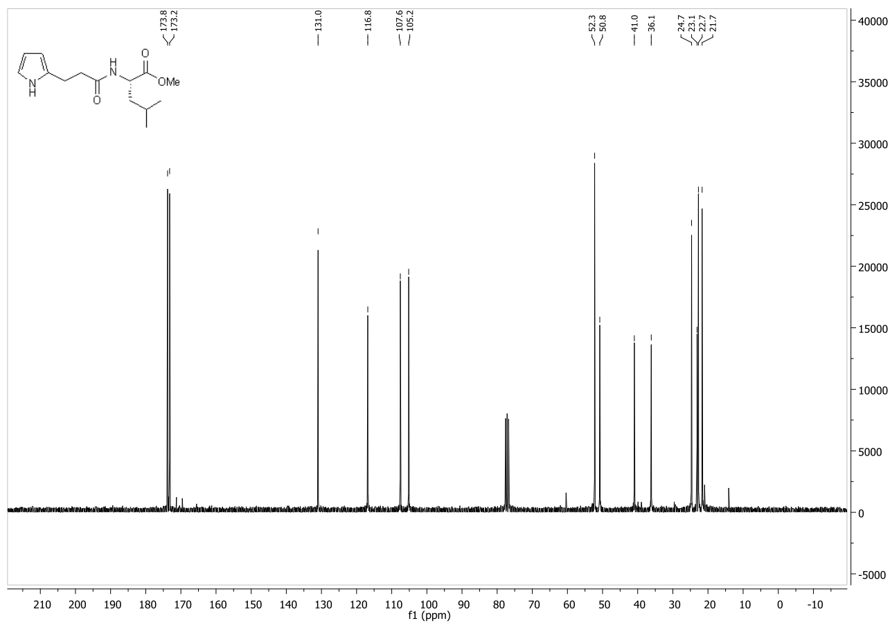
Compound 12b :
