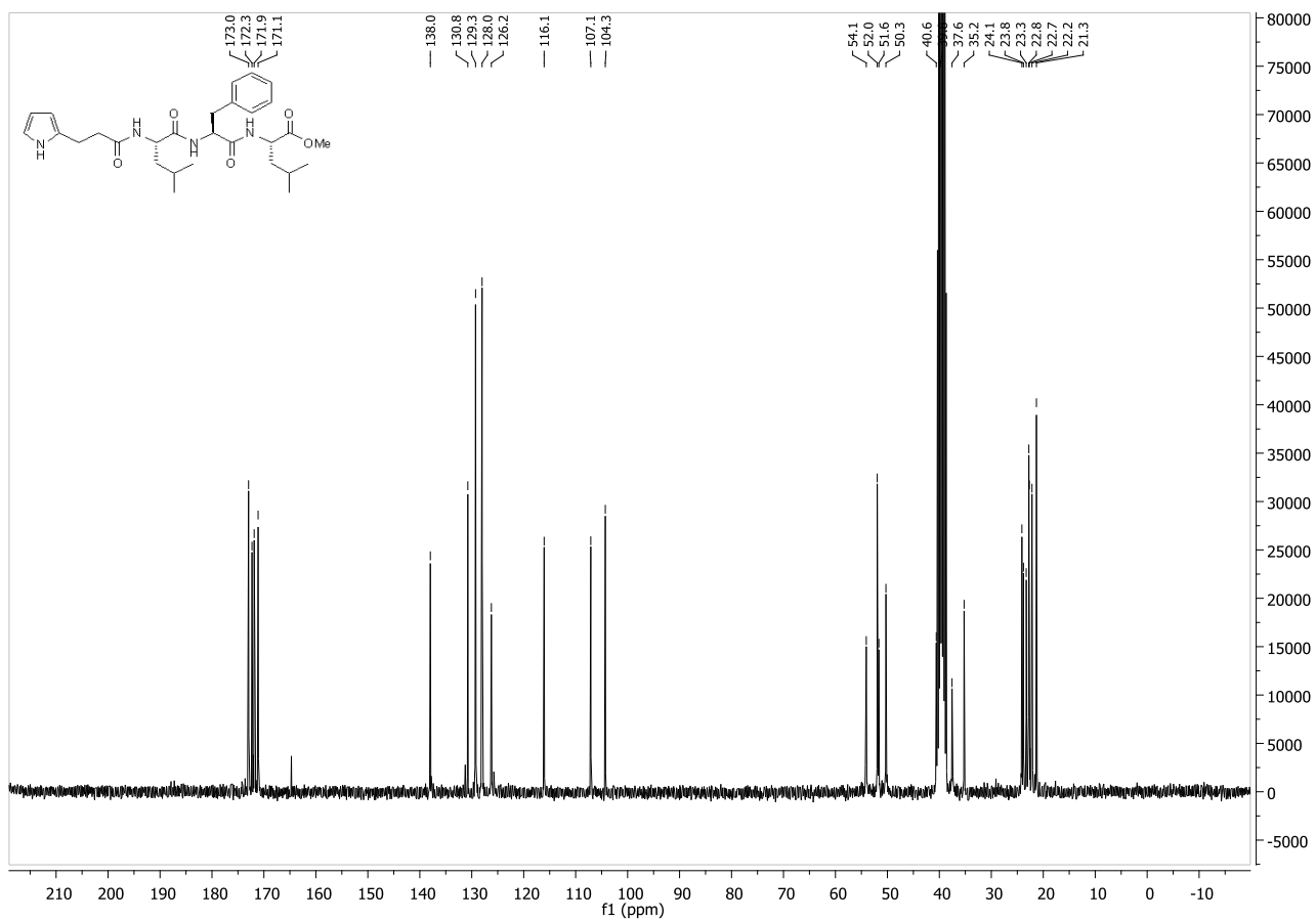
Compound 19b :
