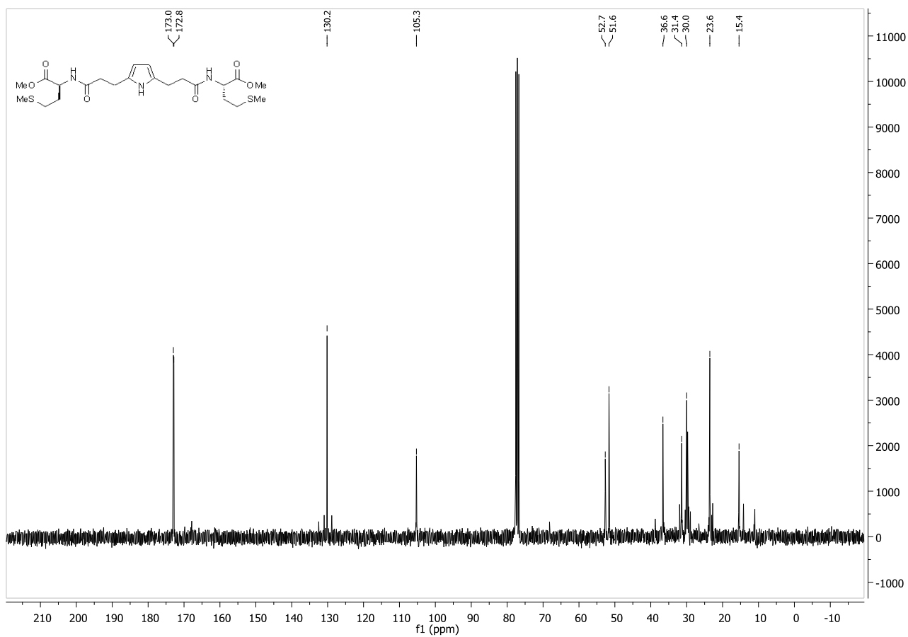
Compound 18a :
