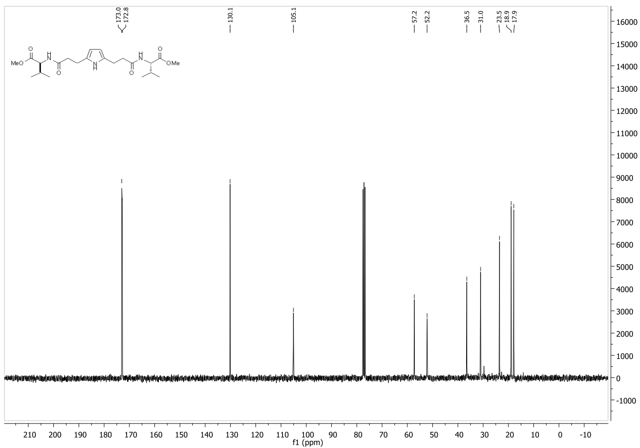
Compound 12a :
