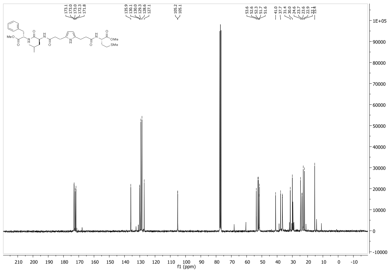
Compound 24 :
