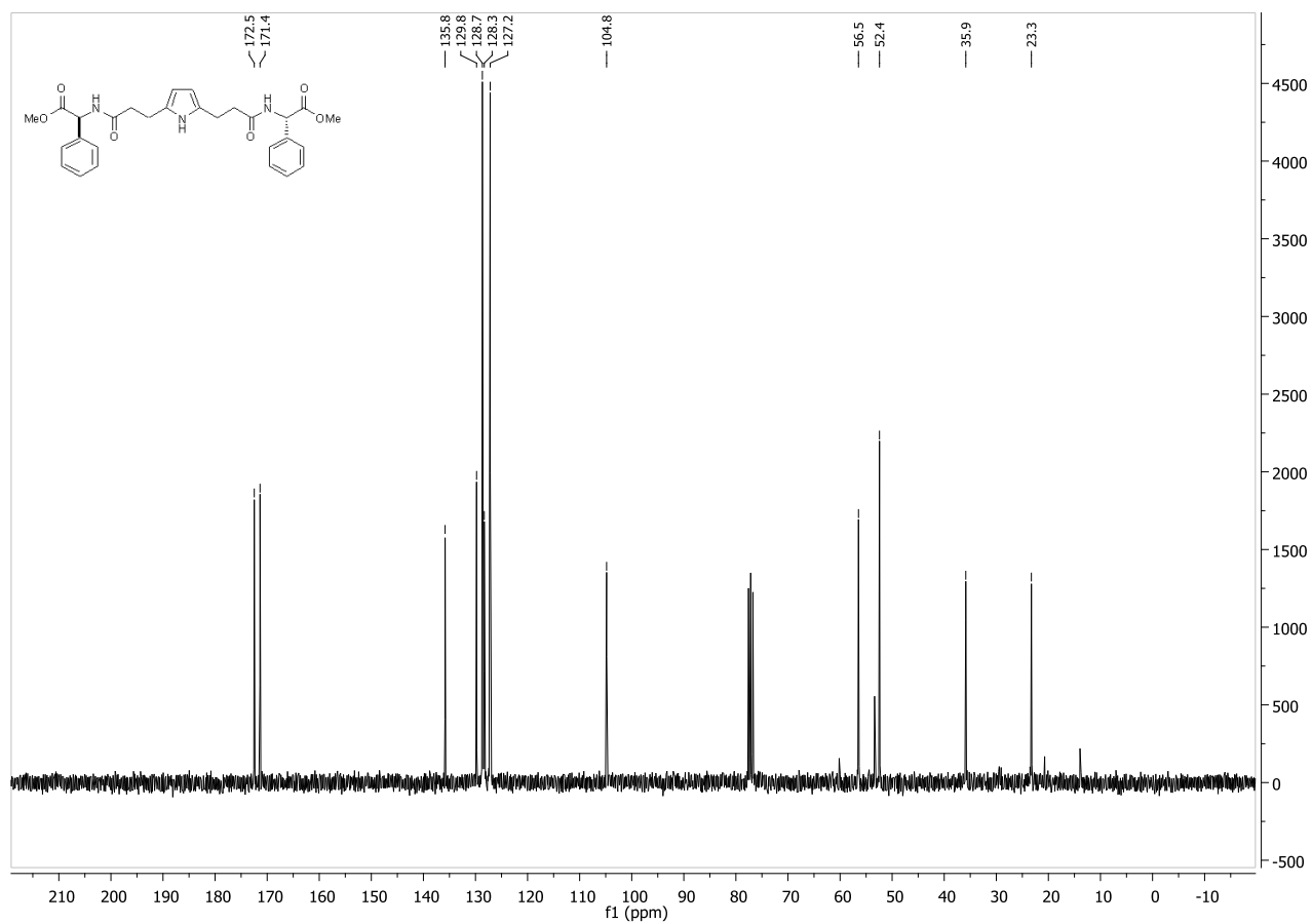
Compound 11a :
