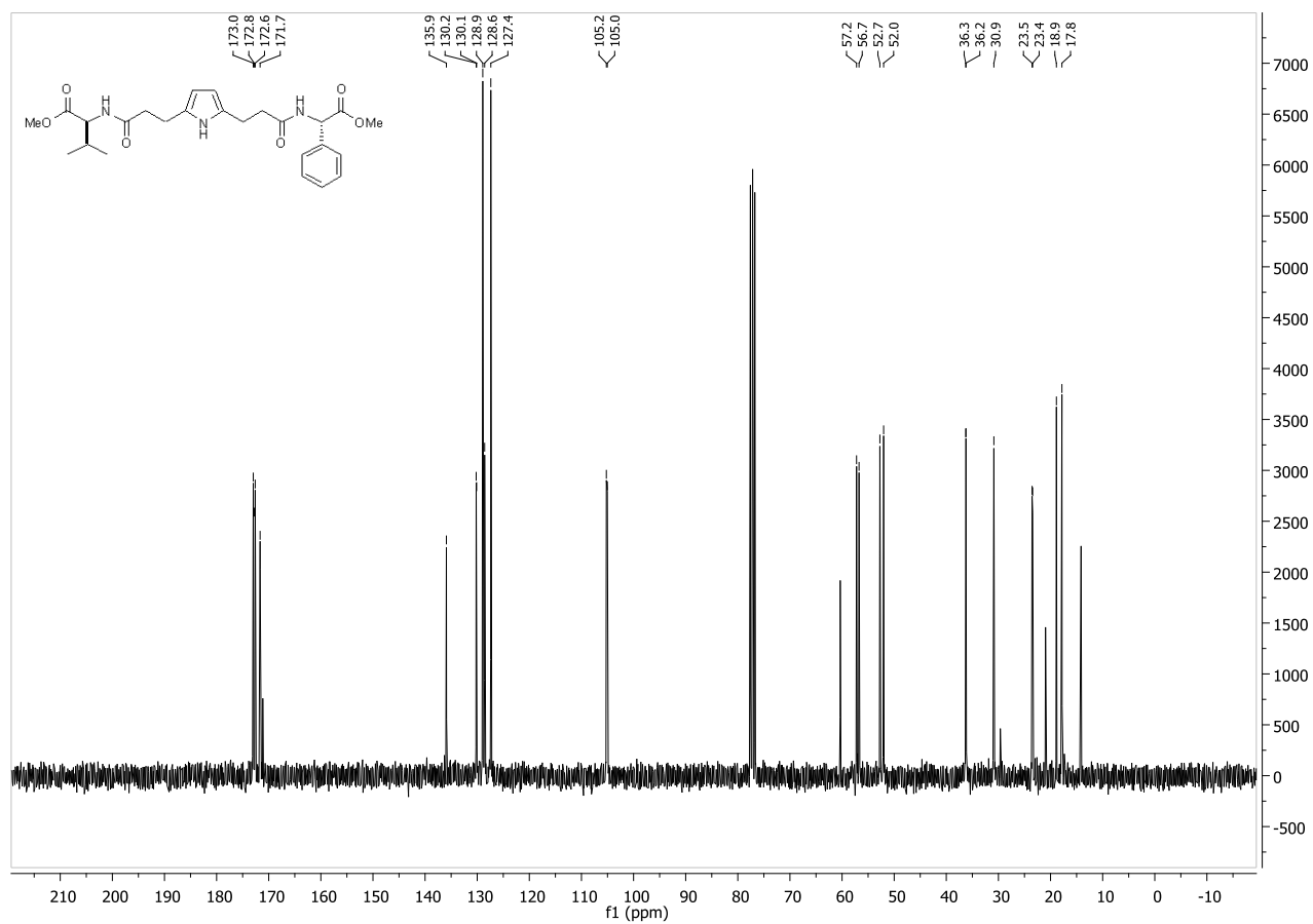
Compound 22 :
