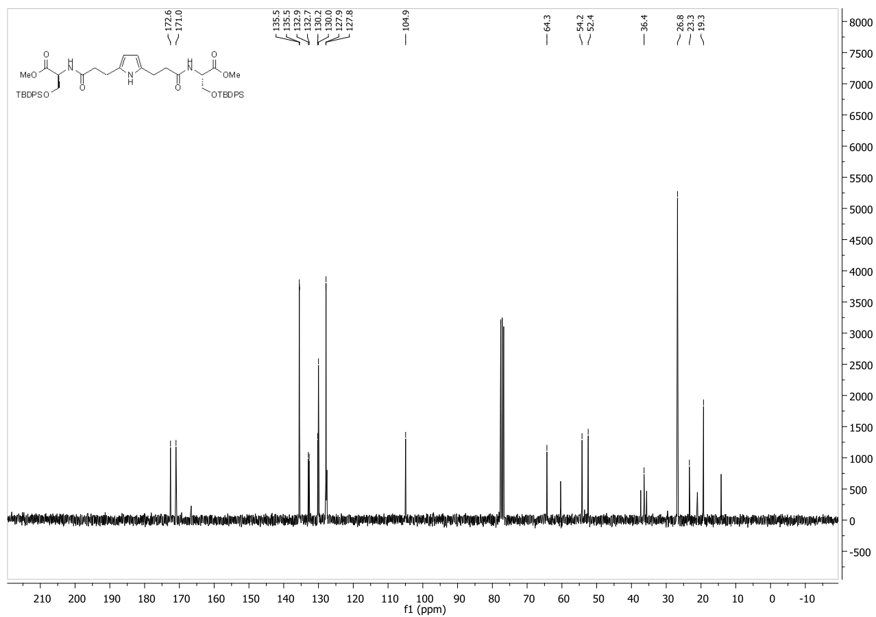
Compound 15a :
