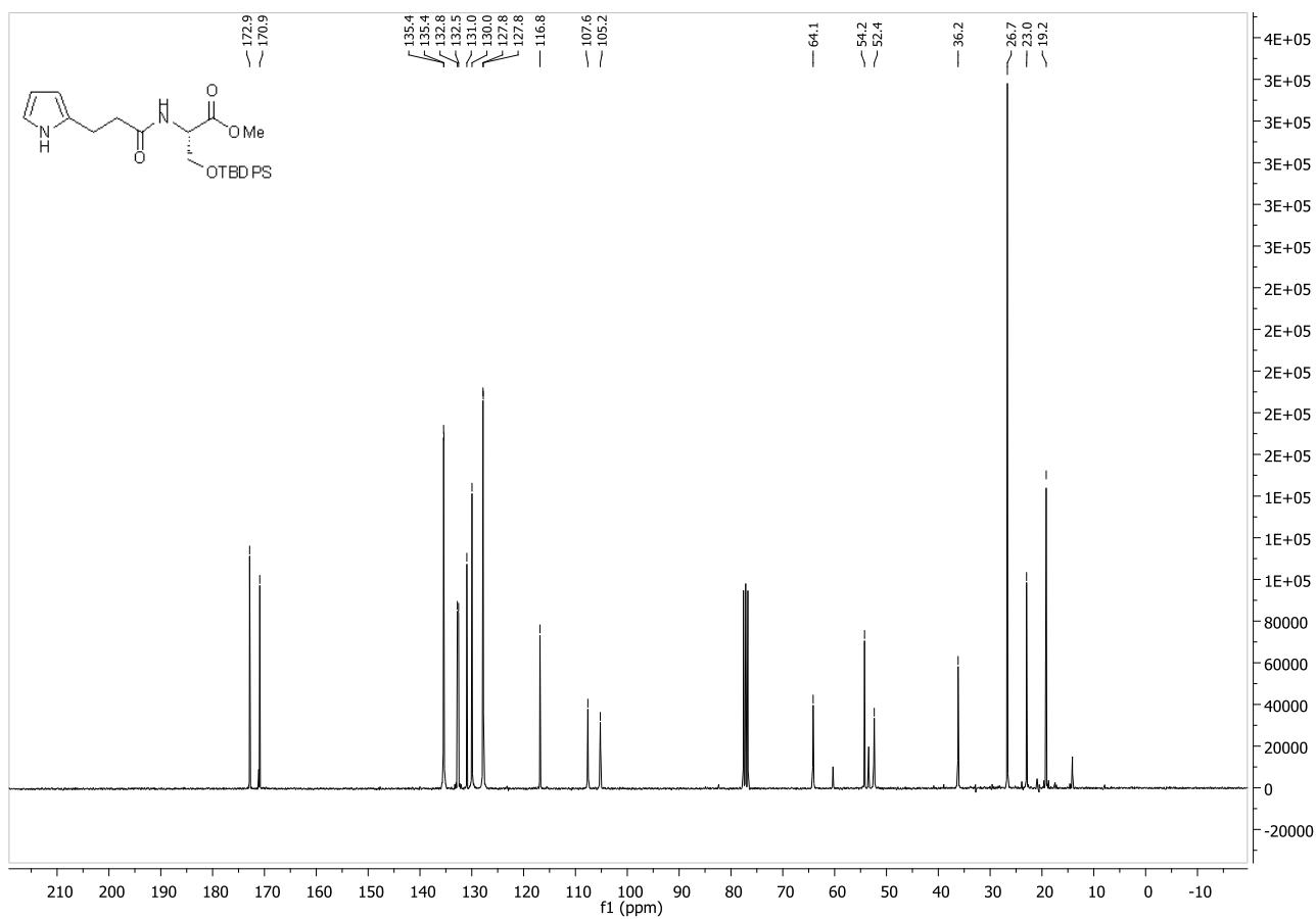
Compound 14b :
