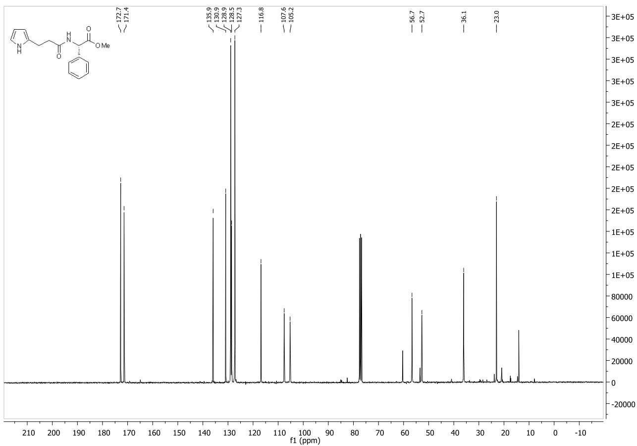
Compound 10b :
