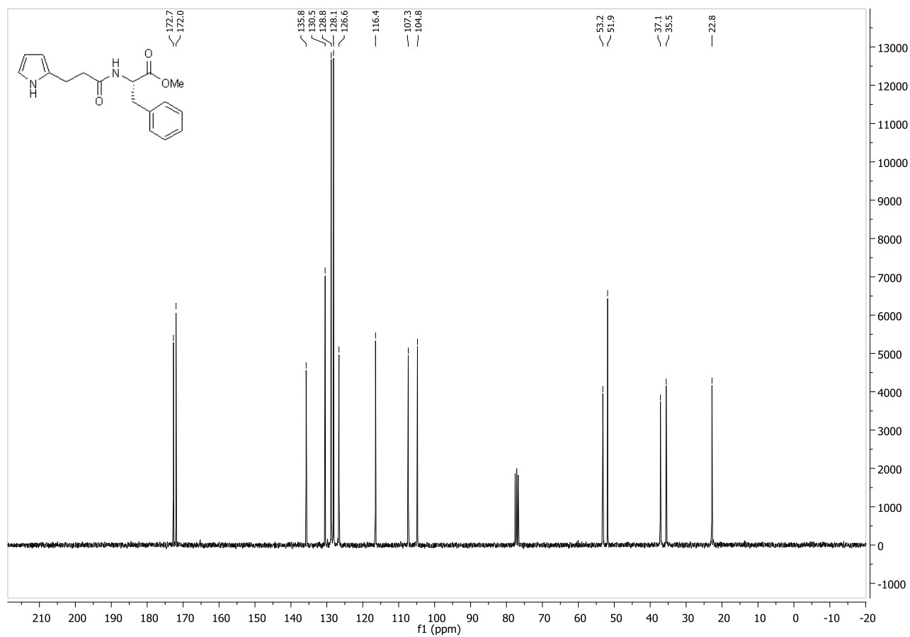
Compound 3b :
