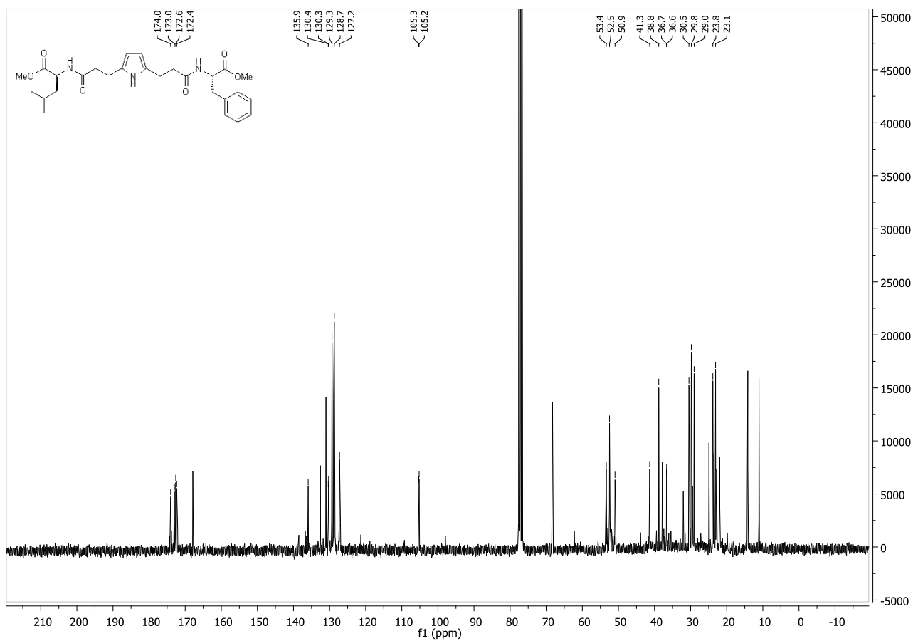
Compound 21 :
