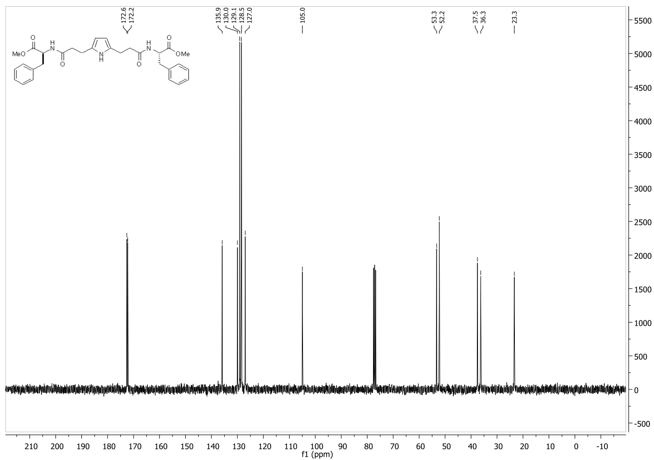
Compound 10a :
