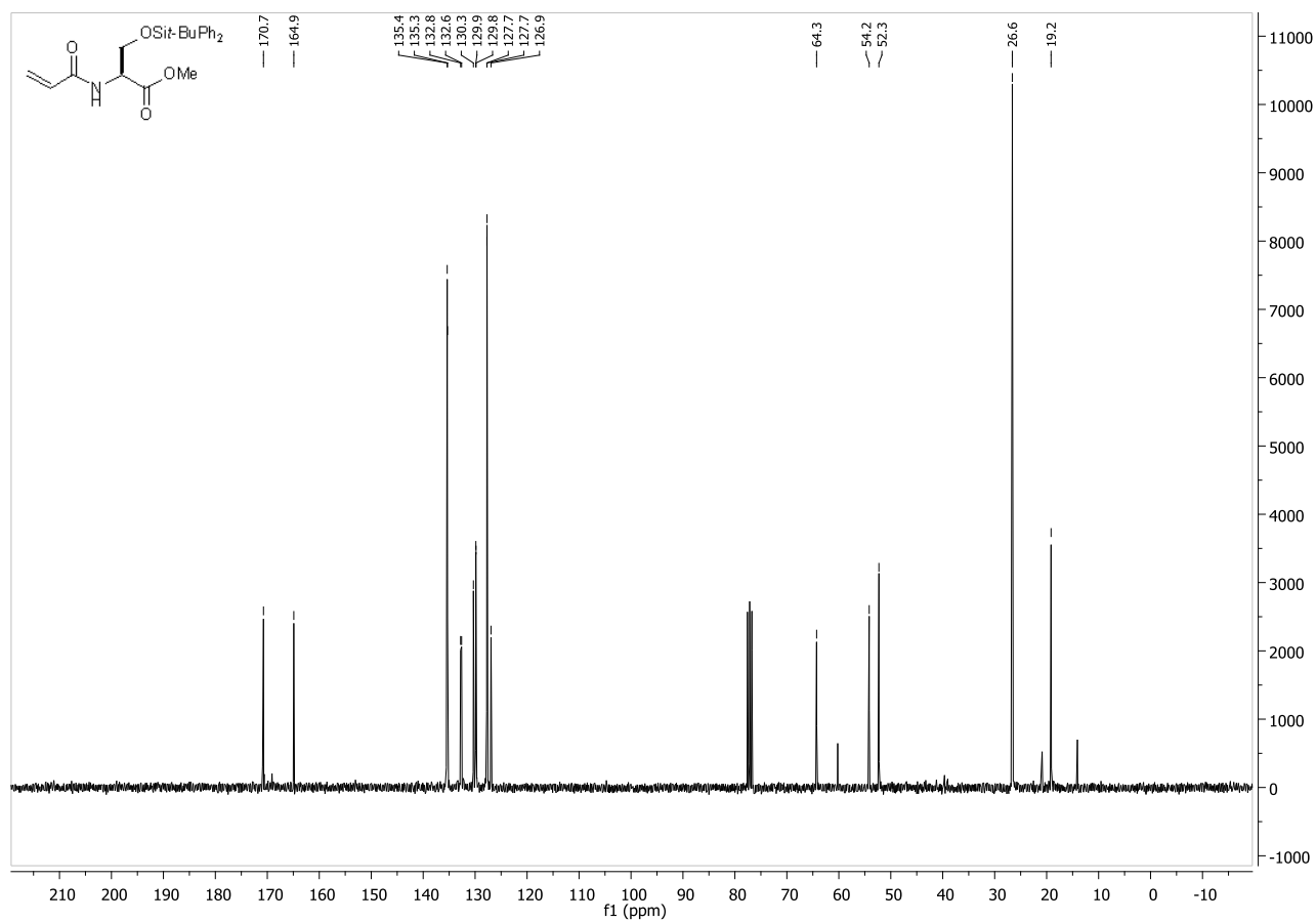
Compound 17 :
