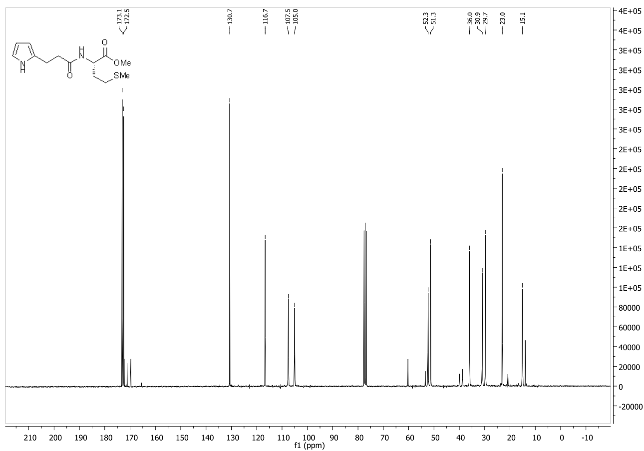
Compound 15b :
