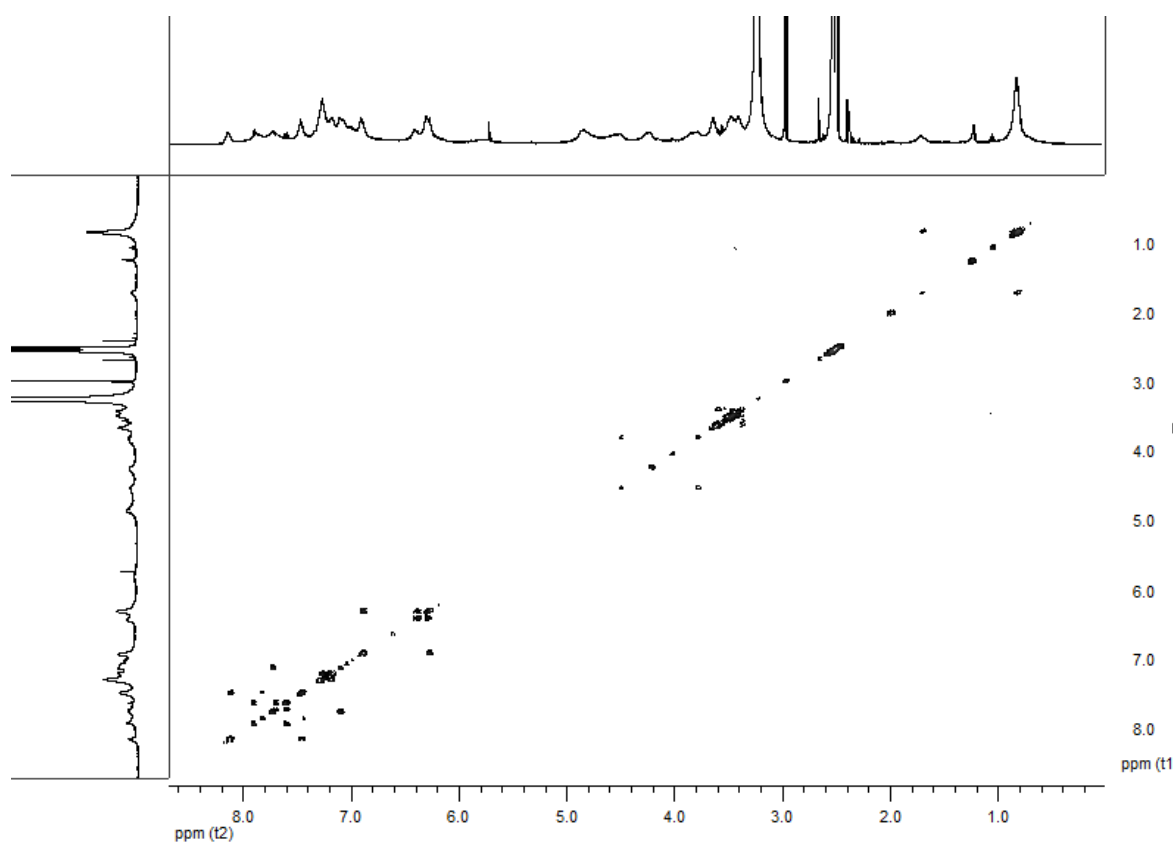
^1\text{H} - ^1\text{H} COSY Spectra of Compound 2 in \text{DMSO-d}_6
