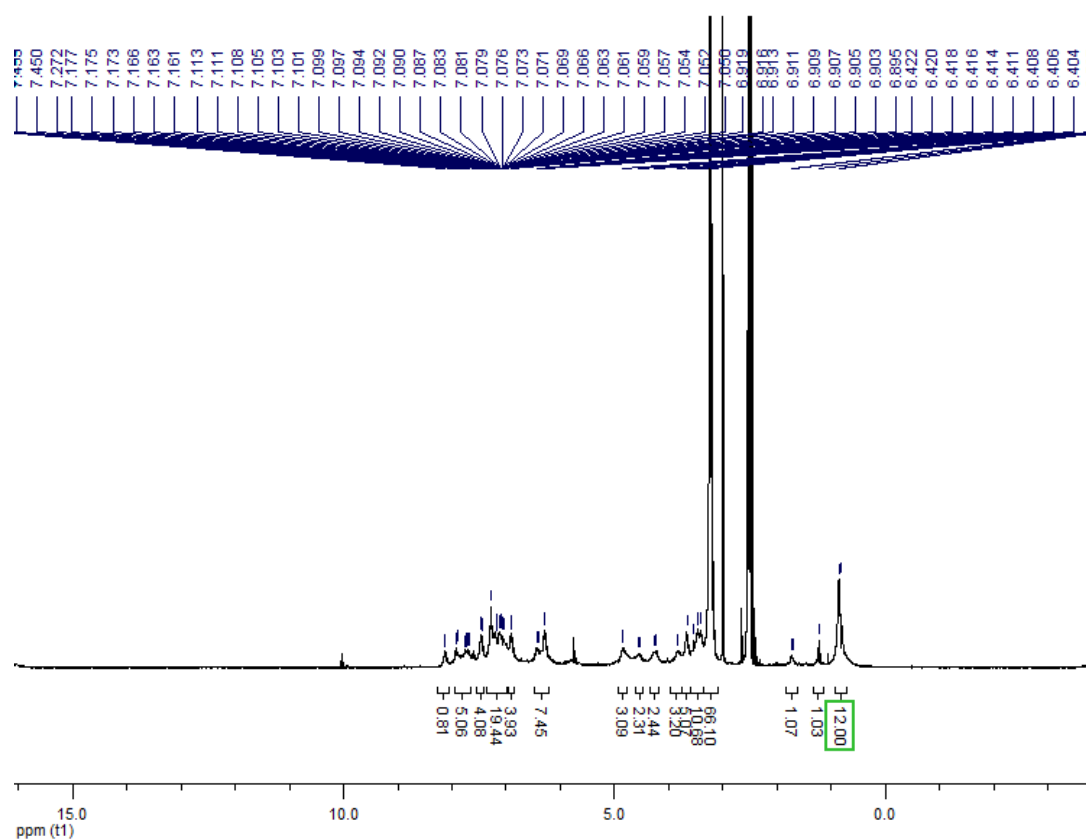
^1\text{H} NMR Spectra of Compound 2 in \text{DMSO-d}_6
