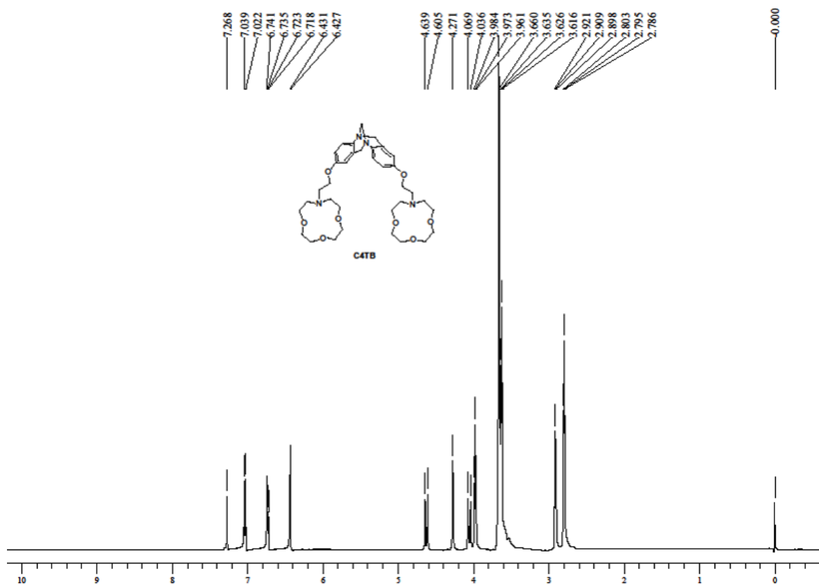
1 H NMR spectra of C4TB in CDCl 3
