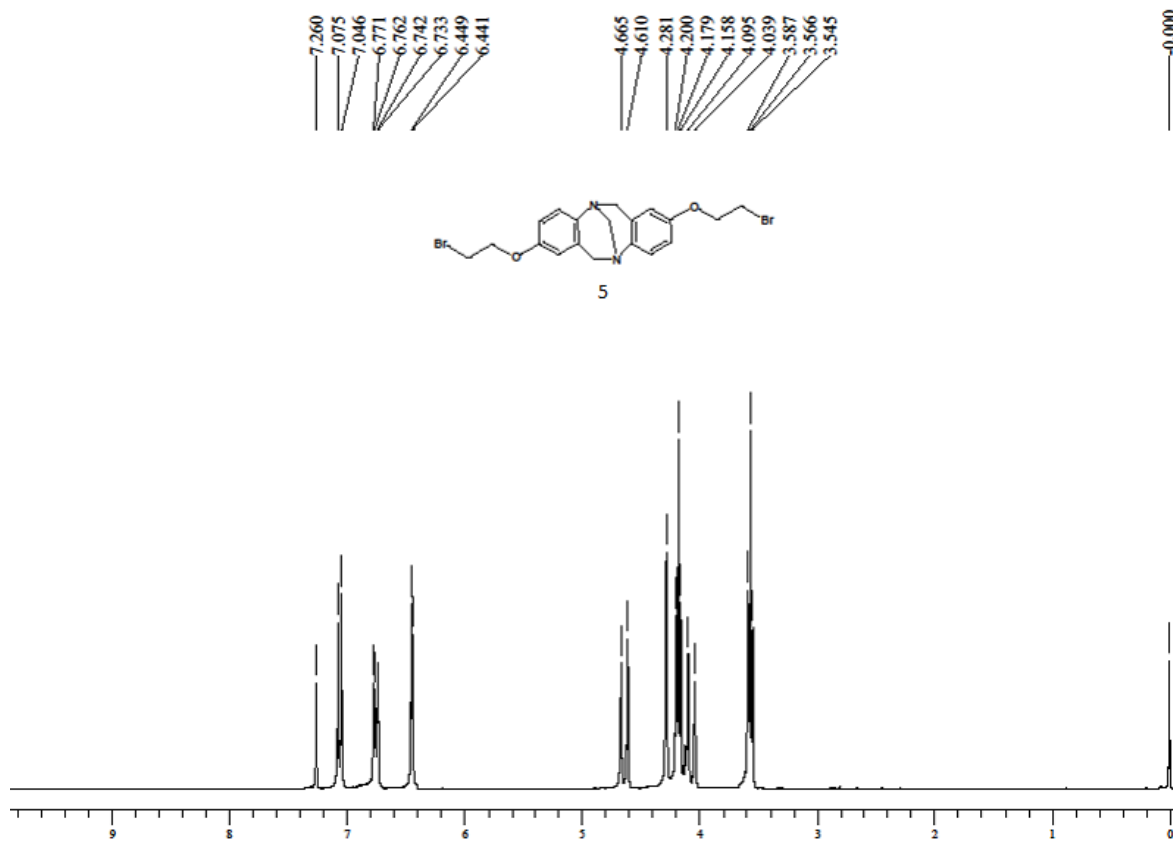
1 H NMR spectra of 5 in CDCl 3
