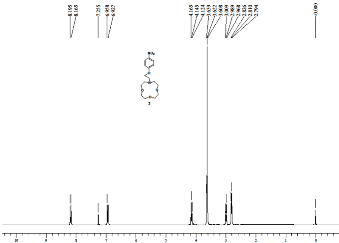
1 H NMR spectra of 2 in CDCl 3
