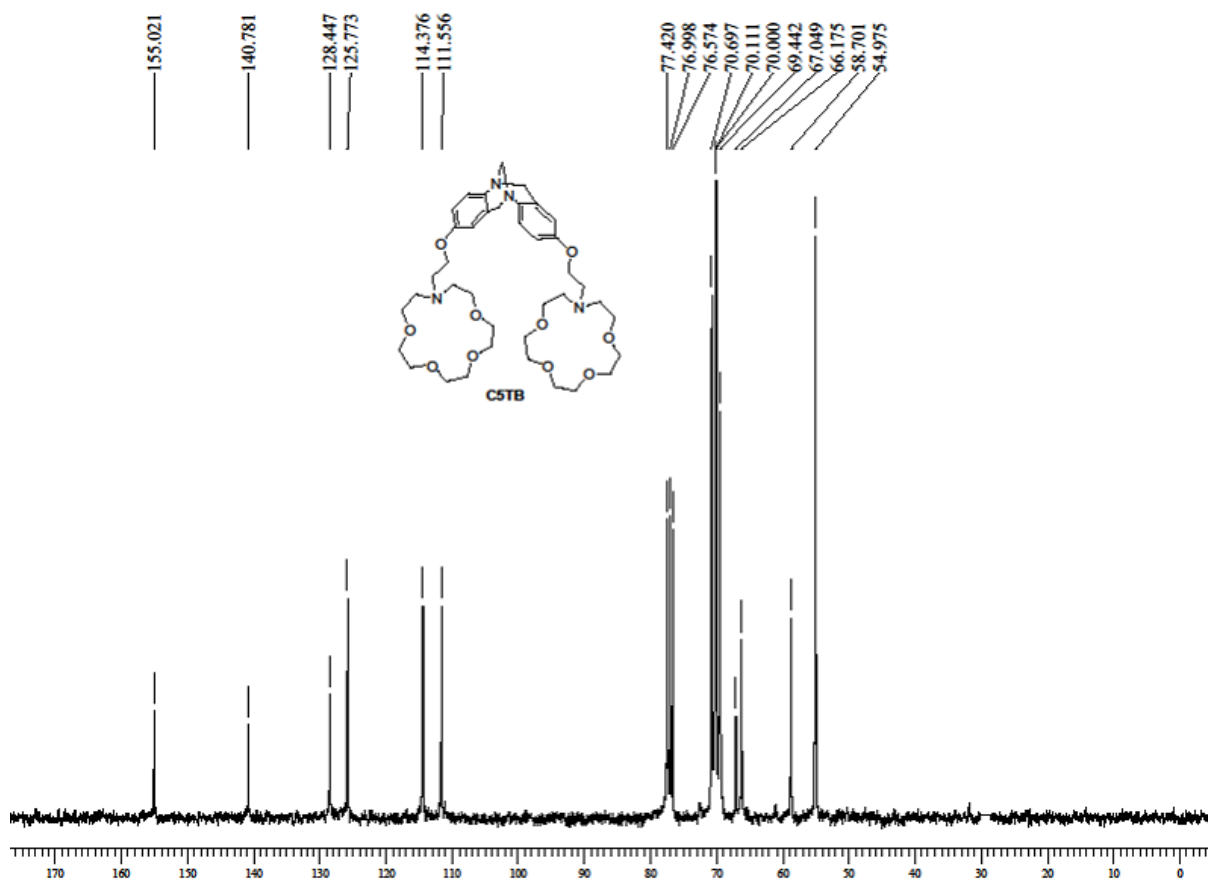
^{13}\text{C} NMR spectra of C5TB in \text{CDCl}_3
