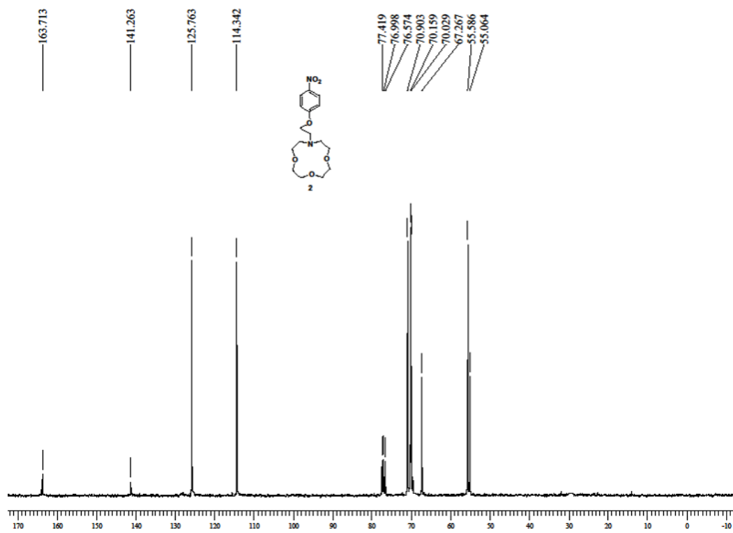
13 C NMR spectra of 2 in CDCl 3
