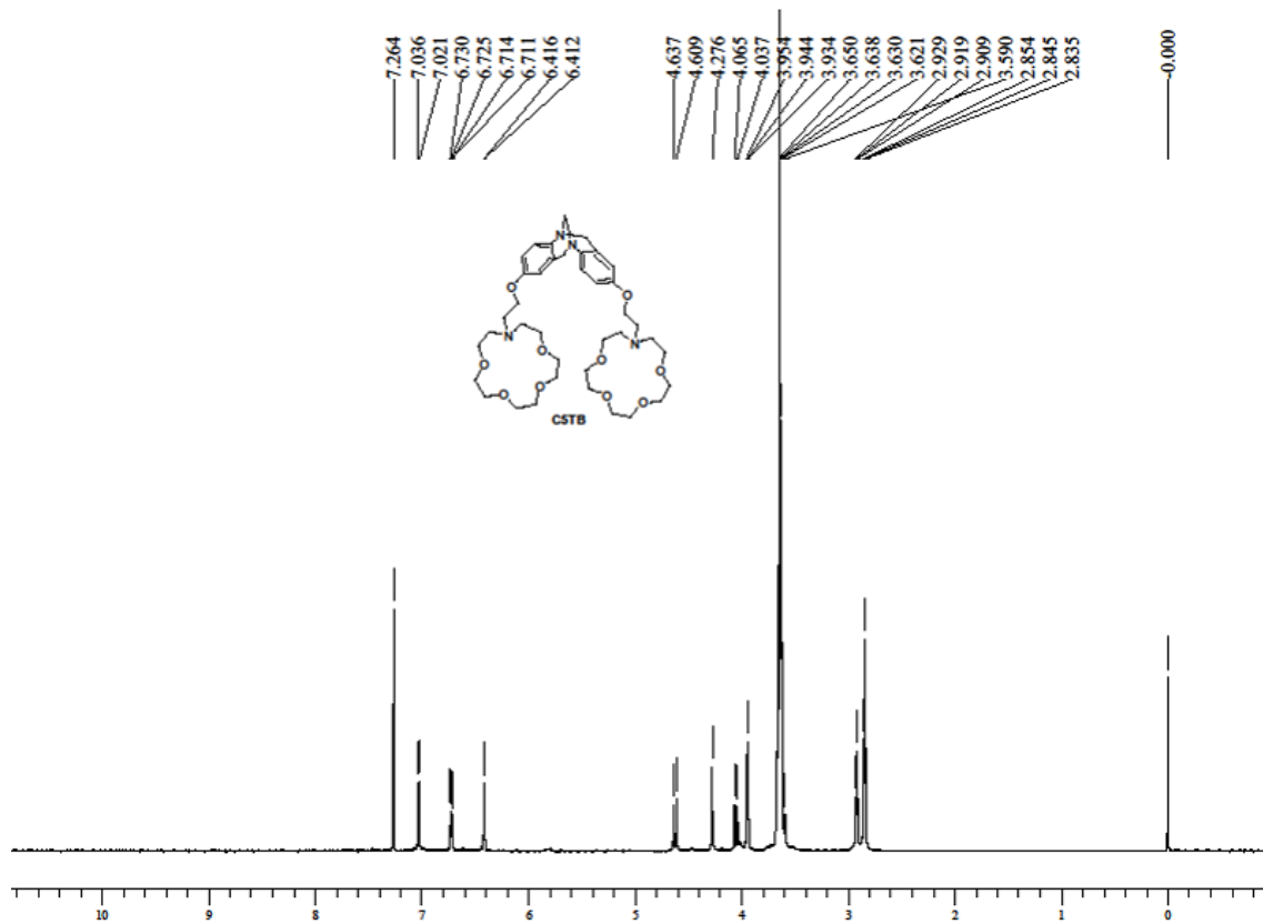
^1\text{H} NMR spectra of C5TB in \text{CDCl}_3
