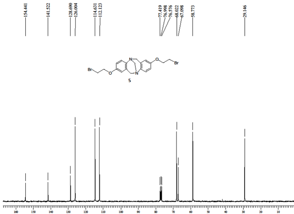
13 C NMR spectra of 5 in CDCl 3
