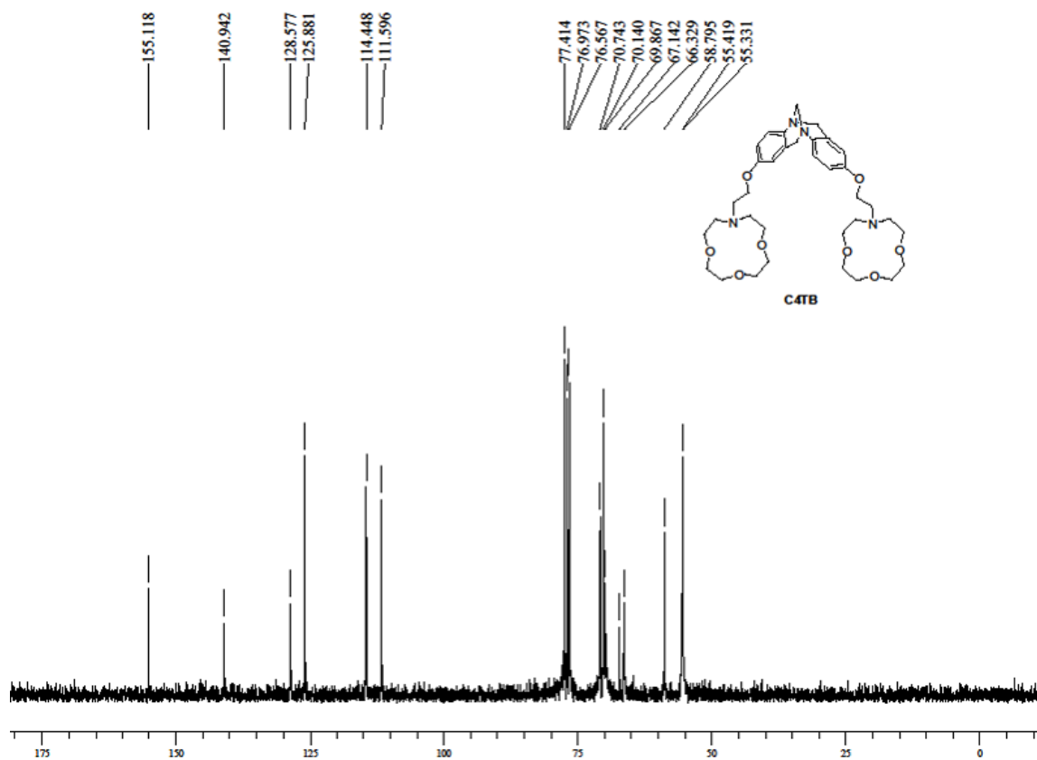
13 C NMR spectra of C4TB in CDCl 3
