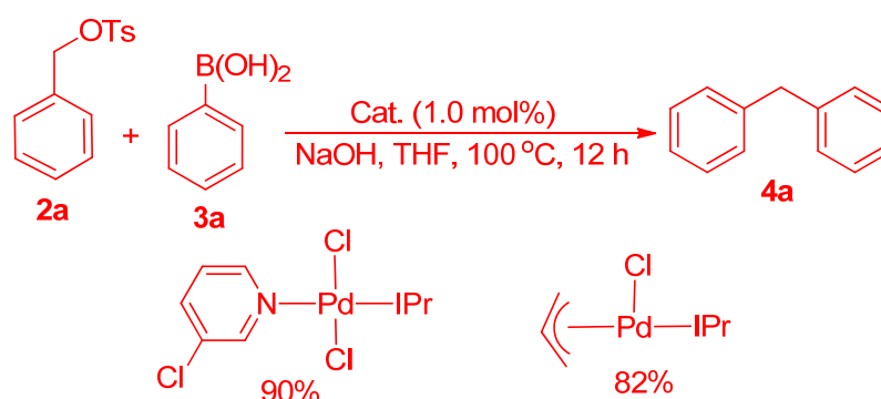
Scheme-SI. Catalytic activity of other NHC-Pd(II) complexes in model reaction under the optimal conditions.
