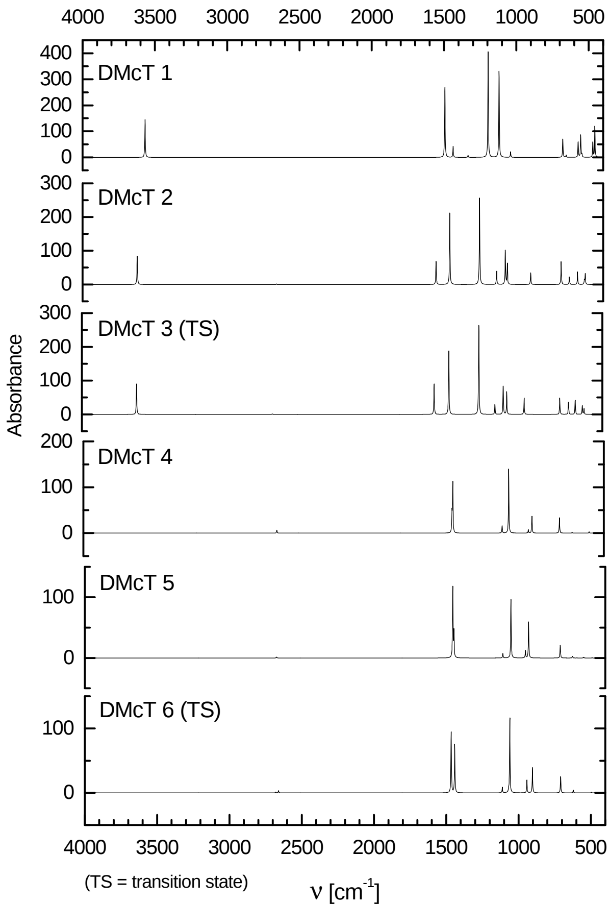
Theoretical IR spectra for all DMcT isomers calculated at B3LYP/6-311+G(d,p) level, unscaled.
