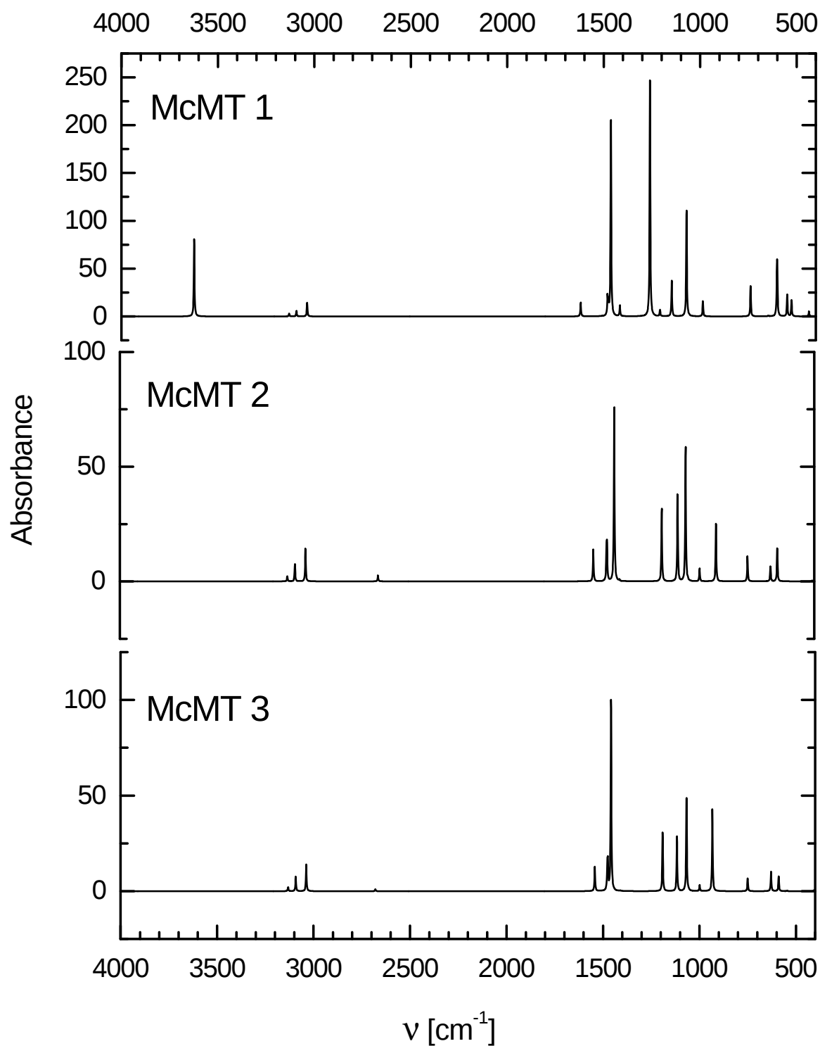
Theoretical IR spectra for all McMT isomers calculated at B3LYP/6-311+G(d,p) level, unscaled.
