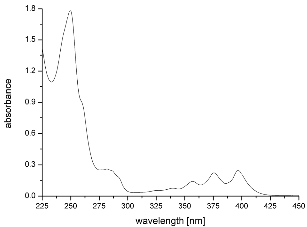
Fig. S2 UV/VIS spectrum of 2 in cyclohexane ( 1.15 \times 10^{-5} mol/L).
