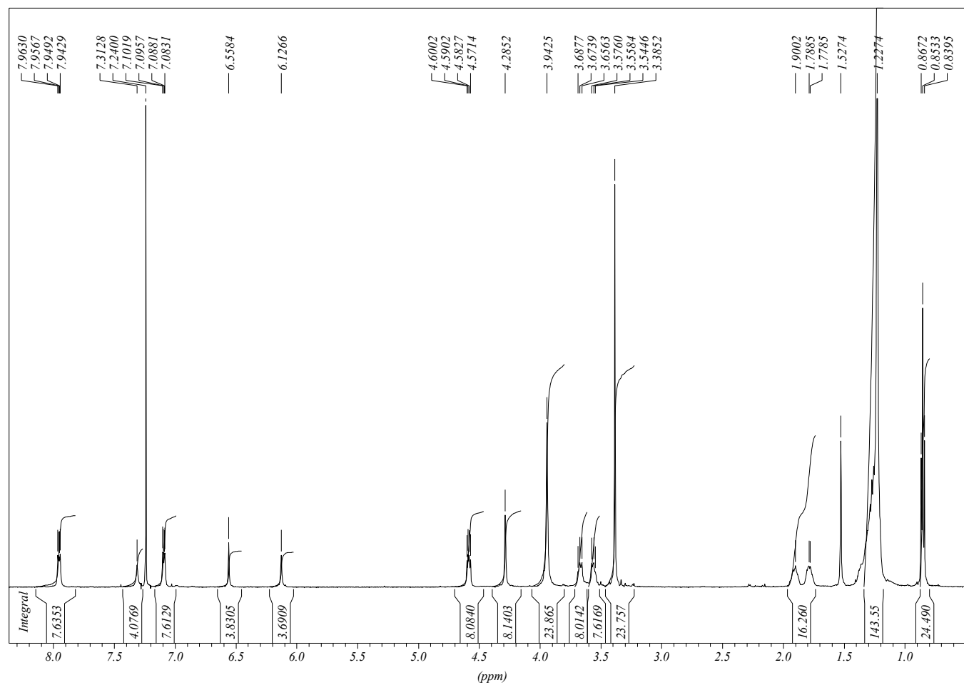
Fig. S3 500 MHz 1 H NMR spectrum of 1 in CDCl 3 (7.24 ppm).
