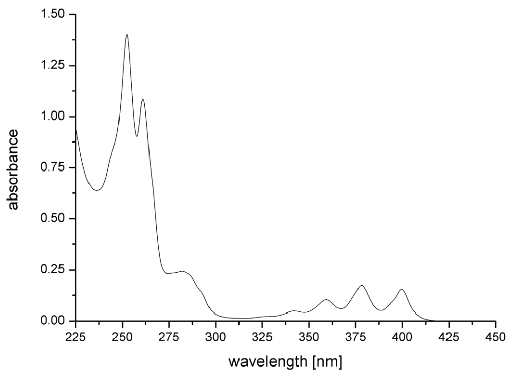
Fig. S1 UV/VIS spectrum of 1 in cyclohexane ( 1.04 \times 10^{-5} mol/L).
