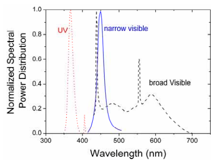
Fig. S1. Emission spectra of the three light sources used in this work, as obtained by their market datasheets. a) UV black-light blue lamps, b) visible fluorescent lamps with 430 cut-off filter and c) royal blue LEDs.
