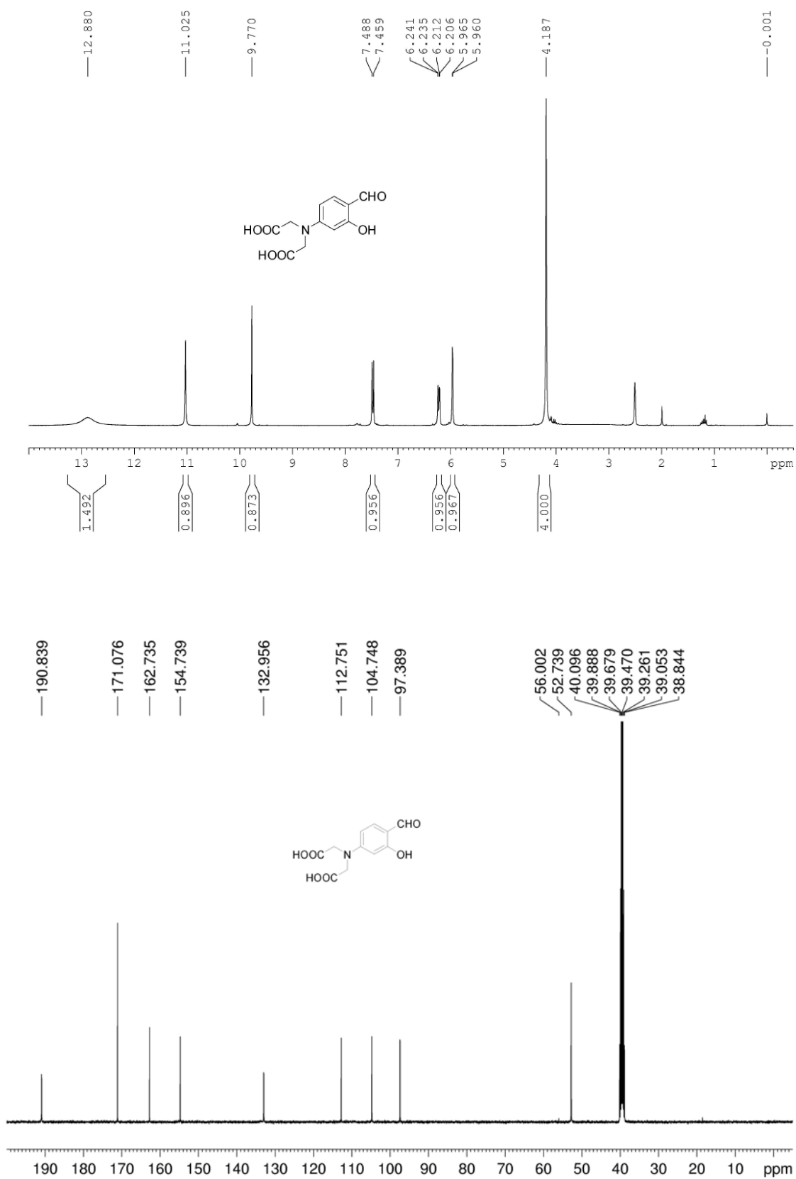
Figure S4. ^1\text{H} NMR and ^{13}\text{C} NMR spectra of 6
