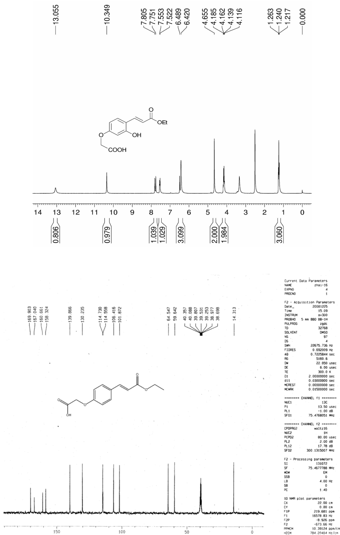
Figure S6. ^1\text{H} NMR and ^{13}\text{C} NMR spectra of 1a
