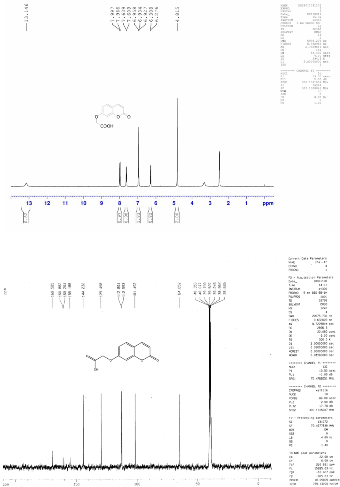
Figure S7. 1 H NMR and 13 C NMR spectra of 2a
