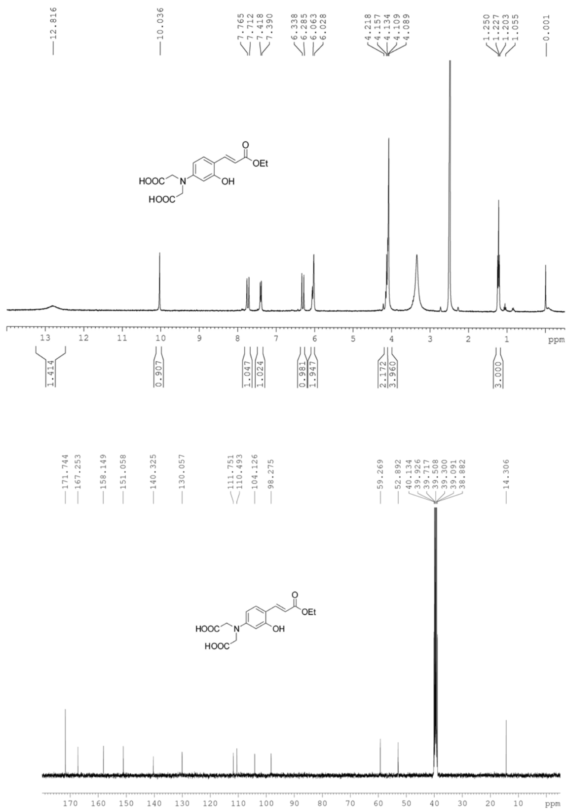
Figure S8. ^1\text{H} NMR and ^{13}\text{C} NMR spectra of 1b
