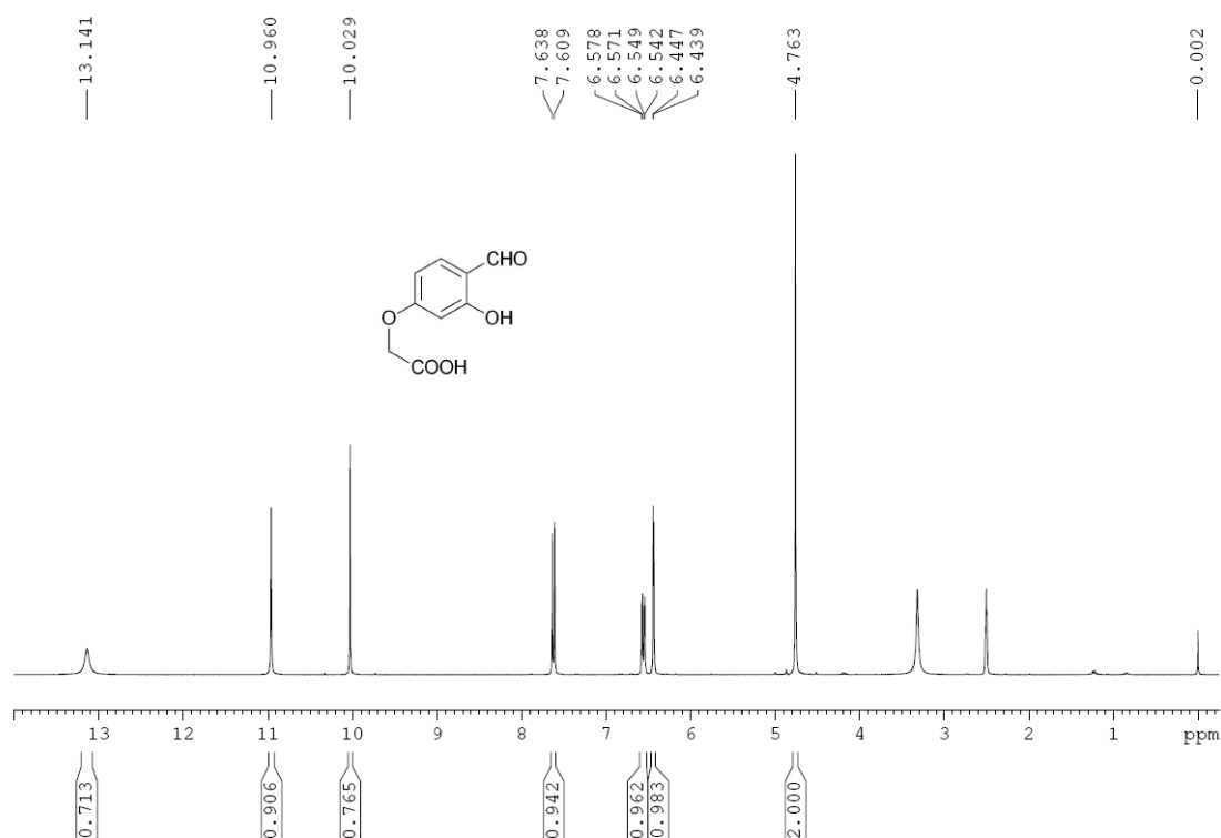
Figure S1. ^1\text{H} NMR spectra of 3
