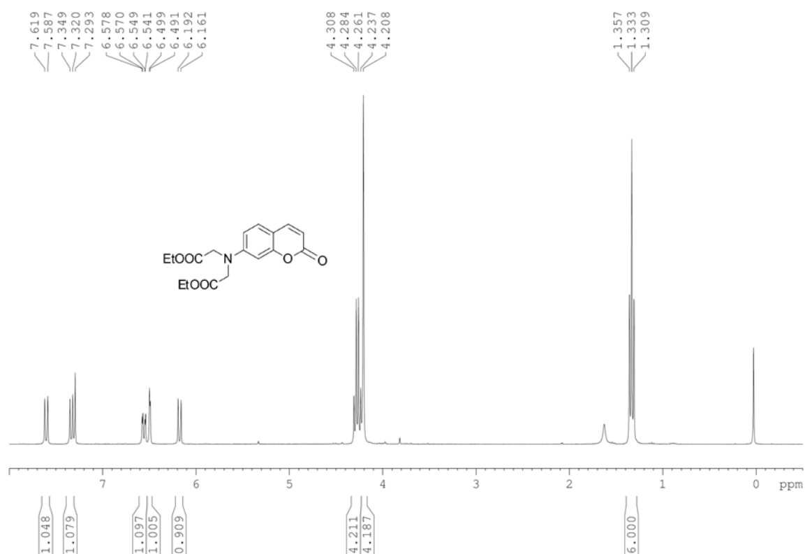
Figure S5. ^1\text{H} NMR spectra of 8
