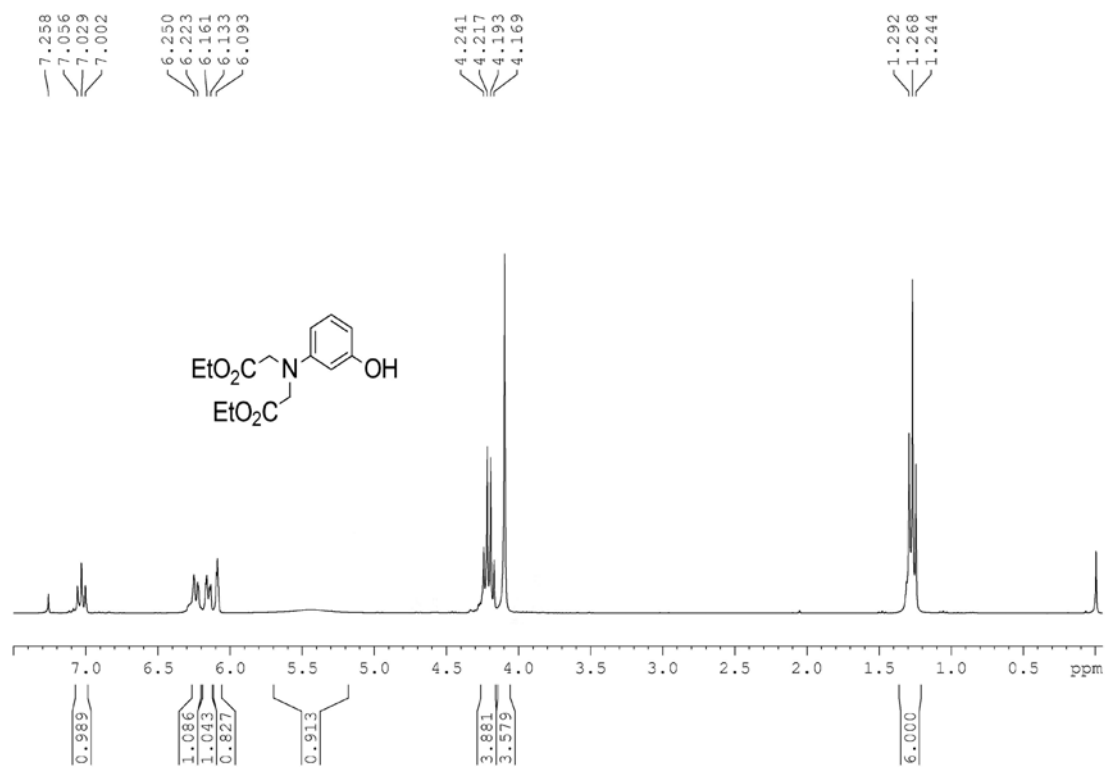
Figure S2. ^1\text{H} NMR spectra of 4
