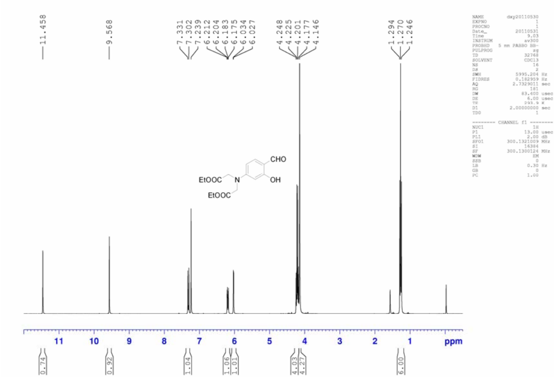
Figure S3. 1 H NMR spectra of 5
