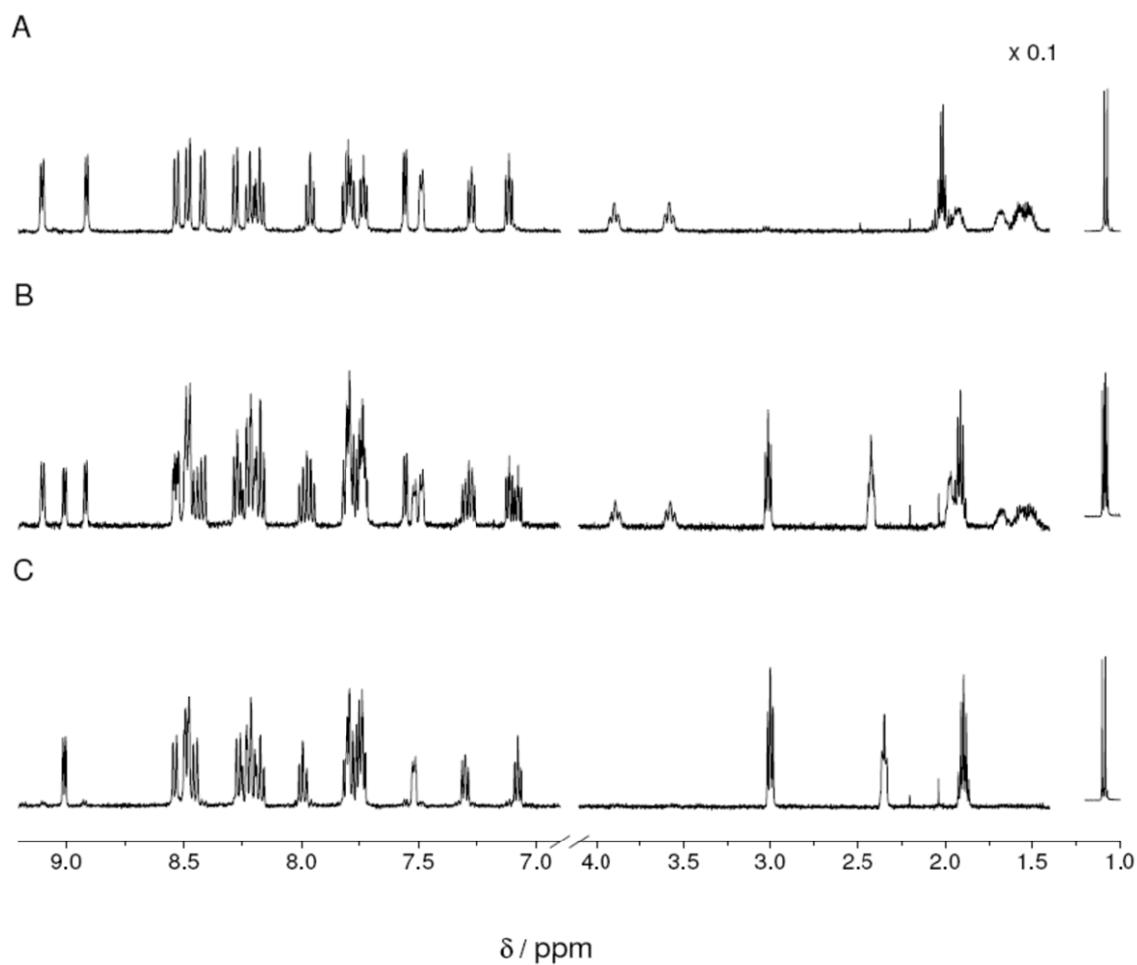
Fig. S1 ^1\text{H} -NMR spectrum of RuBiGABA-2 in \text{D}_2\text{O} before irradiation (A), after 40 s photolysis inside the NMR tube with 525 nm green light (B) and after 3 minutes irradiation, achieving full photolysis (C).
