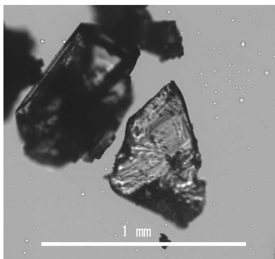
Figure S1. Crystals of VBT-4Pyr ( 3 ) before the irradiation.
