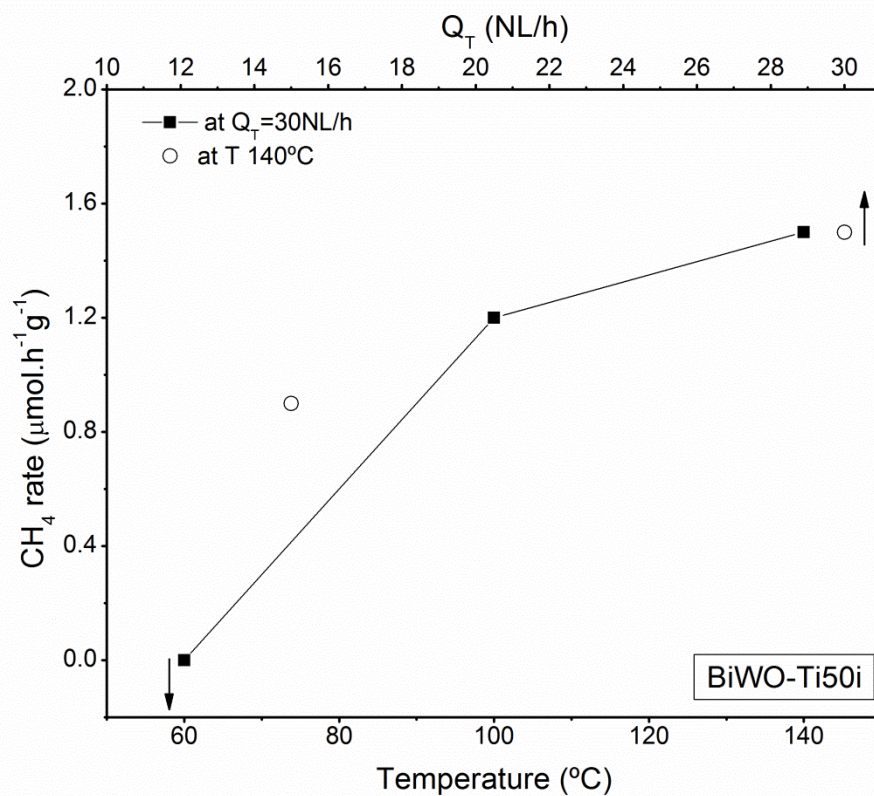
Figure S2. Preliminary tests with BiWO-Ti50i at different temperature (black) and total volume flow (white) conditions.
