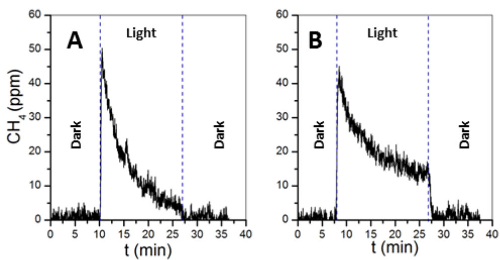
Figure S3. Evolution of the \text{CH}_4 signal during the photocatalytic tests with Pt-BiWO-Ti50i without (A) and with blue phosphors (B).
