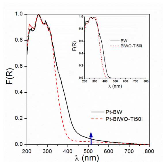
Figure S1. UV-vis diffuse reflectance spectra of the platinised photocatalysts. In the inset, the corresponding spectra of the non-platinised materials.
