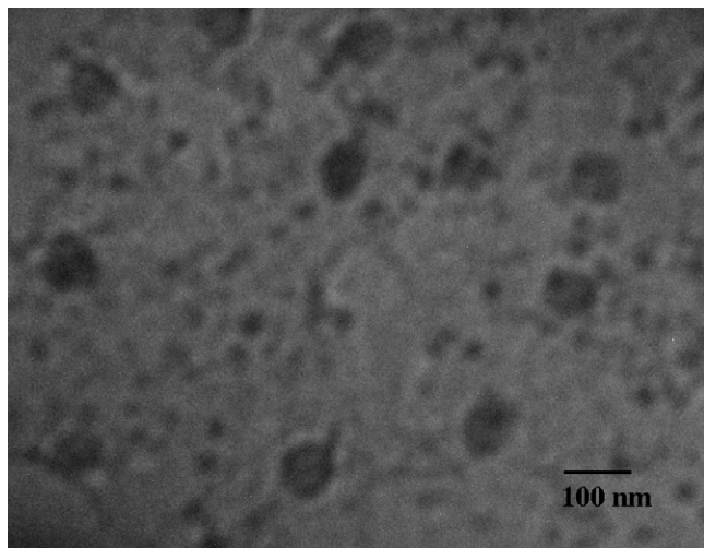
Figure S1. TEM image of PEO- b -PAMPS- b -PS micelles. The sample for the TEM measurement was prepared from the solution in which the concentration of polymer is 1 gL -1 . The micelles were stained by Fe 3+ ions. The large particles with a diameter of approximately 70 nm correspond to the micelles, while the small particles with a diameter of approximately 20 nm correspond to the flocks of Fe 3+ ions
