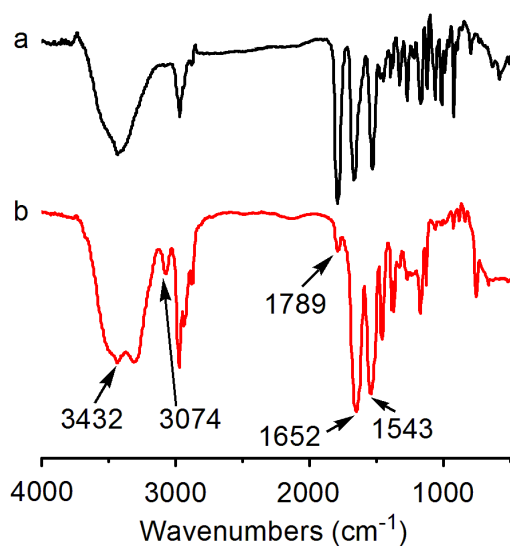
Fig. S1 FT-IR spectra of (a) poly(1 0.1 -co-4 0.9 ) and (b) poly(1 0.1 -co-4 0.9 )-based hydrogel (KBr tablet).
