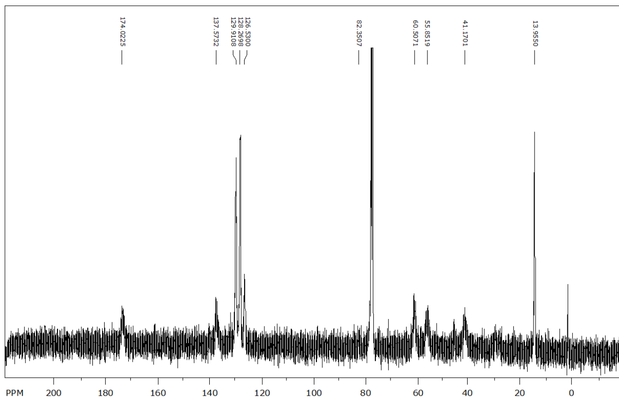
Fig. S4 ^{13}\text{C} NMR spectrum of polymer 10
