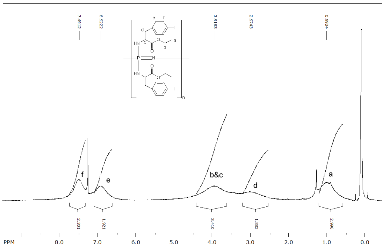
Fig. S5 1 H NMR spectrum of polymer 15
