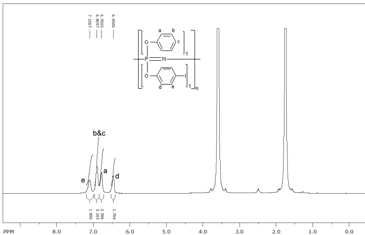
Fig. S1 1 H NMR spectrum of polymer 4
