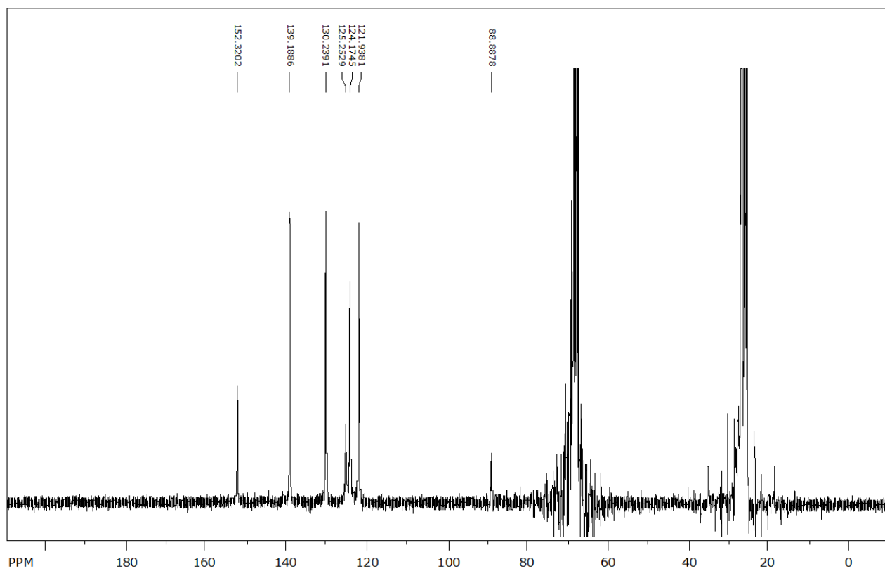
Fig. S2 ^{13}\text{C} NMR spectrum of polymer 4
