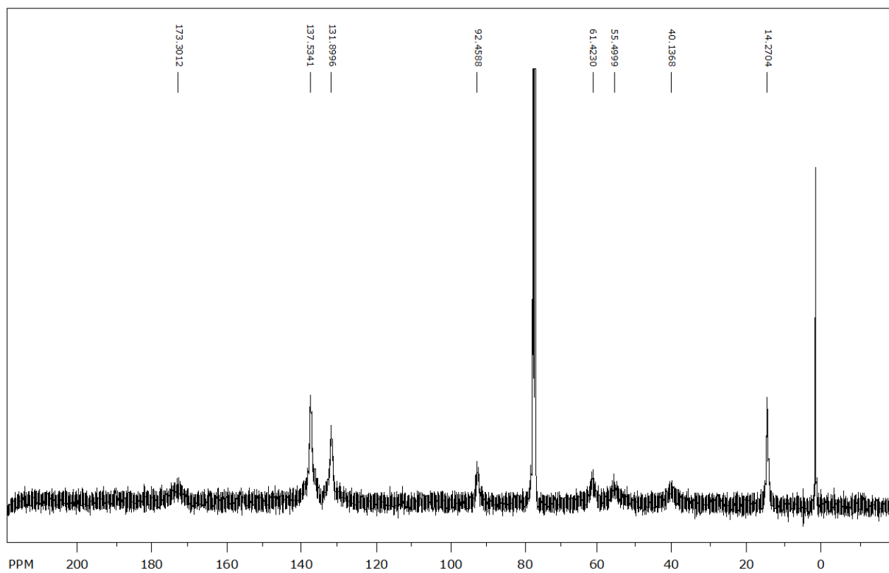
Fig. S6 ^{13}\text{C} NMR spectrum of polymer 15
