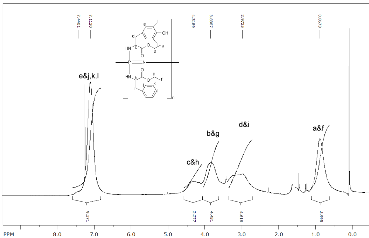
Fig. S3 1 H NMR spectrum of polymer 10
