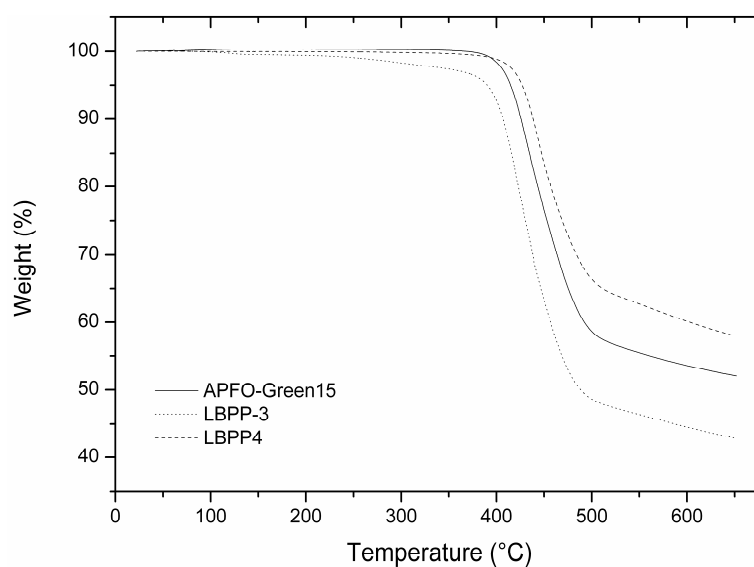
Fig. S1 Thermogravimetric analyses (TGA) of polymers in nitrogen atmosphere. Temperature is increased from room temperature to 650°C by 10°C/min.
