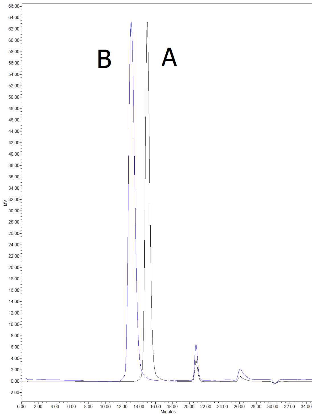
Fig.S1 SEC trace of allyl-(PEG-OH) 2 , A: M_n = 5.27 \times 10^3 , PDI = 1.08; B: M_n = 20.85 \times 10^3 , PDI = 1.09.
