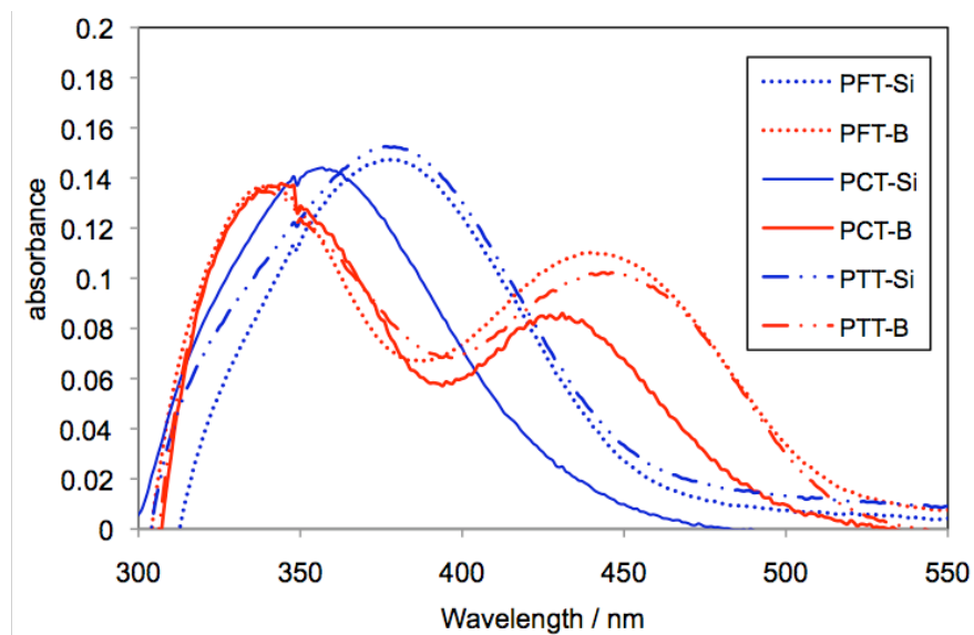
Figure S5. UV-vis absorption spectra for polymer thin films
