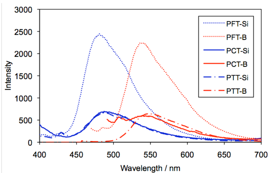
Figure S6. Fluorescence spectra for polymer thin films (excited at \lambda_{\text{max,abs}} )
