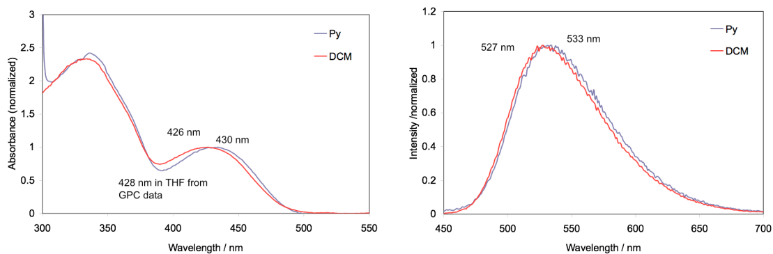
Figure S3. Absorption and Emission Spectra of PCT-B in Pyridine and DCM
