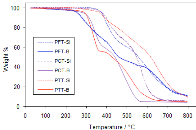
Figure S1. TGA traces for alternating copolymers (heating rate: 10 °C /min)
