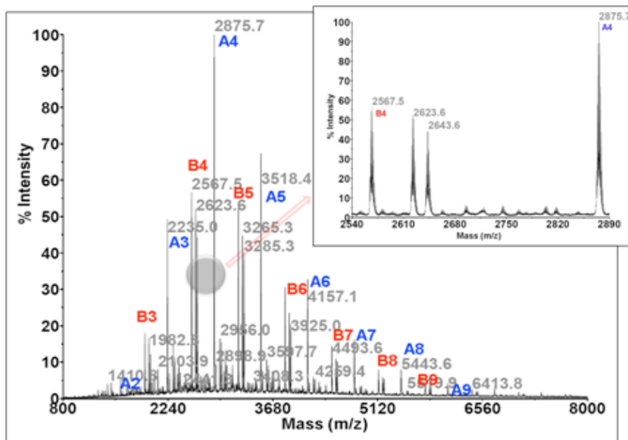
Figure S2. MALDI-TOF mass spectrum for PFT-Si acquired in (+) ion reflector mode; A_n = [Th_2Si_2-(Fl-Th_2Si_2)_n-H]^+ ; B_n = [H-(Fl-Th_2Si_2)_n-H]^+
