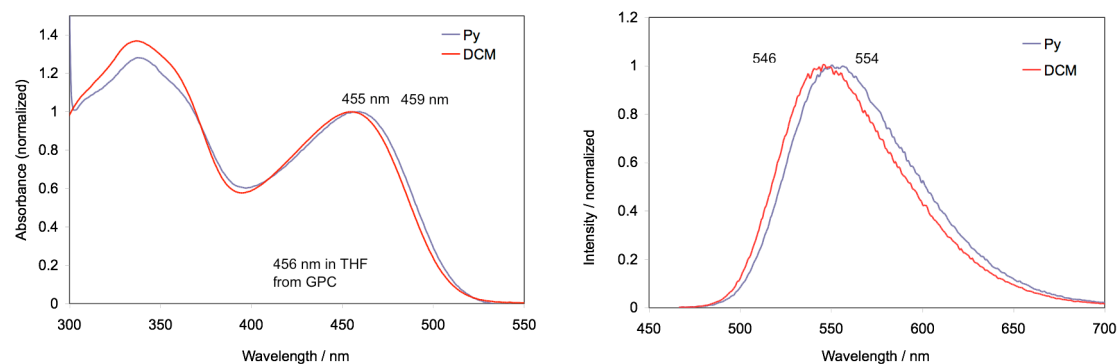
Figure S4. Absorption and Emission Spectra of PTT-B in Pyridine and DCM
