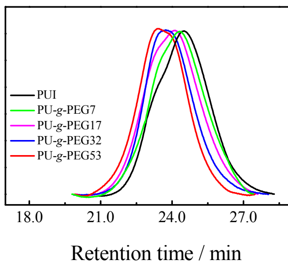
Figure S1. GPC curves of PUI and PU-g-PEG copolymers.
