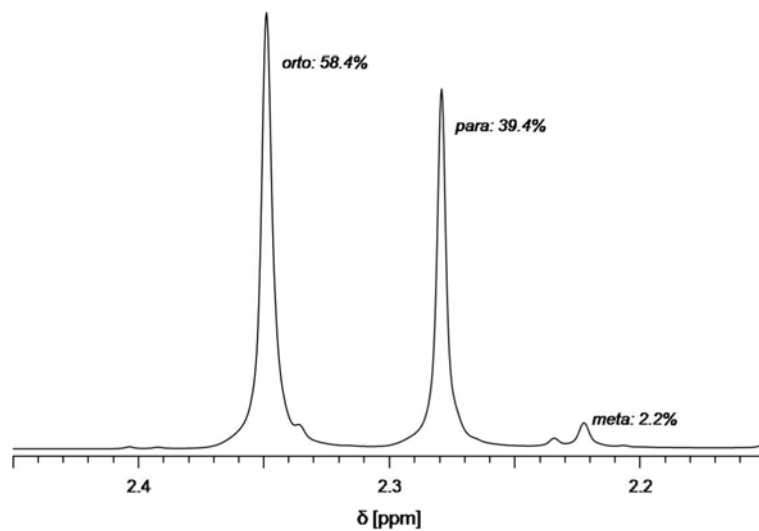
Figure 1S. 1 H-NMR spectrum (aliphatic region) of benzylmethylbenzene; the peaks correspond to -CH_3 group of the isomers.
