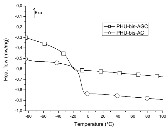
Figure S1: DSC thermograms of PHU-bis-AGC and PHU-bis-AC.
