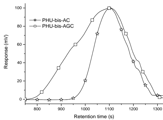
Figure S2: SEC chromatogram of PHU-bis-AGC and PHU-bis-AC in DMF solvent.
