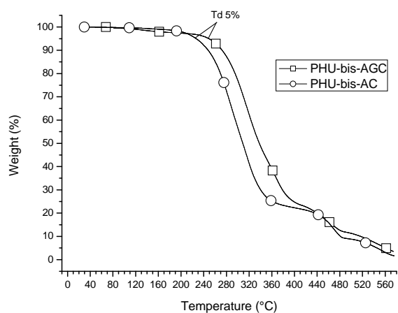
Figure S3: TGA thermogram of PHU-bis-AGC and PHU-bis-AC (heating rate 20°C/min).
