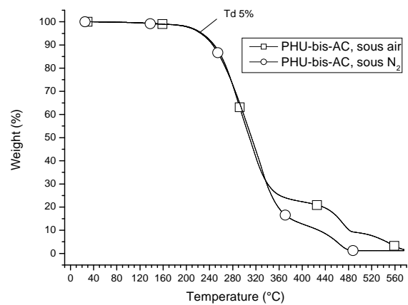
Figure S4: TGA thermogram of PHU-bis AC under air and under nitrogen (heating rate 20 °C/min).
