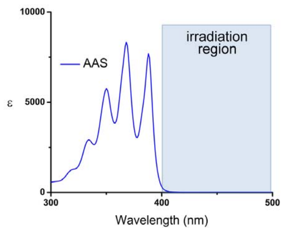
SF3. Absorption spectrum of AAS and irradiation wavelength for thiol-ene reaction
