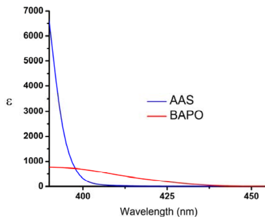
SF2. UV-vis spectra of AAS and BAPO
