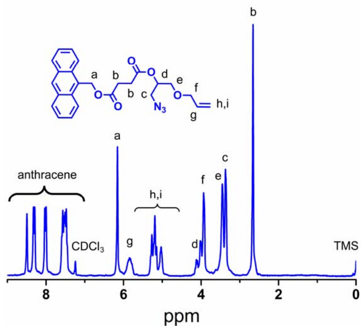
SF1. 1 H NMR spectrum of the core compound, AAS
