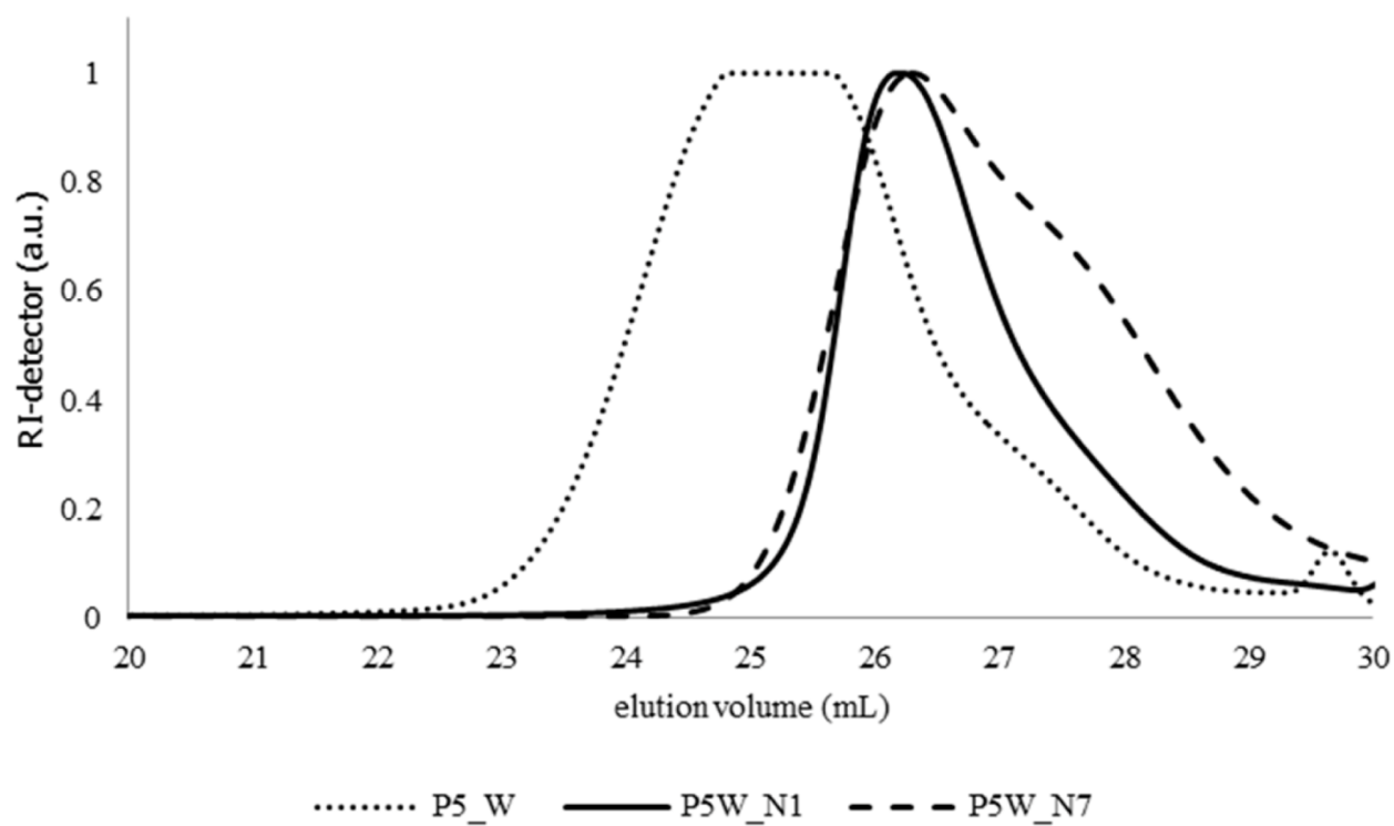
Figure S2 Gel permeation chromatograms of P5_W , P5W_N1 and P5W_N7 showing the shift in molecular weight after conversion with amines.
