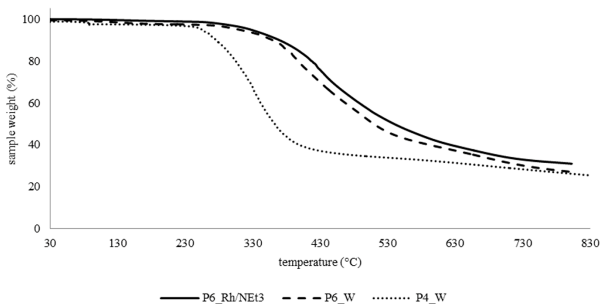
Figure S1 Thermogravimetric analysis of P6_Rh/NEt 3 , P6_W and P4_W.
