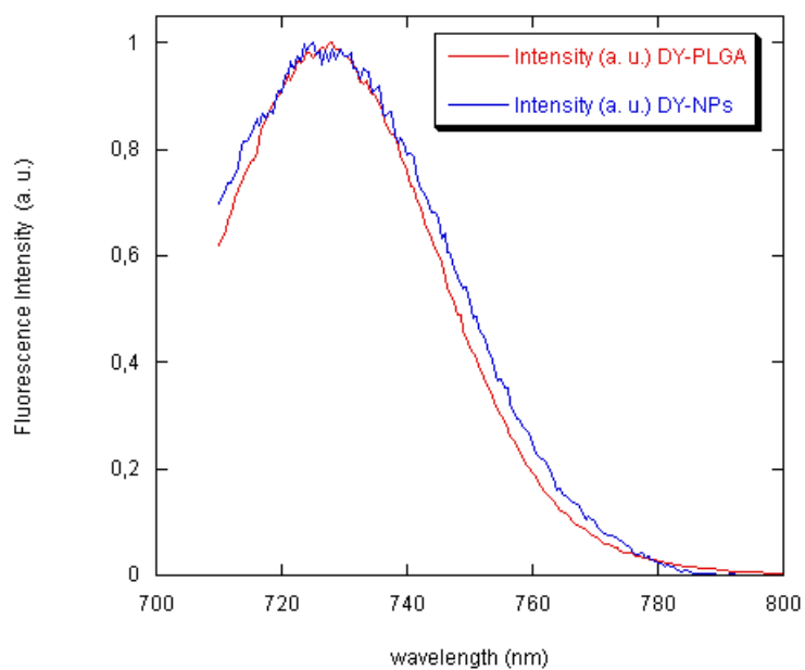
Figure S1: Fluorescent spectrum of DY-PLGA in DCM:ethanol 2:1 (v:v) (red) and DY-NPs in water (blue). The excitation wavelength was set at 700nm.
