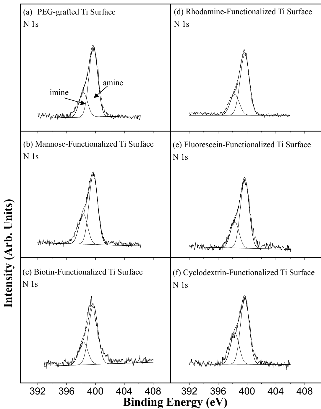
Figure S1: XPS N 1s core-level spectra of the six functionalized Ti surfaces
