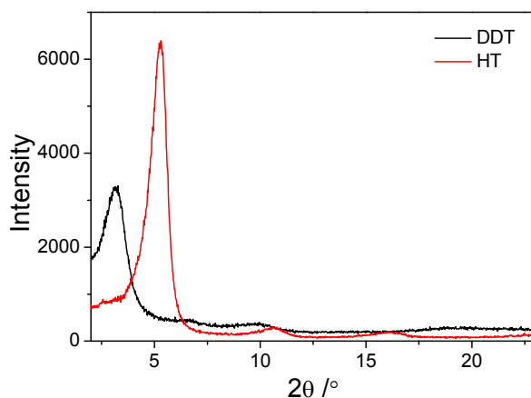
Fig. S1 XRD patterns of P3DDT and P3HT films.
