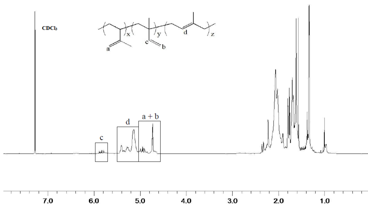
(a) The 1 H NMR spectra of PI oligomers.
