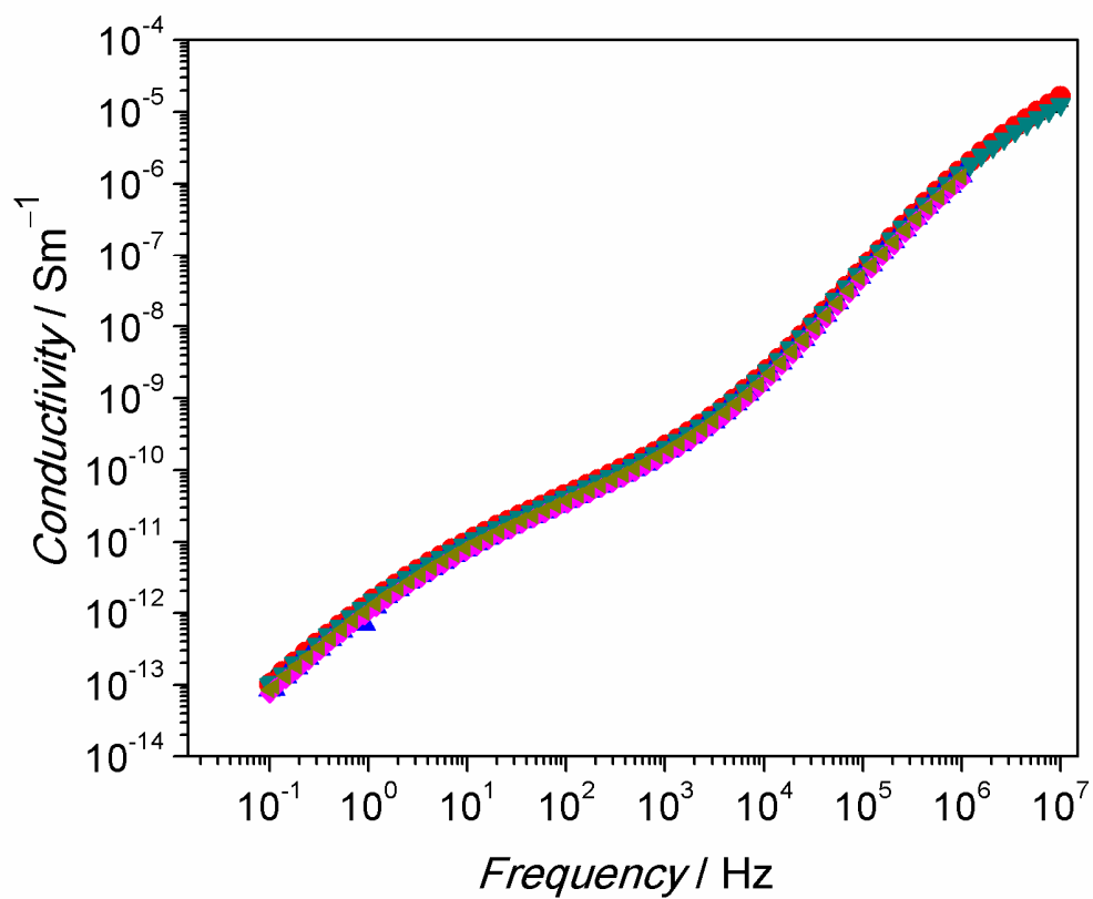
Figure S1: Conductivity as a function of frequency for PVDF containing 0.1 and 1.0 wt % of pristine SWCNTs as well as 0.05, 0.1 and 0.25 wt % of PVDF-functionalized SWCNTs.
