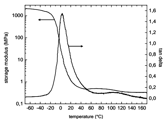
Figure 2. DMA trace of the SLSar-95 film.
