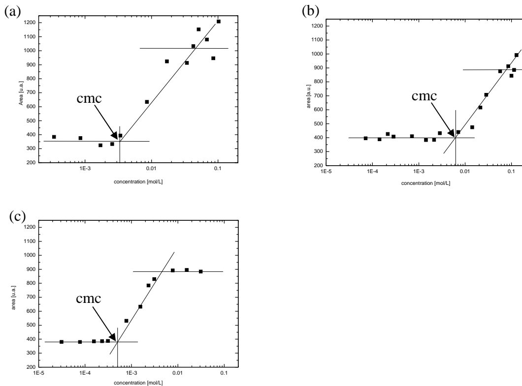
Figure 1. cmc determination of (a) SLSar, (b) SLGlu and (c) SMSar surfactants by fluorescence spectrophotometry using Nile red as the fluorescence probe. The arrows point the cmc values.
