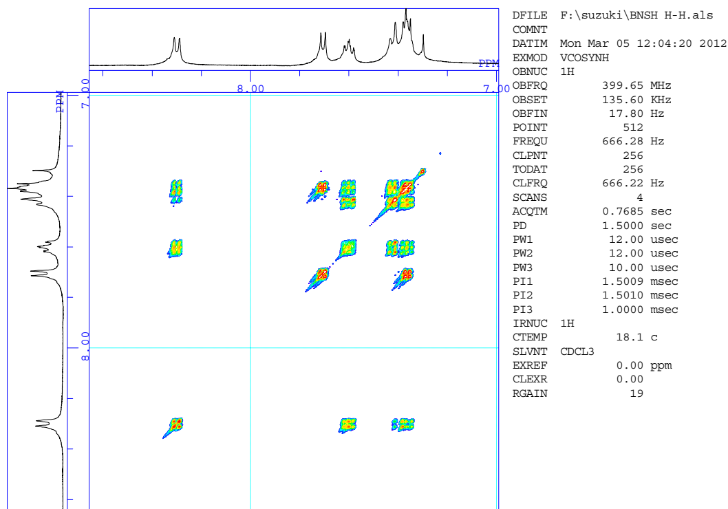
Figure S1. ^1\text{H} COSY spectrum of 3
