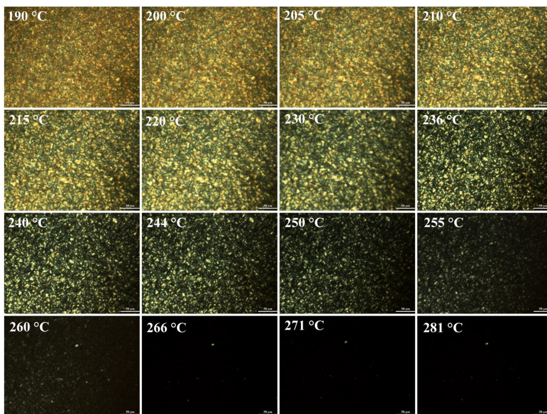
Fig. S1 Polarized optical microscope photographs of PDPBP5 obtained at different temperatures during heating (magnification 500 ×).
